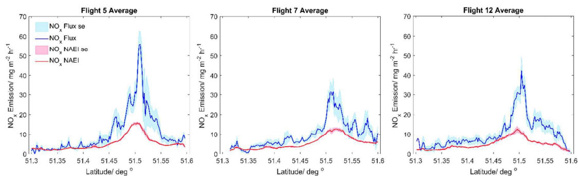
Figure 5. Average for Flight's 5, 7 and 12, measured \text{NO}_x flux plotted in blue with standard error as the shaded blue area. Calculated and scaled NAEI estimates of \text{NO}_x emission is plotted in red, with standard error as the shaded red area.
