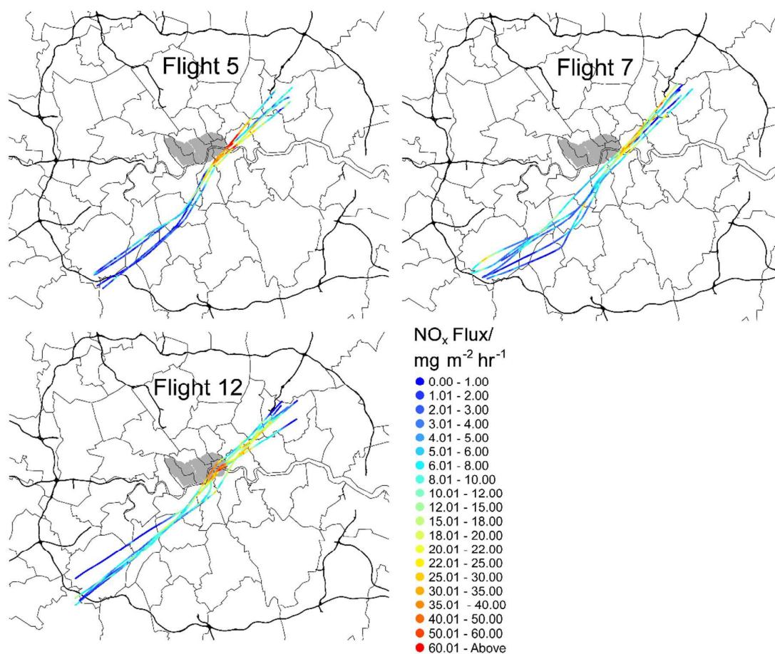
Figure 4. Tracks of all the flight legs for flights 5 (3 rd July 2013 morning), 7 (4 th July 2013 afternoon) and 12 (9 th July 2013 afternoon), mapped over Greater London, coloured to the measured NO x flux. The grey area represents London's Low Emission's Zone (LEZ).
