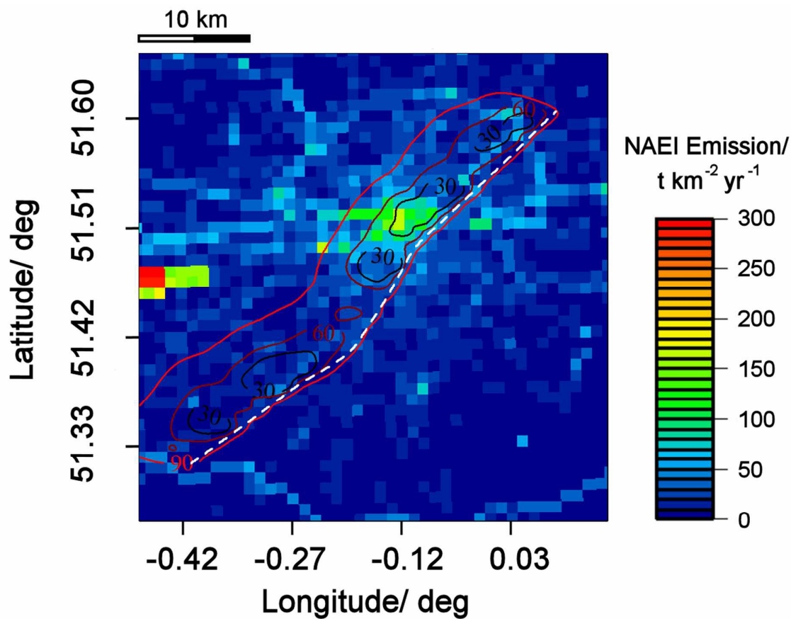
Figure 3. The contributing footprint area to a typical flight track, dependant on the prevailing wind direction and altitude of flight. The footprint is overlaid onto the NAEI at 1 km 2 grid resolution, coloured to annual NO x tonnage emission estimates.
