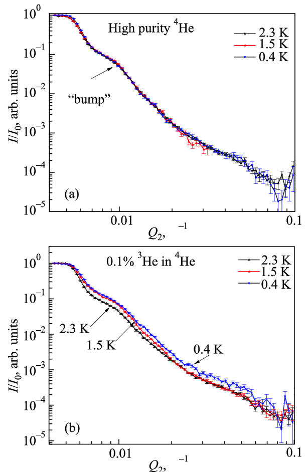
FIG. 1. Surface reflectivity curves collected at different temperatures: 2.3, 1.5, and 0.4 K from (a) isotopically purified helium; and (b) 0.1% 3 He/ 4 He mixture. We hypothesise that the seemingly anomalous “bump” indicated by the arrow in Fig. 1(a) is attributable to optical distortion caused by the liquid helium meniscus.
