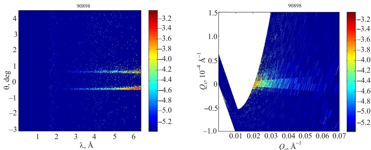
FIG. 3. Reflectivity signal maps shown on an area detector from a \text{D}_2\text{O} surface in a sample cell of 65 mm diameter. The neutron beam's horizontal dimension is significantly smaller than cell's diameter. There is no distortion due to the effect of the meniscus.
