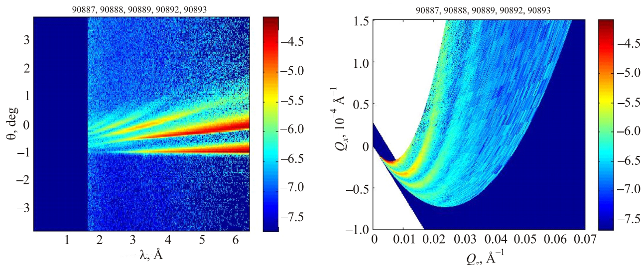
FIG. 4. Reflectivity signal maps shown on an area detector from a D 2 O surface in a sample cell of 35 mm diameter. The neutron beam's horizontal dimension is comparable with the cell diameter. We can see a periodic pattern in the reflection signal that can be explained by the interference of neutron waves on a curved surface.
