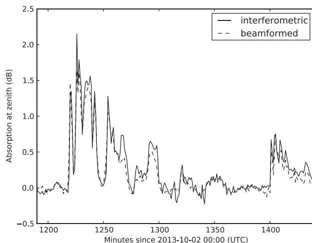
Figure 8. Detail showing the comparison between inteferometric and beamformed absorption measurements.
