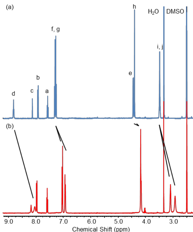
Figure 2: 1 H NMR spectra of (a) macrocycle 1 and (b) catenane 2 ( d 6 -DMSO, 400 MHz, 298 K). See Scheme 1 for atom labels.
