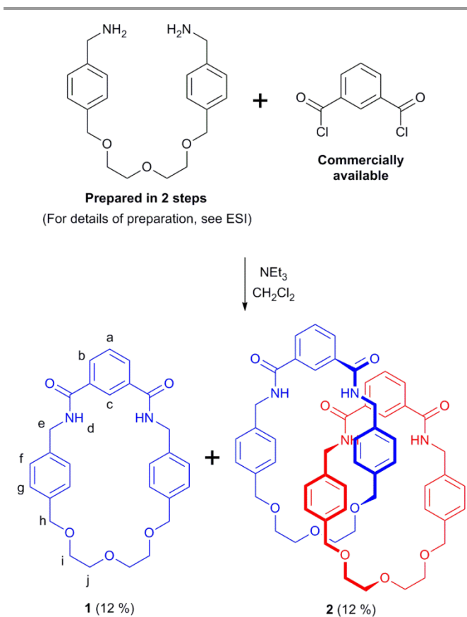
Scheme 1: Synthesis of Macrocycle 1 and Catenane 2 .
