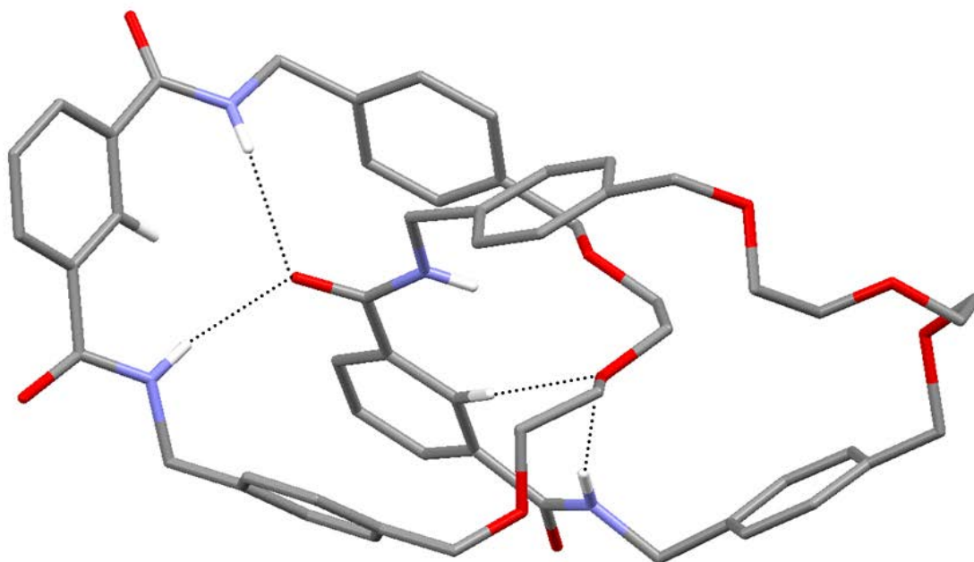
Figure 3: X-ray structure of catenane 2 . Hydrogen atoms (except N-Hs and isophthalamide internal C-Hs) and disorder in one of the rings are omitted for clarity.
