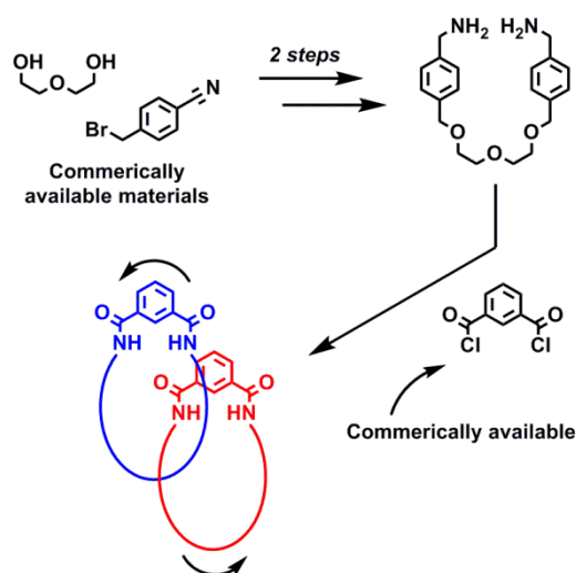
Figure 1: Schematic representation of the expedient three step synthesis of a dynamic isophthalamide [2]catenane.
