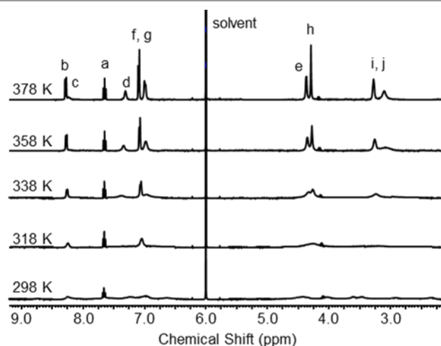
Figure 5: ^1\text{H} NMR spectra of catenane 2 recorded at T = 298\text{ K} to 378\text{ K} in \text{CD}_2\text{Cl}_4 (400 MHz). See Scheme 1 for atom labels.
