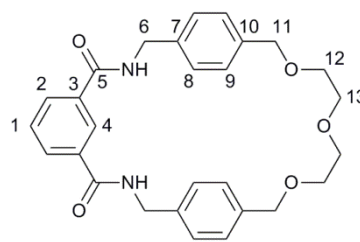
Figure 6: Carbon atom labels used in the assignment of the NMR data.
