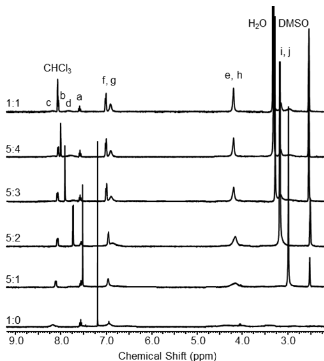
Figure 4: ^1\text{H} NMR spectra of catenane 2 recorded in \text{CDCl}_3:d_6\text{-DMSO} solvent mixtures (2.5 mM, 400 MHz, 298 K). See Scheme 1 for atom labels.
