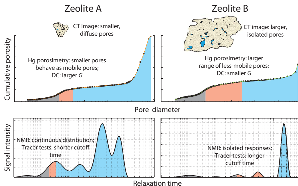
Figure 9. A simplified summary of the contrast in properties between zeolite A and zeolite B. Zeolite A has smaller and more continuous distribution of pores along with a larger G ; zeolite B has larger, isolated pores and a smaller G . The gray, red, and blue correspond to \theta_{dc} , \theta_{lm} , and \theta_m , respectively.
