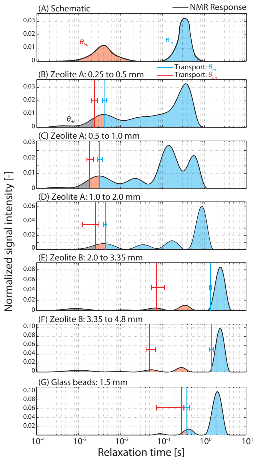
Figure 6. (a) The schematic shows an idealized NMR relaxation time distribution dominated by two distinct peaks that would correspond to \theta_m or \theta_{lm} , given by a single cutoff time. In the subsequent subplots (b–g), the NMR relaxation time is shown for each of the samples. The transport-estimated best fit \theta_m and \theta_{lm} are shown as blue and red lines, respectively, with associated error bars assuming a 1% error in the estimated \theta_m and \theta_{lm} .
