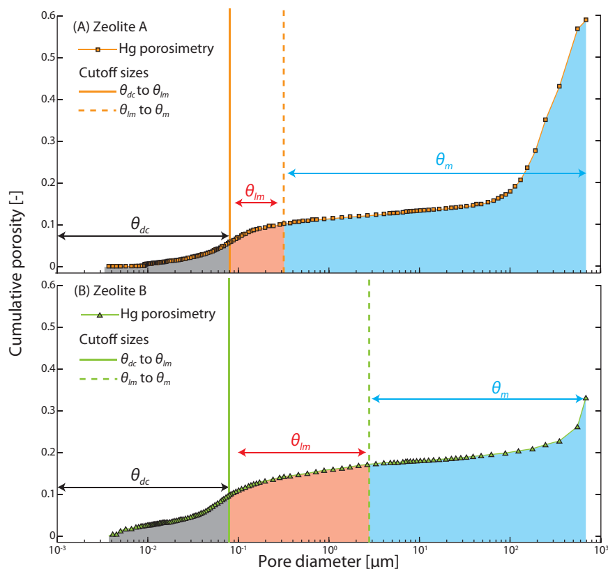
Figure 4. The results of the Hg porosimetry data show the cumulative porosity distribution from approximately 0.01 up to 700 \mu\text{m} for unsieved samples of zeolites A and B. The average difference between the transport and gravimetric porosity for the two zeolites, \theta_{dc} , is not active for transport. Cutoff values for \theta_m and \theta_{lm} are based on model calibration and assume that pores of a similar size have the same surrounding pore environment including degree of connectedness. Zeolite A has a wider range of pore-sizes that act as \theta_m .
