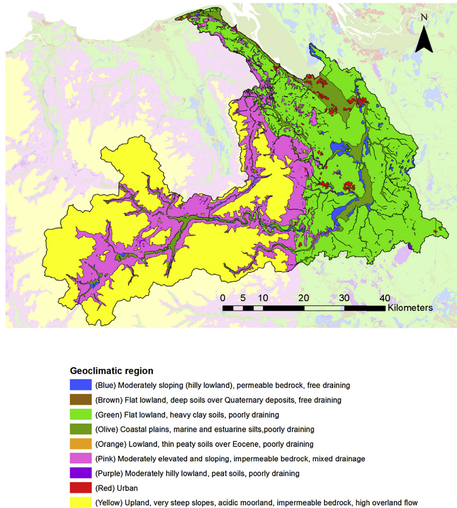
Fig. 5. Location and extent of the revised geoclimatic framework for the River Dee Water Framework Directive River Basin District (WFD RBD). The location of the River Dee catchment in the UK context is indicated in Fig. 3.
