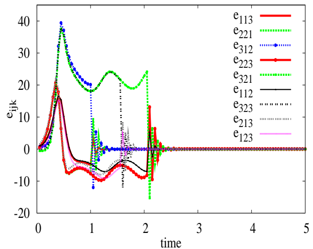
Fig. 4 Multi-switching synchronization error for switches 2,3 and 4. The controllers were activated at different times, switch 2 at time t \geq 1.5 , Switch 3 at t \geq 2 and Switch 4 at t \geq 1 . The error states are e_{112}, e_{223}, e_{321}, e_{123}, e_{213}, e_{323}, e_{113}, e_{221} , and e_{312} .
