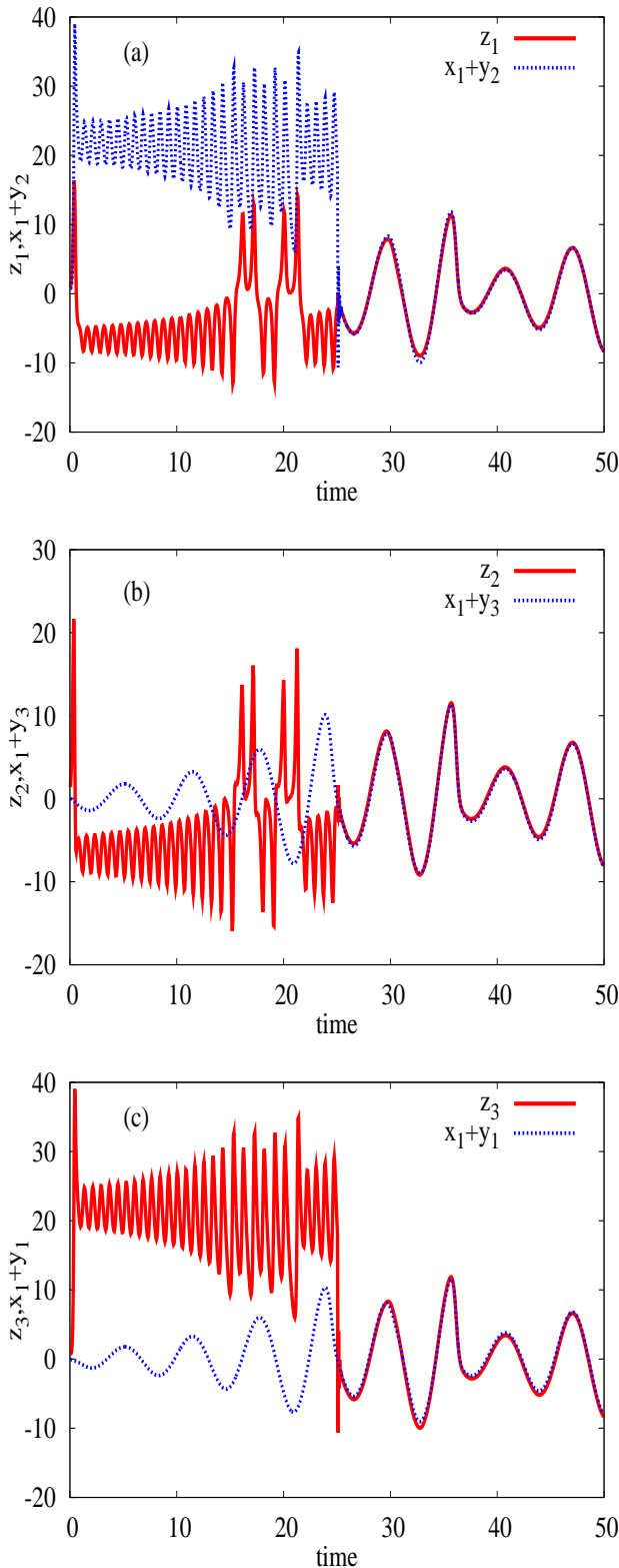
Fig. 2 Temporal behaviour of the synchronizing variables (a) z_1, (x_1 + y_2) , (b) z_2, (x_1 + y_3) , and (c) z_3, (x_1 + y_1) in the multi-switching compound synchronization state, with simultaneous activation of the controls at t \geq 25 . The parameters of the systems were chosen as a_1 = 0.2, b_1 = 0.2, c_1 = 5.7, a_2 = 0.4, b_2 = 0.175, a_3 = 10.0, b_3 = 23.0 and c_3 = 8.0/3 .
