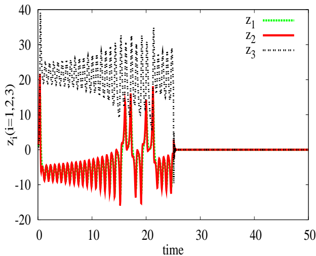
Fig. 3 Stabilization of state variables z_1, z_2, z_3 of the Lorenz system, when the controllers in Corollary 3 were activated at time, t \geq 25 .
