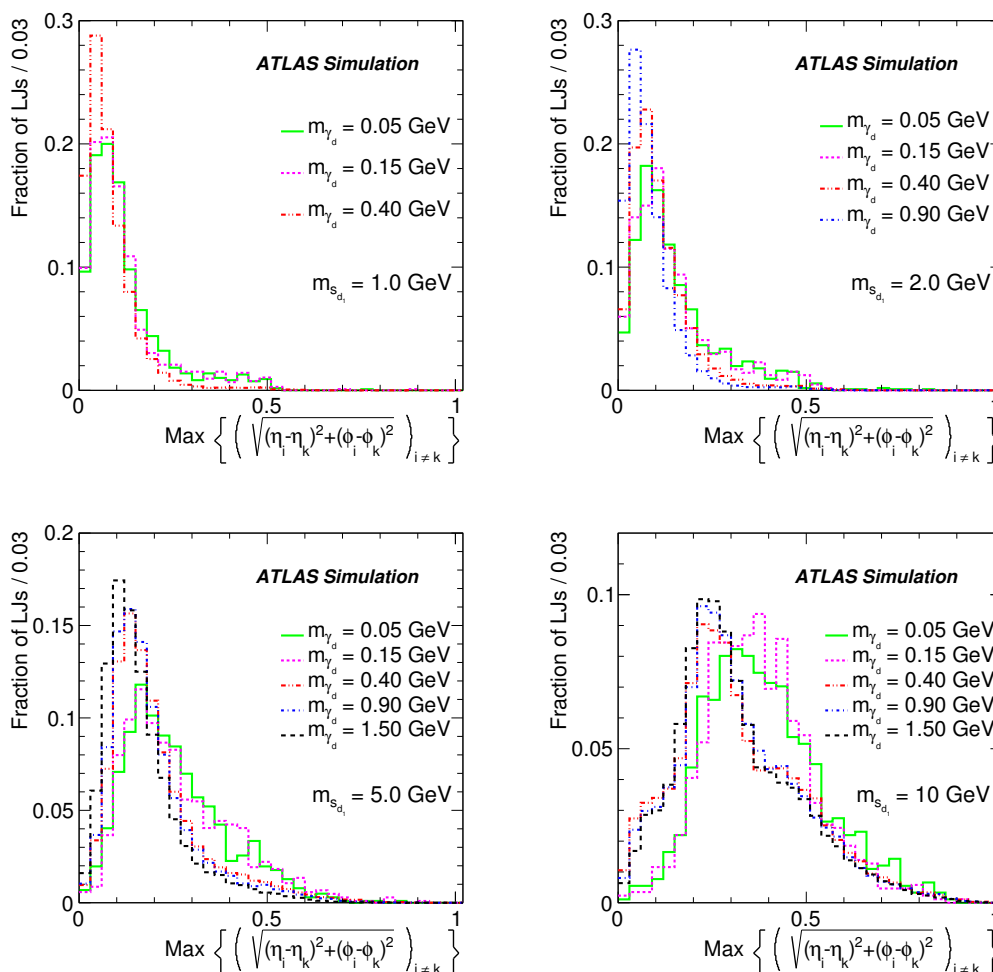
Figure 4. Maximum opening \sqrt{(\eta_i - \eta_k)^2 + (\phi_i - \phi_k)^2} between the reconstructed objects in the LJ (muons for TYPE0 LJ, muons and jets for the TYPE1 LJ) for the s_{d1} masses 1 GeV (top left), 2 GeV (top right), 5 GeV (bottom left) and 10 GeV (bottom right) and for all the kinematically allowed \gamma_d masses.
