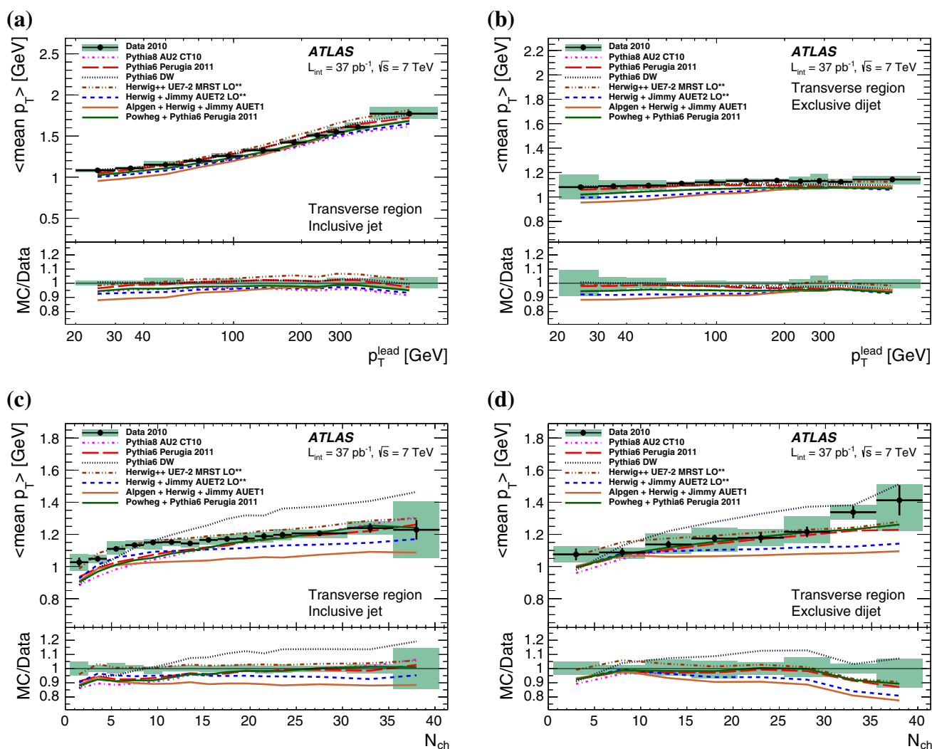
Fig. 6 Transverse region profiles of the mean p_T of charged particles for the inclusive (left) and exclusive dijet (right) selection against the leading-jet p_T (top row) and charged-particle multiplicity (bottom row). The jets are required to have p_T of at least 20 GeV and to be within
