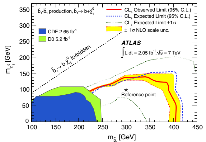
FIG. 2 (color online). Expected and observed exclusion limits, as well as \pm 1\sigma variation on the expected limit, in the \tilde{b}_1 - \tilde{\chi}_1^0 mass plane. The band around the observed limit delimited by the two dashed lines shows the effect of renormalization and factorization scale variation. The reference point indicated on the plane corresponds to the MSSM scenario with sbottom and neutralino masses of 300 GeV and 100 GeV, respectively. Results are compared to previous exclusion limits from Tevatron experiments. Results from LEP cover the region with sbottom mass below 100 GeV.
