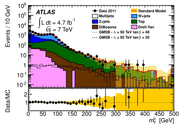
(a) m_T^\mu distribution for the τ + μ final state.
