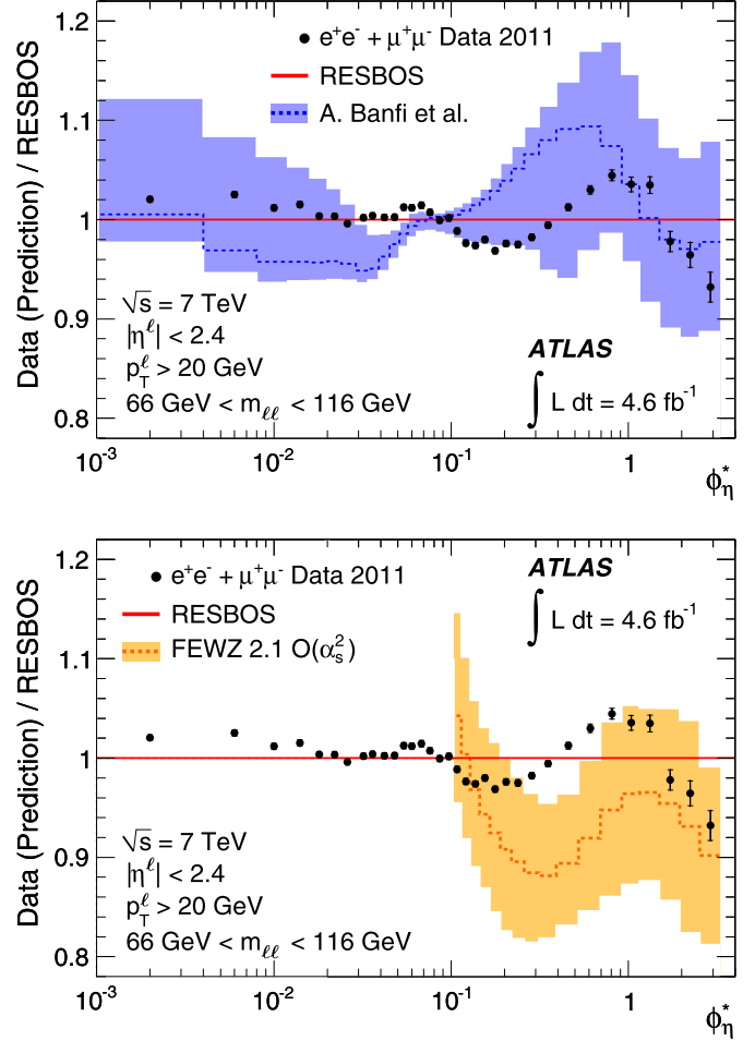
Fig. 2. The ratio of the combined normalised differential cross section 1/\sigma^{\text{fid}} \cdot d\sigma^{\text{fid}}/d\phi_{\eta}^* to ResBos predictions as a function of \phi_{\eta}^* . The inner and outer error bars on the data points represent the statistical and total uncertainties, respectively. The uncertainty due to QED FSR is included in the total uncertainties. The measurements are also compared to predictions, which are represented by a dashed line, from Ref. [22] and from FEWZ in the top and bottom panels, respectively. Uncertainties associated with these two calculations are represented by shaded bands. The prediction from FEWZ is only presented for \phi_{\eta}^* > 0.1 .
