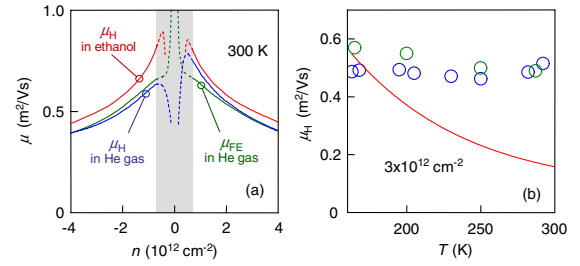
FIG. 3 (color online). Changes in \mu induced by ethanol. (a) Behavior of \mu_H and \mu_{FE} for the device shown in Fig. 2(b). Measurements of \mu are generally reliable only if \mu_H \approx \mu_{FE} . Inside the region around the NP, which is indicated by the gray area, apparent \mu_{FE} diverges because V_g passes through zero whereas apparent \mu_H goes to zero because \rho_{xy} passes through zero. The small difference between \mu_H and \mu_{FE} observed outside the gray area is attributed to a macroscopic inhomogeneity that leads to slightly different \rho_{xy} for different pairs of Hall contacts. (b) Varying dielectric screening in situ . \mu as a function of T for two devices immersed in ethanol (symbols). Dielectric constant \kappa of ethanol increases from \approx 25 to 55 with decreasing T . The solid curve is the T dependence expected in the case of dominant Coulomb scatterers [4,15]. The measurements are presented for n = 3 \times 10^{12} \text{ cm}^{-2} , but there is little difference for other assessable n > 1 \times 10^{12} \text{ cm}^{-2} . For the sample that shows a slight increase in \mu_H at lower T , we have found [by fitting the curves such as shown in Fig. 3(a)] that this increase is related to changes in \mu_L rather than \rho_S .
