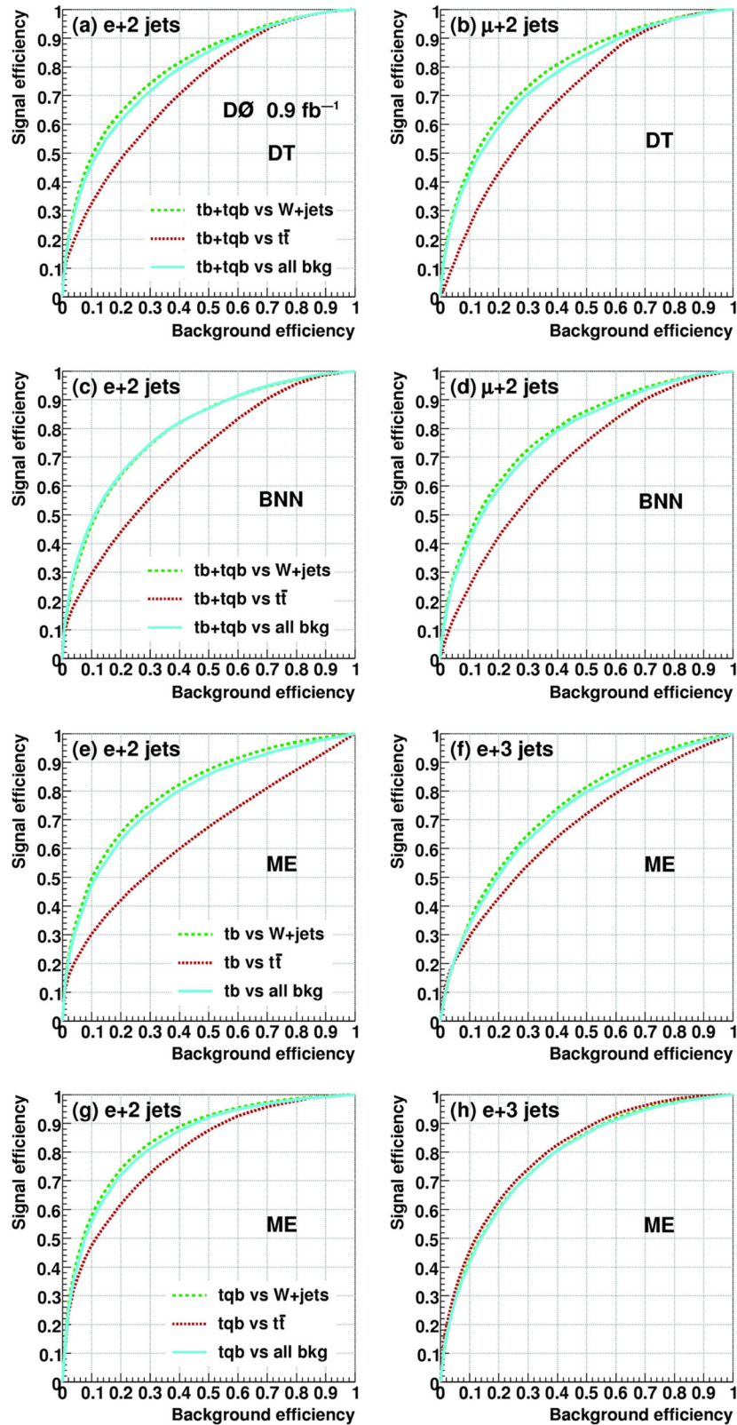
FIG. 14 (color online). For plots (a)–(d), DT and BNN tb + tqb signal efficiency versus background efficiency in the e + jets channel (left column) and \mu + jets channel (right column) for events with two jets of which one is b tagged. Plots (e)–(h) show the ME signal versus background efficiency for tb signal (third row) and tqb signal (fourth row), for b tagged e + jets events with two jets (left column) and three jets (right column). These curves are derived from the discriminants shown in Fig. 13.
