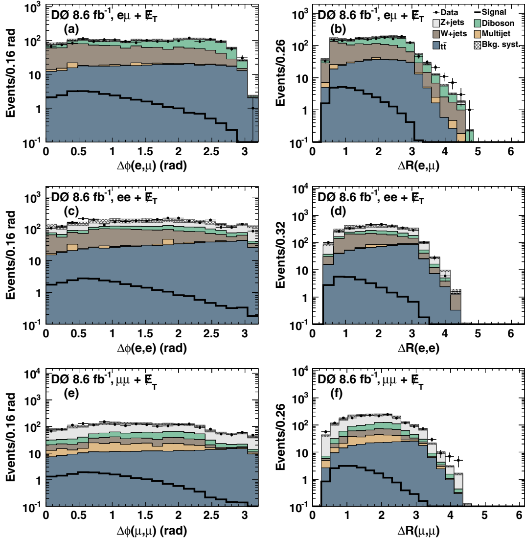
FIG. 6 (color online). The (left column) \Delta\phi(\ell_1, \ell_2) and (right column) \Delta R(\ell_1, \ell_2) for the e\mu (a),(b), ee (c),(d), and \mu\mu (e),(f) channel at the final selection stage. The signal distribution shown corresponds to a Higgs boson mass of 165 GeV. The hatched bands show the total systematic uncertainty on the background prediction.
