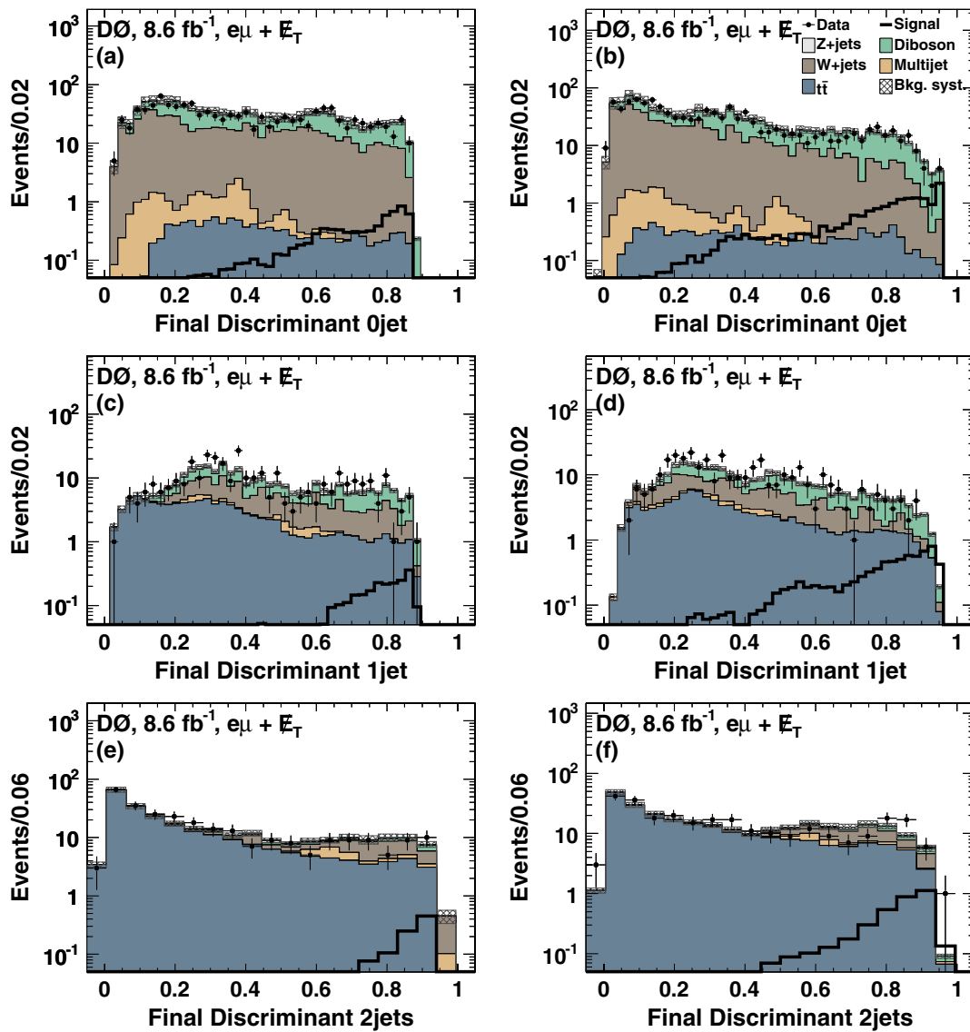
FIG. 10 (color online). Final BDT discriminant for the (top row) 0-jet, (middle row) 1-jet, and (bottom row) \geq 2 -jet bins for the e\mu final state for Higgs boson masses of 125 GeV [left (a),(c),(e)] and 165 GeV [right (b),(d),(f)]. The hatched bands show the total systematic uncertainty on the background prediction.
