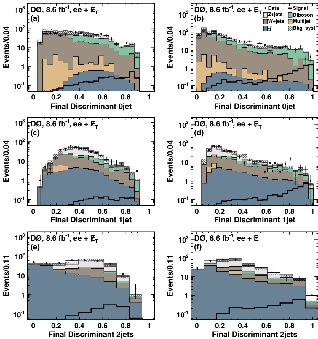
FIG. 11 (color online). Final BDT discriminant for the (top row) 0-jet, (middle row) 1-jet, and (bottom row) \geq 2 -jet bins for the ee final state for Higgs boson masses of 125 GeV [left (a),(c),(e)] and 165 GeV [right (b),(d),(f)]. The hatched bands show the total systematic uncertainty on the background prediction.
