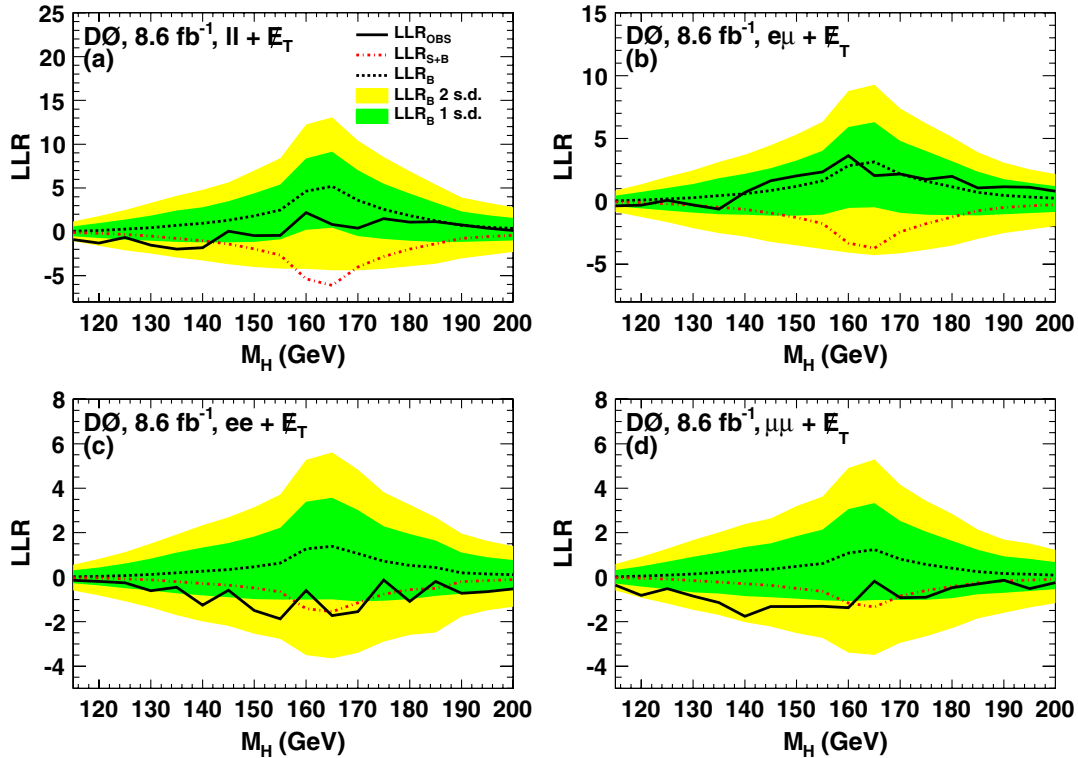
FIG. 16 (color online). The observed LLR (solid line) as a function of M_H using (a) all channels, (b) e\mu channel, (c) ee channel, (d) \mu\mu channel. Also shown are the expected LLR distributions for the background-only hypothesis (dashed line) and for the signal + background (dash-dotted line) hypothesis, with the dark grey and light grey bands indicating \pm 1 and \pm 2 s.d. fluctuations of the expected LLR distributions for the background-only hypothesis, respectively.
