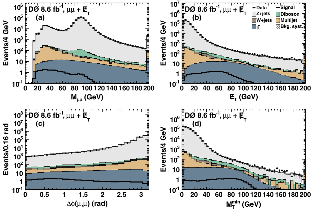
FIG. 3 (color online). (a) The dilepton mass, (b) \cancel{E}_T , (c) \Delta\phi between the leptons, and (d) minimum transverse mass for the \mu\mu channel at the preselection stage. The last bin also includes all events above the upper range of the histogram (a),(b),(d). The signal distribution shown corresponds to a Higgs boson mass of 165 GeV. The hatched bands show the total systematic uncertainty on the background prediction.
