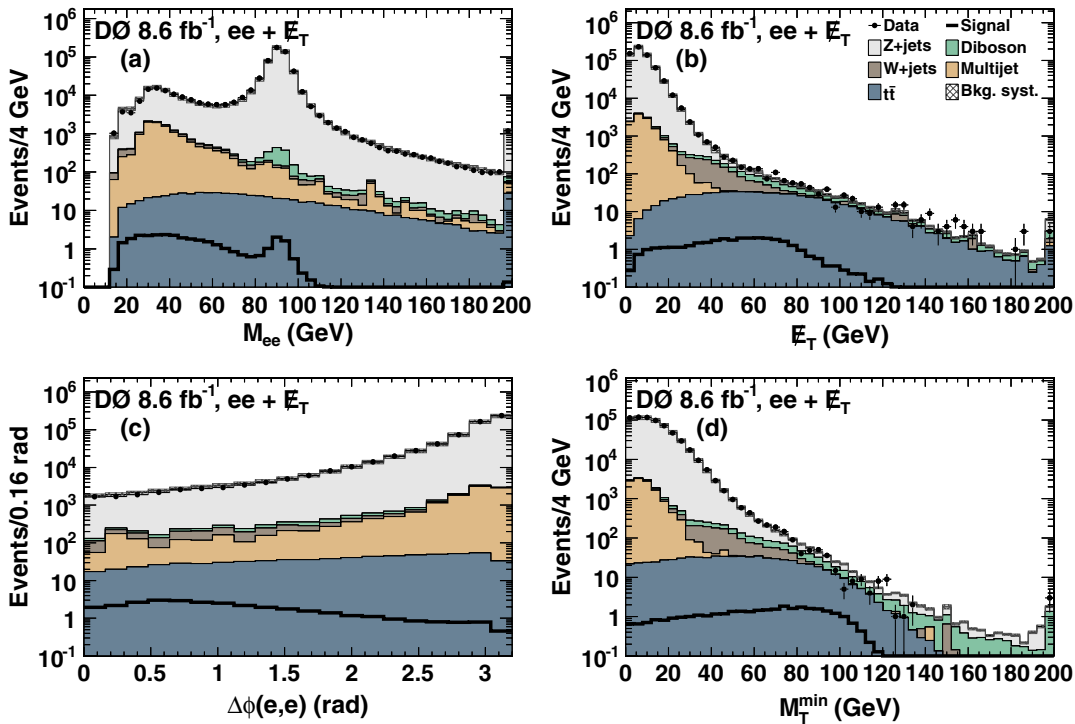
FIG. 2 (color online). (a) The dilepton mass, (b) \cancel{E}_T , (c) \Delta\phi between the leptons, and (d) minimum transverse mass for the ee channel at the preselection stage. The last bin also includes all events above the upper range of the histogram (a),(b),(d). The signal distribution shown corresponds to a Higgs boson mass of 165 GeV. The hatched bands show the total systematic uncertainty on the background prediction.
