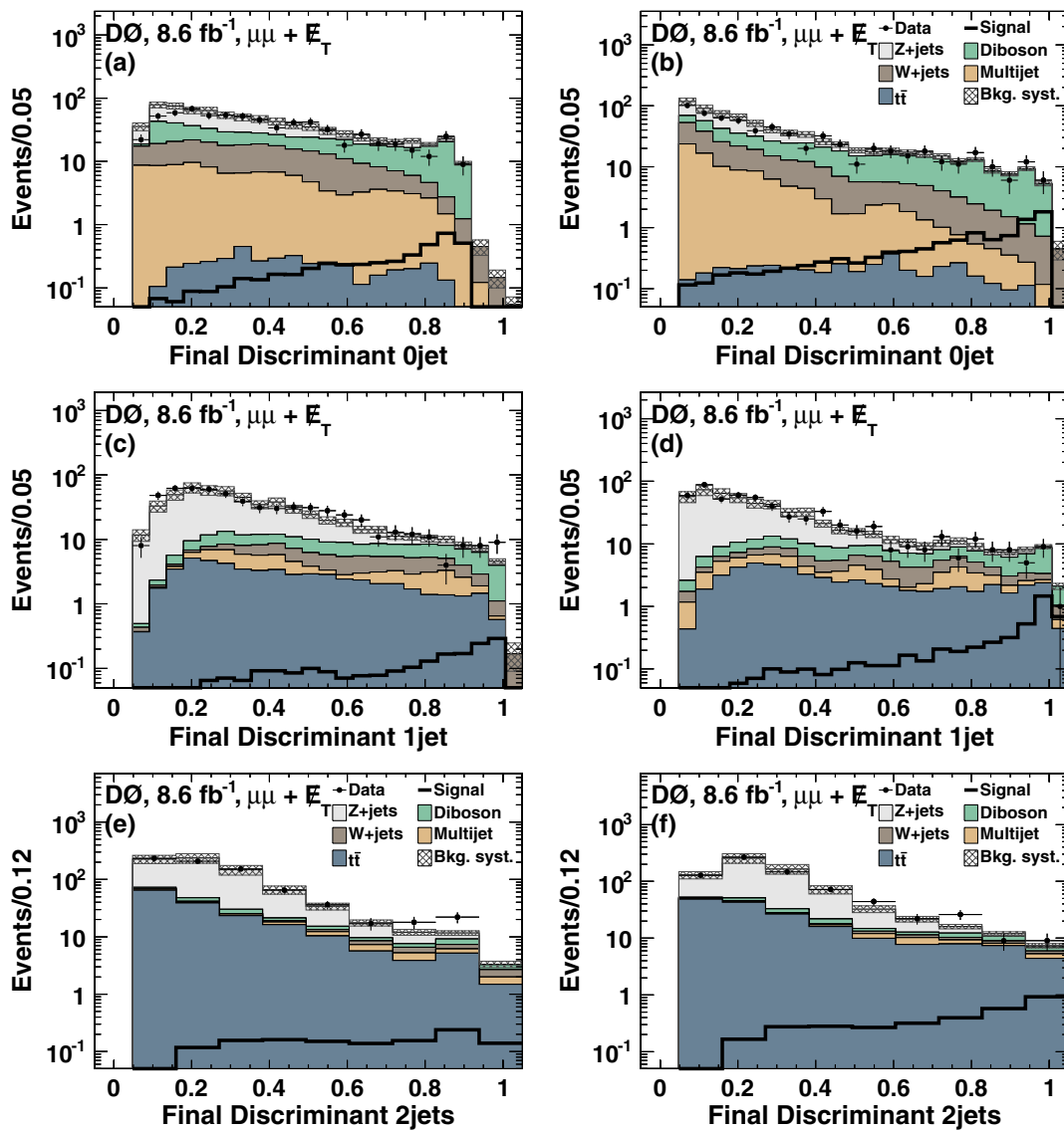
FIG. 12 (color online). Final BDT discriminant for the (top row) 0-jet, (middle row) 1-jet, and (bottom row) \geq 2 -jet bins for the \mu\mu final state for Higgs boson masses of 125 GeV [left (a),(c),(e)] and 165 GeV [right (b),(d),(f)]. The hatched bands show the total systematic uncertainty on the background prediction.
