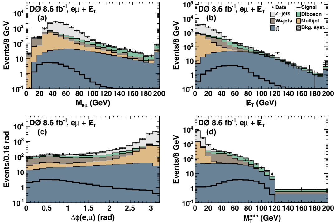
FIG. 1 (color online). (a) The dilepton invariant mass, (b) \cancel{E}_T , (c) \Delta\phi between the leptons, and (d) minimum transverse mass for the e\mu channel at the preselection stage. The last bin also includes all events above the upper range of the histogram (a),(b),(d). The signal distribution shown corresponds to a Higgs boson mass of 165 GeV. The hatched bands show the total systematic uncertainty on the background prediction.
