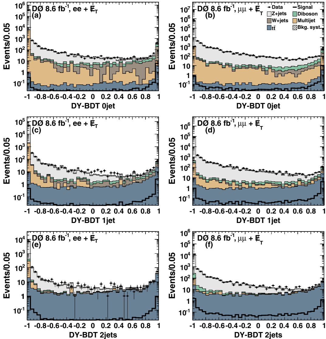
FIG. 5 (color online). DY-BDT discriminant for the 0-jet (top row), 1-jet (middle row), and \geq 2 -jet (bottom row) for the ee [left (a), (c),(e)] and \mu\mu [right (b),(d),(f)] final states. The discriminant shown is trained for a Higgs boson mass of 165 GeV. A final selection requirement is applied in the above distributions of 0.35, -0.6 , and -0.85 for the ee final state and 0.9, 0, and -0.7 for the \mu\mu final state, in the 0-jet, 1-jet, and \geq 2 -jet bins, respectively. The hatched bands show the total systematic uncertainty on the background prediction.
