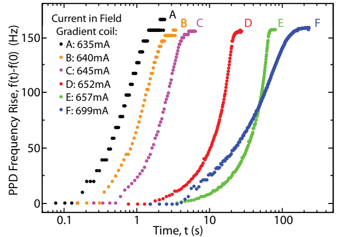
FIG. 4: The increase in the frequency of the PPD as a function of time during its free decay. The curves A,B,C,D,E and F correspond to different applied field gradients as indicated in figure 3.
