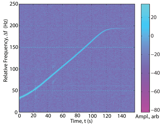
FIG. 2: A typical PPD signal. The plot shows a time dependent Fourier transform of the output signal from the mixer, giving the relative frequency \Delta f as a function of time. The color scale indicates the signal amplitude, see text.
