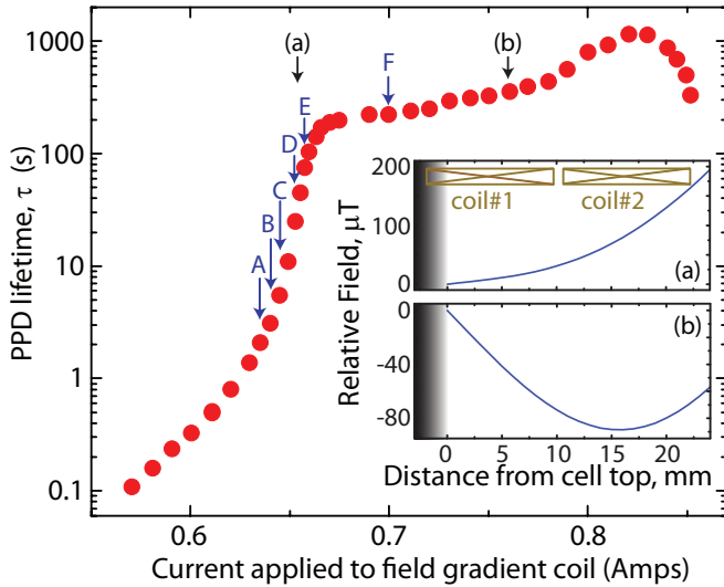
FIG. 3: The lifetime of the PPD as a function of the current applied to the field gradient coil. The measurements were taken using coil #1. The Inset shows calculated field profiles at two different applied field gradients, showing that the field minimum is well within the cell at (b) and moves out of the cell as the gradient falls below the value indicated at (a). The labels A,B,C,D,E and F indicate the applied field gradients at which further measurements are presented in figures 4-6.
