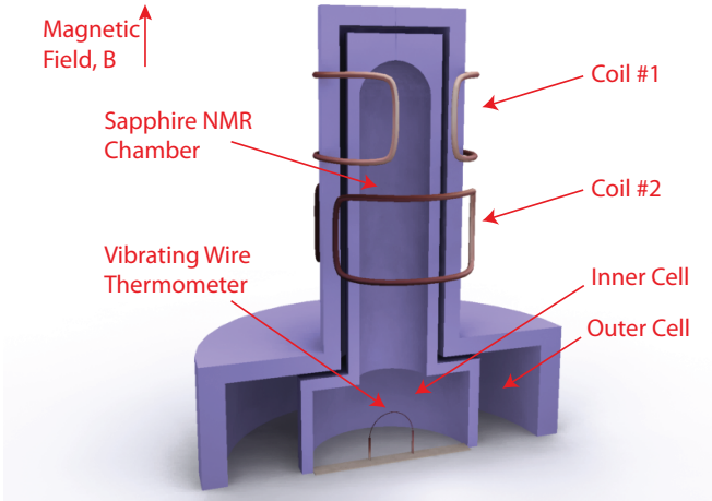
FIG. 1: A schematic of the double walled experimental cell. Two saddle coils are used to excite and detect the PPD in different locations. The NMR chamber is formed by a cylindrical sapphire tube extending up from the inner cell.
