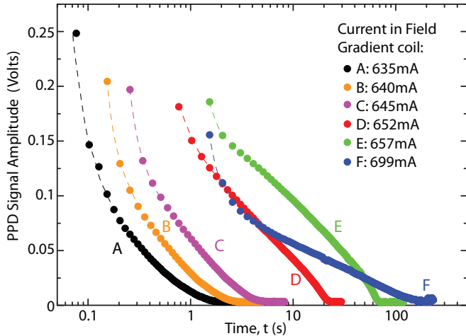
FIG. 5: The amplitude of the PPD signal, measured directly from the voltage data, as a function of time during its decay. The data show the same PPDs used in figure 4.
