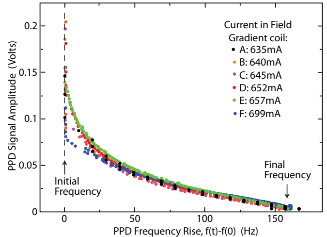
FIG. 6: The amplitude of the PPD signal as a function of its rise in frequency, f(t) - f(0) . The data show the same PPDs used in figures 4 and 5.
