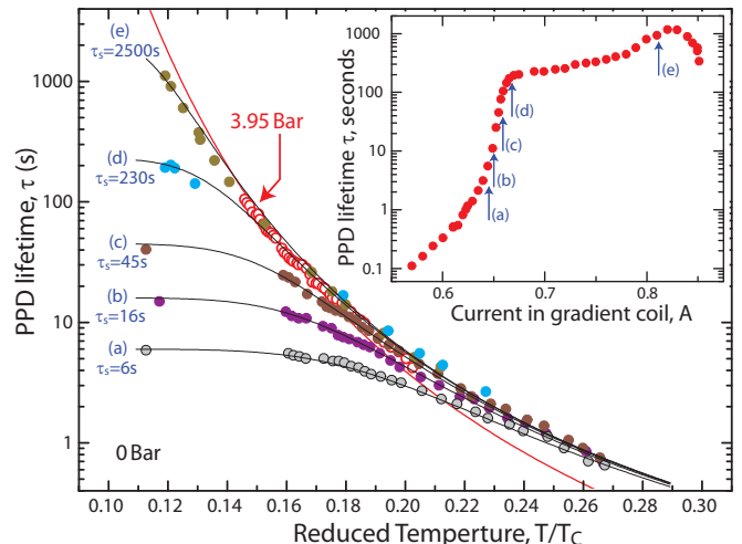
FIG. 7: The lifetime of the PPD as a function of reduced temperature, T/T_C , for various applied field gradients. Data at 0 bar pressure are shown for 5 different applied field gradients, labelled (a) to (e) as indicated in the inset. The inset shows the lifetime at the lowest temperatures as a function of the current applied to the gradient coil. Open red circles show data taken at 3.95 bar pressure for PPD held well away from the end of the cell. Black lines give fits to the data using equations 24 and 25 with different values for the surface relaxation lifetime \tau_s as indicated. The red line corresponds to 3T_{DF} , where T_{DF} is given by eq. (50), See text.
