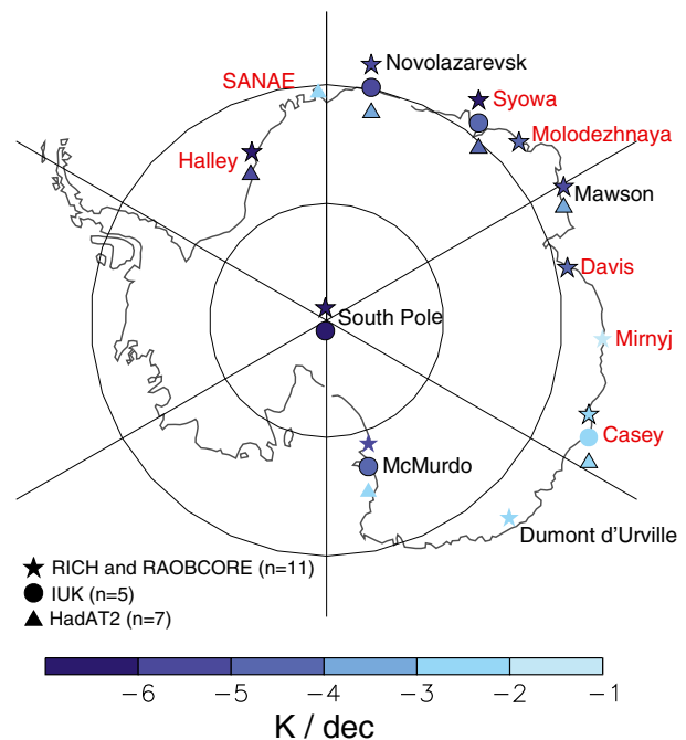
Figure 1. Locations of the radiosonde stations from the different data sets used in this study, colored by their November 100 hPa trend over 1969 to 1998 (K/dec). Symbols with black outlines indicate that the trend is significant at the 5% level. Stations in red are those analyzed by Thompson and Solomon [2002].
