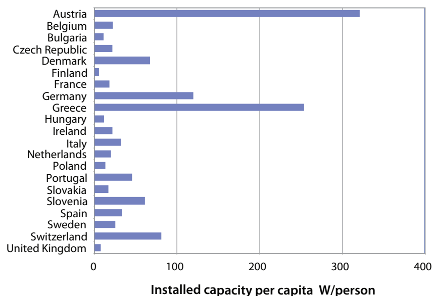
Figure 15: Installed capacity solar thermal 2010
