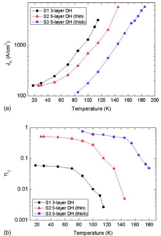
FIG. 3. (Color online) (a) Dependence of threshold current density ( J_{\text{th}} ) on temperature ( T ) and (b) the dependence of differential quantum efficiency on temperature for the samples S1, S2, and S3.
