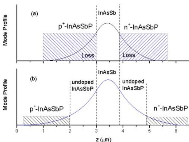
FIG. 1. (Color online) InAs 0.61 Sb 0.13 P 0.26 /InAs 0.96 Sb 0.04 fundamental TE optical mode profile along the growth axis for (a) conventional three-layer DH laser and (b) five-layer DH structure with additional undoped InAs 0.61 Sb 0.13 P 0.26 layers inserted between the InAsSb active region and the highly doped InAsSbP cladding layers.
