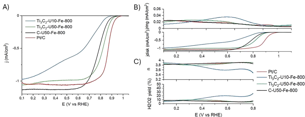
Fig. 4 (A) Linear sweep voltammogram at 5 \text{ mV s}^{-1} of the different samples in 0.1 \text{ M} aerated KOH electrolyte (corrected) at 1600 \text{ rpm} . (B) Rotating ring disk electrode measurements of the different \text{Ti}_3\text{C}_2\text{-U}_x\text{-Fe-800} samples, C-U50-Fe-800, and Pt/C in 0.1 \text{ M} aerated KOH electrolyte (corrected) at 1600 \text{ rpm} and scan rate of 5 \text{ mV s}^{-1} : j_{\text{disk}} (bottom) and j_{\text{ring}} (top), (C) calculated \text{H}_2\text{O}_2 yield (bottom) and electron-transfer number n (top) for \text{Ti}_3\text{C}_2\text{-U}_x\text{-Fe-800} samples, C-U50-Fe-800, and Pt/C.
