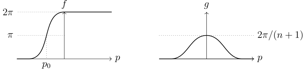
Figure 4: The functions f and g used in the definitions of the symplectomorphisms \rho and \delta in §3.3.
