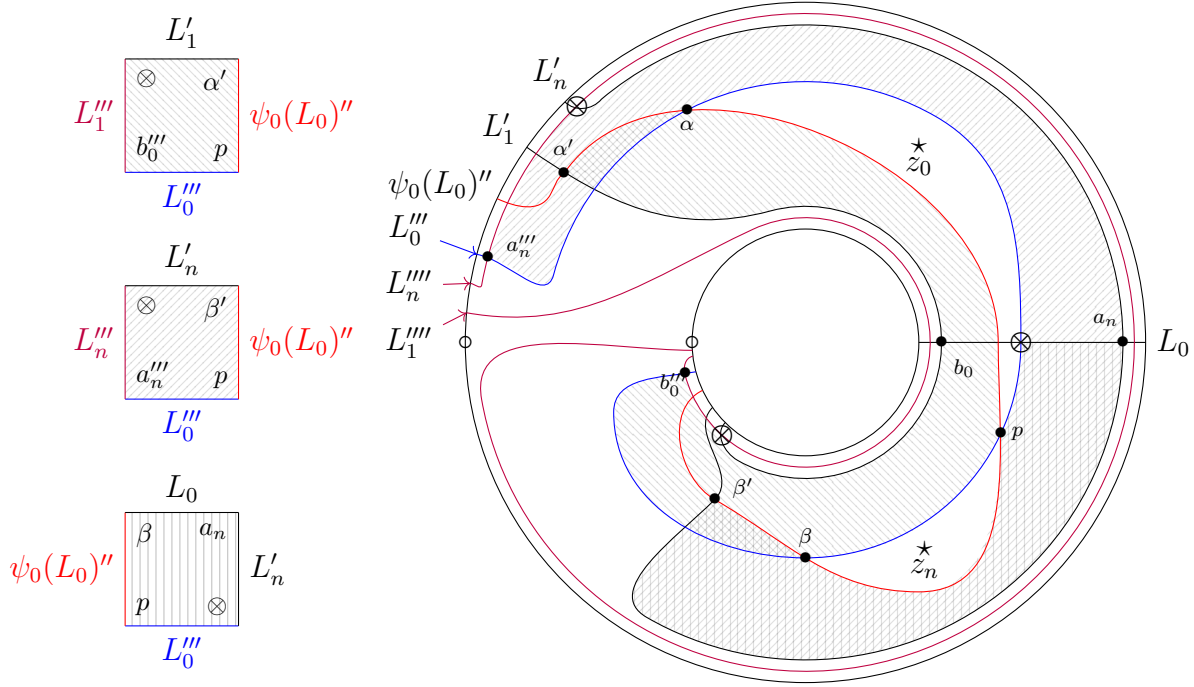
Figure 6: The choices of partially wrapped Hamiltonian perturbations for the computations in §3.8. The intersection points marked \otimes denote the identity elements of the corresponding Floer complex. We show the three holomorphic quadrilaterals which contribute to \mu_3(\alpha', p, b_0''') , \mu_3(\beta', p, a_n''') and \mu_3(a_n, \beta', p) (all other products vanish with these choices); the quadrilaterals are distinguished by the direction of their hatching.
