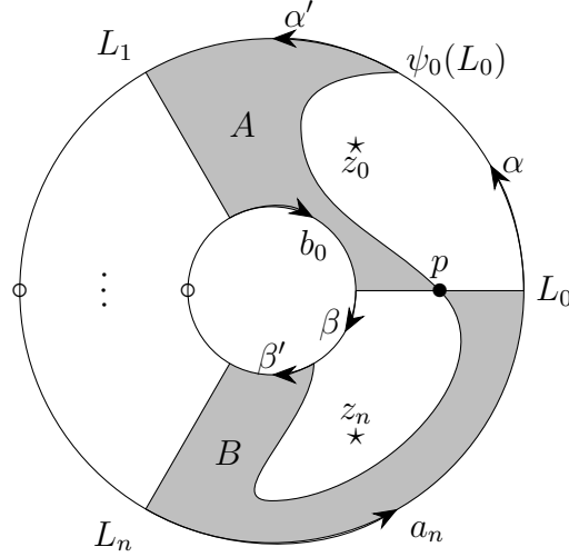
Figure 5: The half-twisted arc \psi_0(L_0) , perturbed slightly along the Reeb flow to separate it from L_0 . We have added two stops on the boundary for convenience; these are labelled \circ . We have also labelled the Reeb orbits connecting the Lagrangian arcs. Note that a_0 = \alpha'\alpha and b_n = \beta'\beta . The point p (marked with a \bullet ) is an intersection point of L_0 with \psi_0(L_0) . Two important polygonal regions A and B are shaded.
