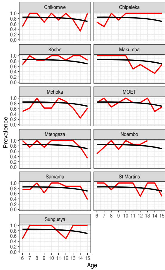
Figure S15: Prior Schistosoma infection prevalence of \alpha = 0.10 for SAC age 6. Single- \beta with no space effect model optimisation prevalence prediction (black line) and observed prevalence (red line) against age of SAC carried out for each species a) Biomphalaria sp. b) Bulinus spp.
