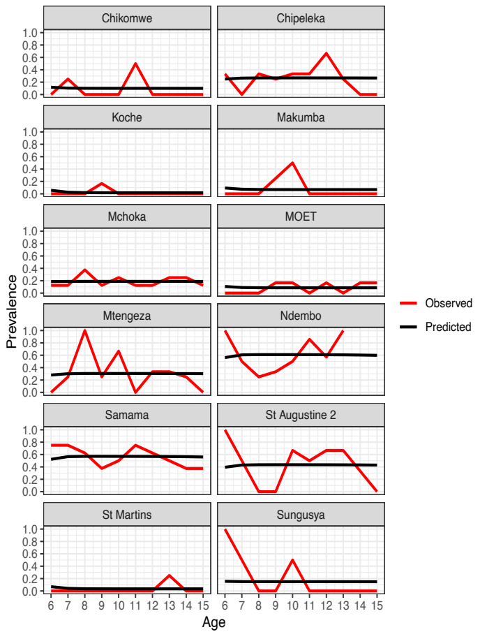
Figure S16: Prior Schistosoma infection prevalence of \alpha = 0.20 for SAC age 6. Multi- \beta_s with space effect model optimisation prevalence prediction (black line) and observed prevalence (red line) against age of SAC carried out for each species a) Biomphalaria sp. b) Bulinus spp.
