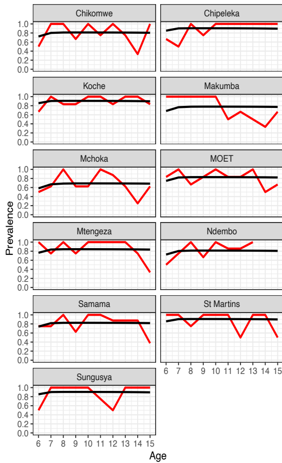
Figure S16: Prior Schistosoma infection prevalence of \alpha = 0.20 for SAC age 6. Multi- \beta_s with space effect model optimisation prevalence prediction (black line) and observed prevalence (red line) against age of SAC carried out for each species a) Biomphalaria sp. b) Bulinus spp.
