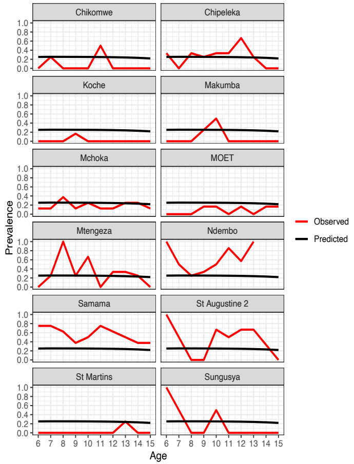
Figure S15: Prior Schistosoma infection prevalence of \alpha = 0.10 for SAC age 6. Single- \beta with no space effect model optimisation prevalence prediction (black line) and observed prevalence (red line) against age of SAC carried out for each species a) Biomphalaria sp. b) Bulinus spp.
