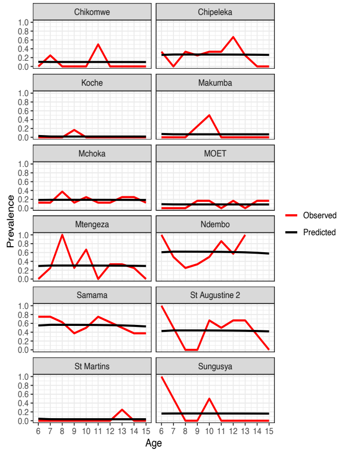
Figure S18: Prior Schistosoma infection prevalence of \alpha = 0.20 for SAC age 6. Multi- \beta_s with no space effect model optimisation prevalence prediction (black line) and observed prevalence (red line) against age of SAC carried out for each species a) Biomphalaria sp. b) Bulinus spp.
