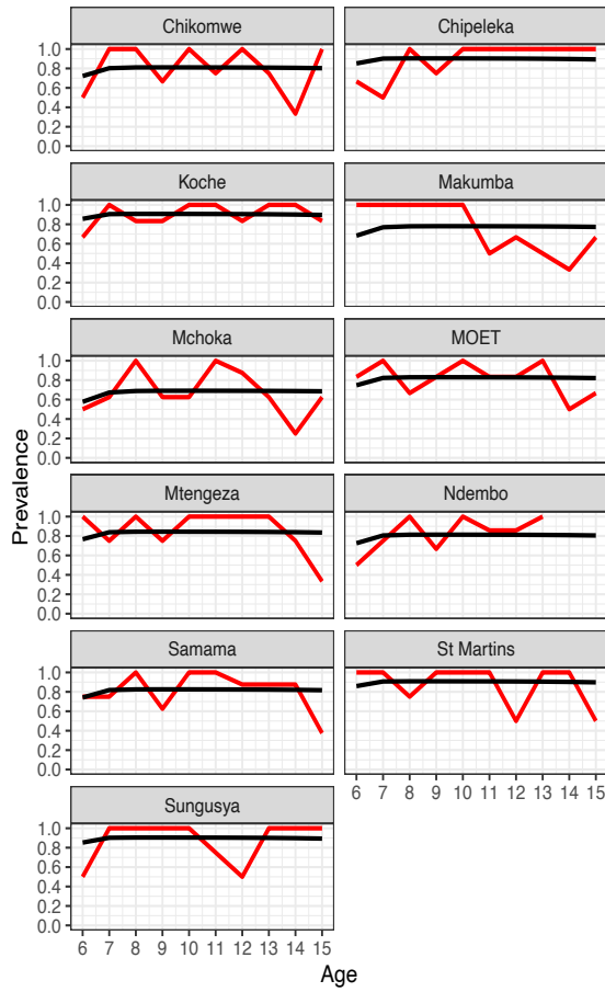
Figure S12: Prior Schistosoma infection prevalence of \alpha = 0.10 for SAC age 6. Multi- \beta_s with space effect model optimisation prevalence prediction (black line) and observed prevalence (red line) against age of SAC carried out for each species a) Biomphalaria sp. b) Bulinus spp.
