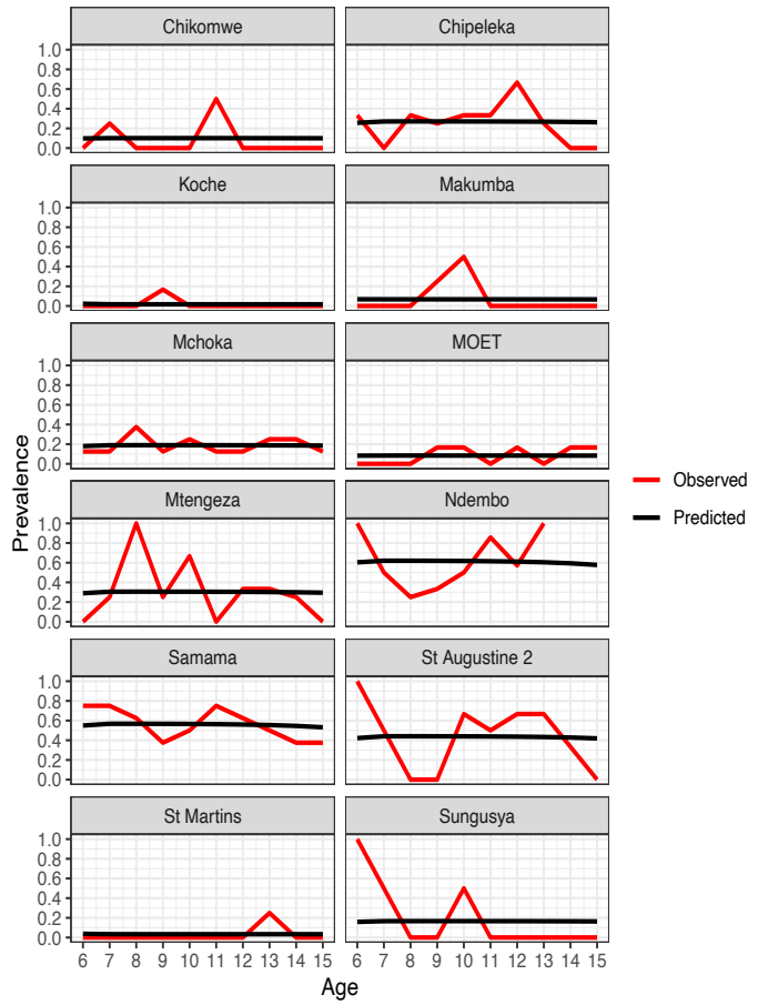
Figure S14: Prior Schistosoma infection prevalence of \alpha = 0.10 for SAC age 6. Multi- \beta_s with no space effect model optimisation prevalence prediction (black line) and observed prevalence (red line) against age of SAC carried out for each species a) Biomphalaria sp. b) Bulinus spp.
