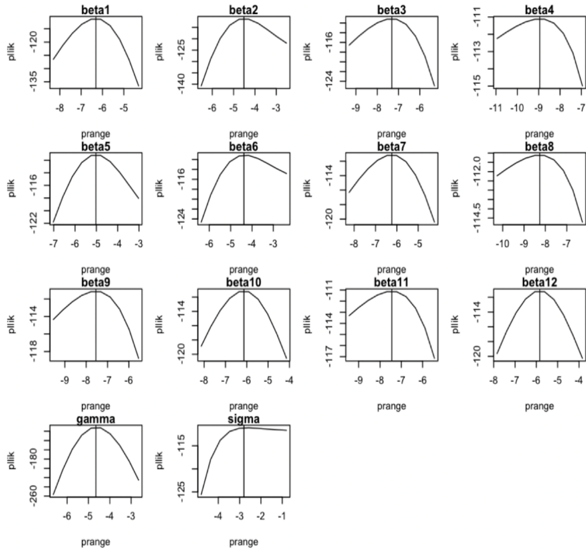
Figure S3: Bulinus sp. Multi- \beta_s with space effect model profile likelihood against fit of model
