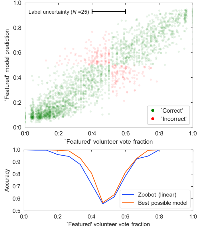
Fig. 13. Detailed model performance for the ‘Smooth or Featured?’ question, illustrating the limitations of classification metrics. Above, the measured ( x -axis) vs. predicted ( y -axis) ‘Featured’ vote fractions, coloured according to whether the binned prediction equals the binned label (‘correct’) or not (‘incorrect’). Classification errors mostly occur for vote fractions where the true label is uncertain (when the label boundary is within our uncertainty on the vote fraction itself). Below, model accuracy as a function of ‘featured’ vote fraction for either Zoobot or a perfect model (see Sect. 4), illustrating that Zoobot is near-perfect within the uncertainty on our labels.
