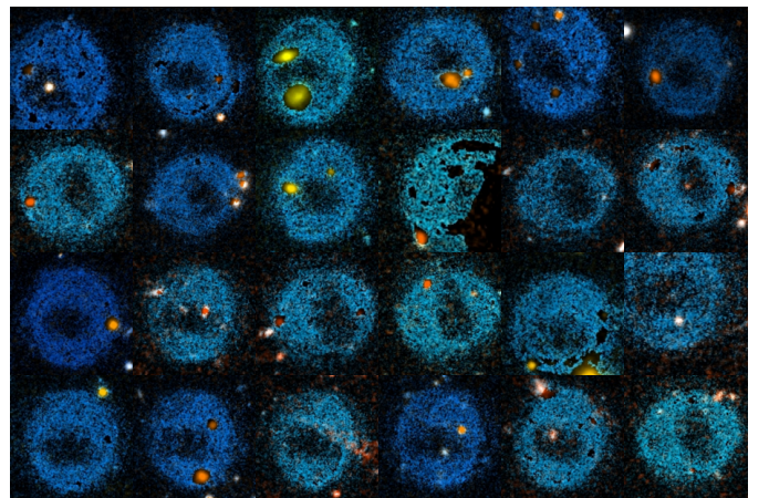
Fig. 11. Q1 sources predicted as most likely to be dichroic ghosts, a well-known artifact caused by internal reflections in telescopes (Euclid Collaboration: Cropper et al. 2025; Euclid Collaboration: Jahnke et al. 2025).
