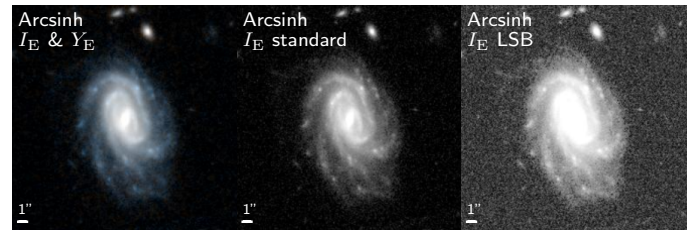
Fig. 3. Example cutouts shown to volunteers. Left to right: I_E and Y_E composite, I_E -only greyscale with standard processing, I_E -only greyscale with enhanced low-surface-brightness processing.
