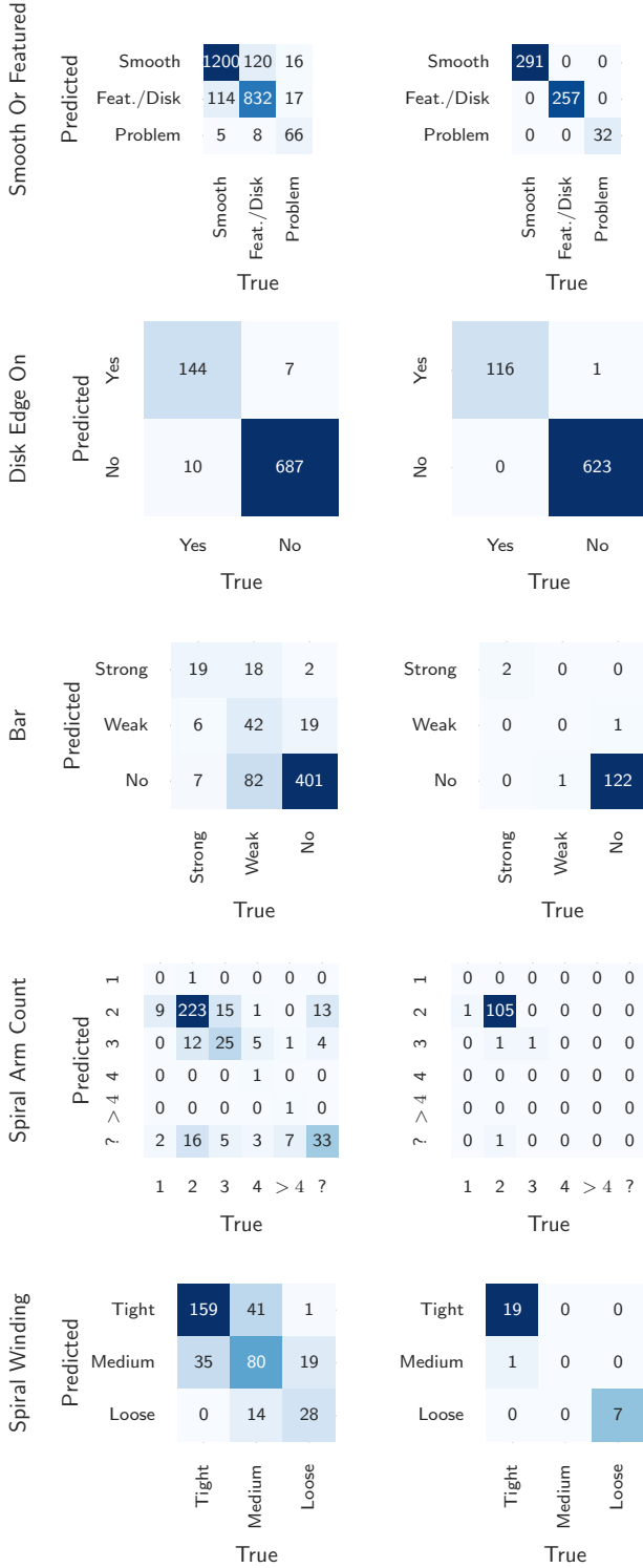
Fig. 12. Confusion matrices for the most commonly-used morphology features. Right column includes only galaxies with high confidence (volunteer vote fraction > 0.8 ) labels. Our model is near-perfect at all questions when evaluated on high-confidence labels. Performance including lower-confidence labels is more mixed, which likely reflects more challenging images for both volunteers and models.
