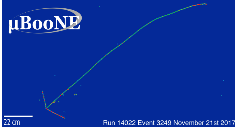
Figure 1: Event display of a candidate \nu_\mu CC2p interaction.
