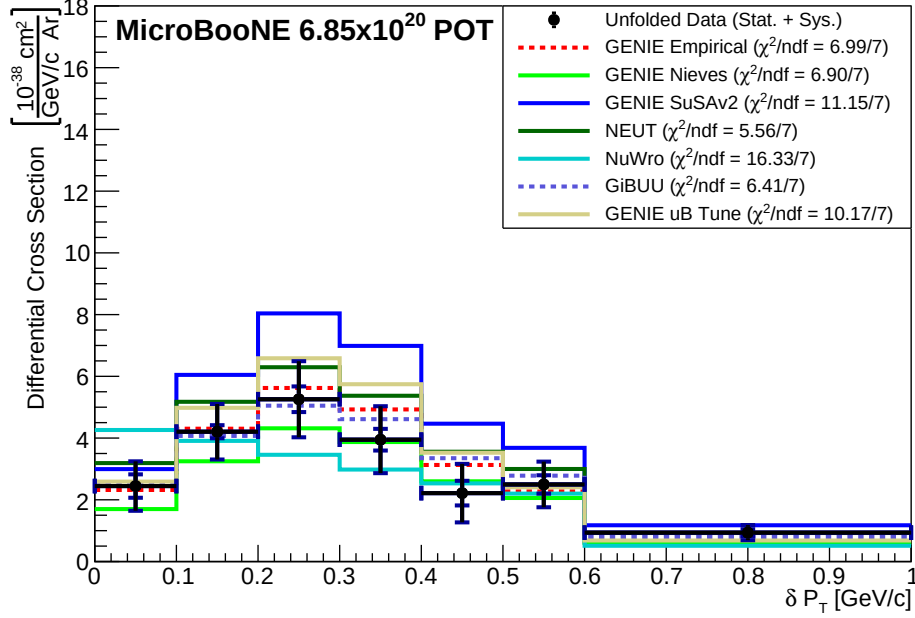
Figure 4: Single differential cross section as a function of the magnitude of the transverse momentum of the final state system, \delta P_T = |\vec{P}_T^\mu + \vec{P}_T^L + \vec{P}_T^R| . The inner error bands on the data represent the statistical uncertainty while the outer error bands represent the systematic uncertainty. A \chi^2/\text{ndf} , considering systematic and statistical uncertainties, is calculated between the data and each model set curve. Details of the generator predictions are given in section 3 .
