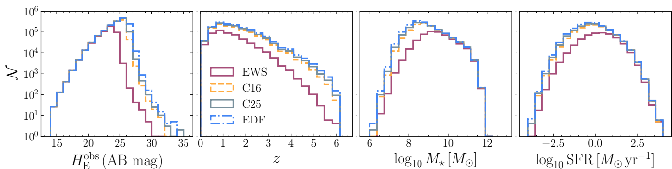
Fig. 2. The four simulated Euclid catalogs used in this work (purple solid , EWS; orange dashed , C16; gray solid , C25; blue dashed-dotted , EDF) are shown as the number of sources as a function of Euclid H_E band magnitude (leftmost panel), redshift (center left), stellar mass (center right), and star-formation rate (rightmost panel). We notice that the magnitude cut upon which the fields are built is an OR condition on the S/N in H_E , I_E filters; as such, simulated galaxies are found below the nominal limiting magnitude cut for H_E band, as those are detected at S/N > 10 in I_E .
