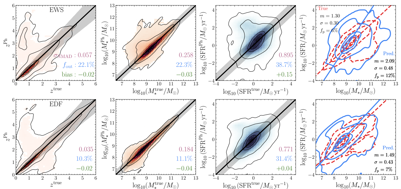
Fig. 3. The Phosphoros results on two simulated Euclid catalogs, EWS (top panels) and EDF (bottom panels), with true values plotted against the Phosphoros recovered ones. The black line is the 1:1 relation; the shaded area is the region beyond which a prediction is an outlier. In every plot, the four contours are the area containing 98%, 86%, 39% (corresponding to the 3\sigma , 2\sigma and 1\sigma levels for a 2D histogram) and 20% of the sample. For SFMS the true distribution is reported in red ( dashed ), the predicted one in blue ( solid ). The lines are the ODR best-fit to the (passive-removed) distribution. The reported metrics are NMAD (purple), the outlier fraction f_{\text{out}} (blue) and the bias (green) for the photometric redshifts and physical parameters, and the slope m , scatter \sigma and fraction of passive galaxies f_p for the SFMS, all defined in Sect. 3.6.
