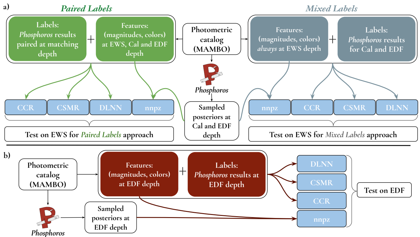
Fig. 4. Flowchart followed for the reported results on the EWS and EDF. Panel a) summarize what has been done for the EWS. In this case, we employed two different approaches: pairing features to labels coming from Phosphoros results at the corresponding depth ( Paired Labels ), or with features always from the Wide simulated catalog and labels coming from Phosphoros results at the Calibration and Deep fields depth for the corresponding sources ( Mixed Labels ). These pairs of (features, labels) – or (features, posteriors for nnpz (see Sect. 3.4) – are thus given as input for the ML models described in Sect. 3. Panel b) illustrates the straighter flowchart for the EDF, where the pairs (features, labels) or (features, posteriors) always come from the simulated Deep field.
