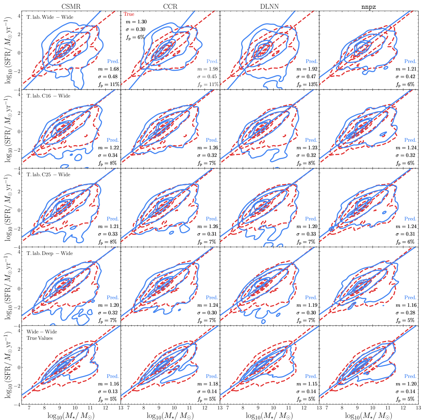
Fig. 8. Same as in Fig. 5, for the SFMS. Red dashed contours are the test SFMS (i.e., the true values), blue solid the predicted one. Contour levels are the same as reported in Fig. 5. The lines are the ODR best-fit to the passive-removed distribution (dashed for test SFMS, solid for predicted). The reported metrics are the SFMS slope, scatter, and fraction of passive galaxies, defined in Sect. 3.6.
