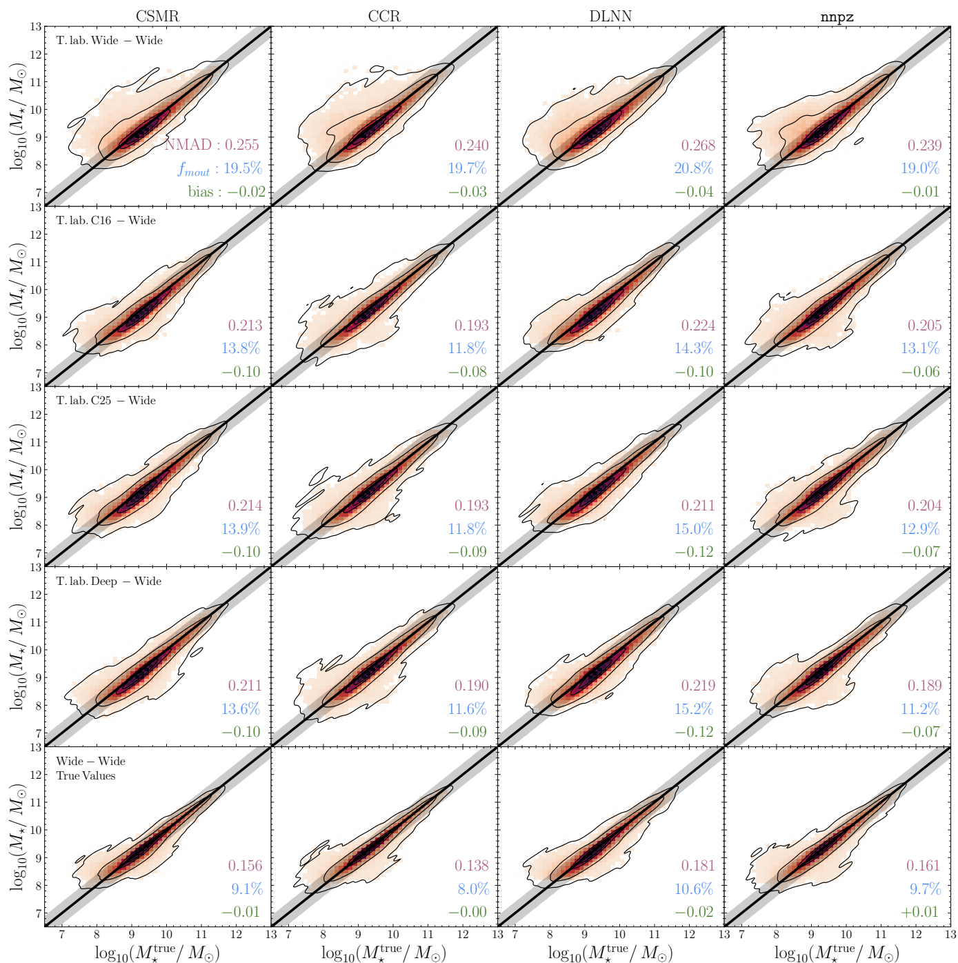
Fig. 6. Same as in Fig. 5, for stellar masses.
