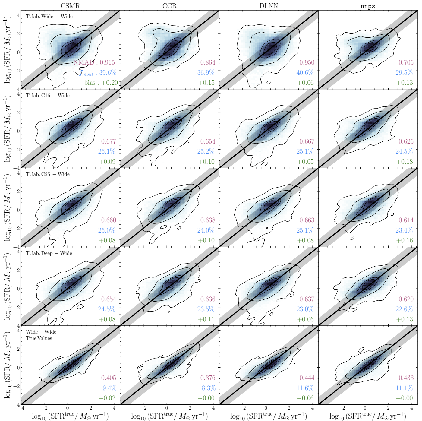
Fig. 7. Same as in Fig. 5, for star-formation rates.
