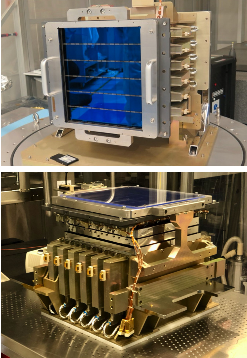
Fig. 10: Two views of the fully-integrated Focal Plane Array. The 36 blue CCDs, supported on the grey SiC detector plane structure, are visible under a protective cover. Below them are two levels of thermal isolation to minimise the parasitic heating of the detectors by the twelve Readout Electronics, which are located below the CCDs (see Figs. 3 and 9) in the body of the Focal Plane Array Electronics Structure. Six Power Supplies for the Readout Electronics are located on two sides of this structure. Spacecraft power is delivered to the connections visible on the Power Supplies, while a SpaceWire data connection to the Control and Data Processing Unit is made to each Readout Electronics in the space below each Power Supply. The harness in the foreground in the lower image is the connection from the Power and Mechanism Control Unit to temperature sensors on the detector plane structure.
