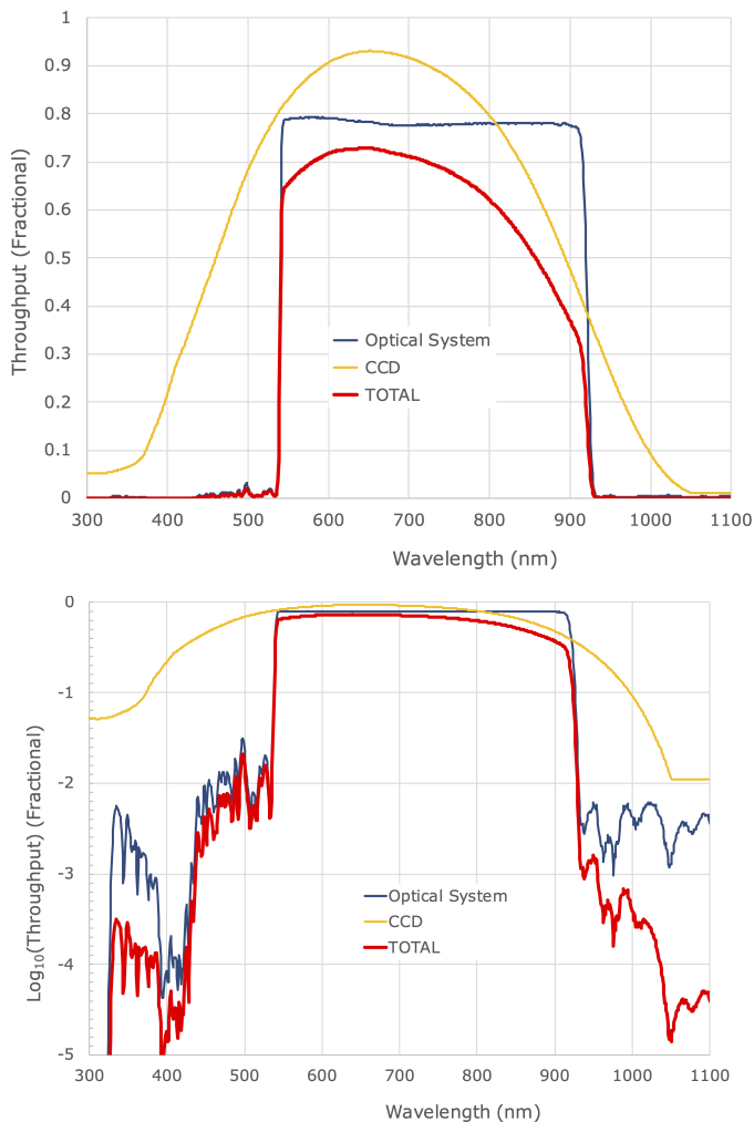
Fig. 7: Top : Throughput as a function of wavelength on a linear scale of the optical elements to VIS (blue) and the Detective Quantum Efficiency of the CCDs (orange), giving the total throughput for this channel (red). Bottom : As for the above but on a log scale to show the definition of the VIS passband.
