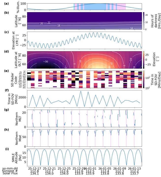
Figure 2. Multi-panel plot showing the same panels as Figure 1. The time-series is zoomed in, showing one month from mid-December 2025 until mid-January 2026.
