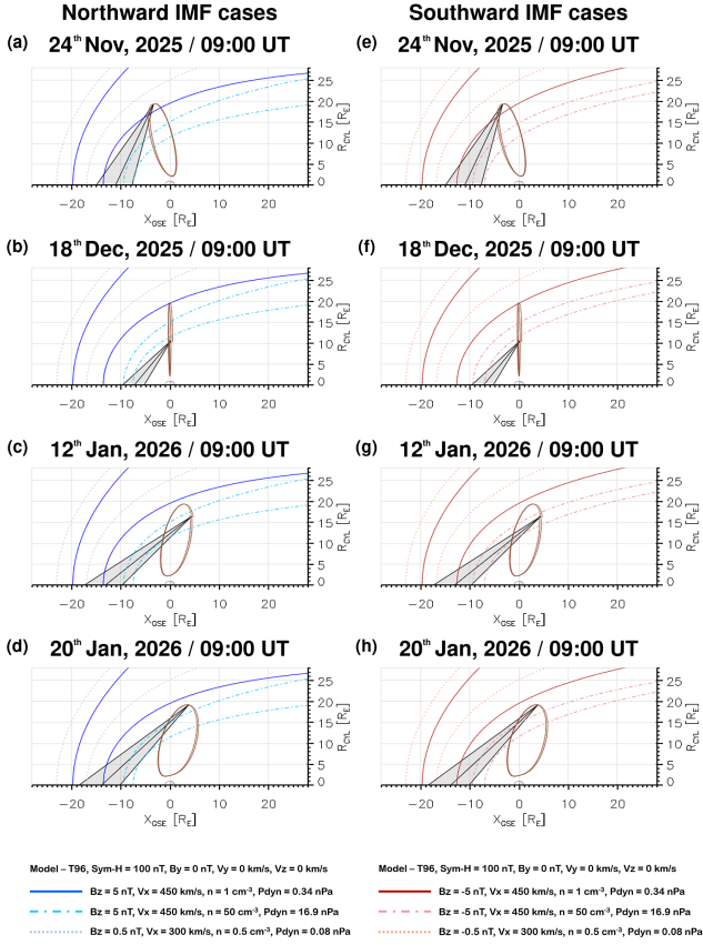
Figure 3. Multi-panel figure showing four example conjunctions from 24 th November 2025 (a and e), 18 th December 2025 (b and f), 12 th January 2026 (c and g) and 20 th January 2026 (d and h). Each panel shows a side-view of the SMILE orbits as it slices the magnetosheath for different possible solar wind conditions, modelled using Geopack with the T96 model (Tsyganenko & Stern 1996). Areas shaded in grey present the configuration of the SMILE SXI field of view for the respective date and time of each panel. The left column shows examples of different northward IMF cases and the right column shows examples of southward IMF cases. Different shades of colour and line-styles display the bow shock and magnetopause locations using the different solar wind conditions, the details of which are listed below the bottom panels of the figure.
