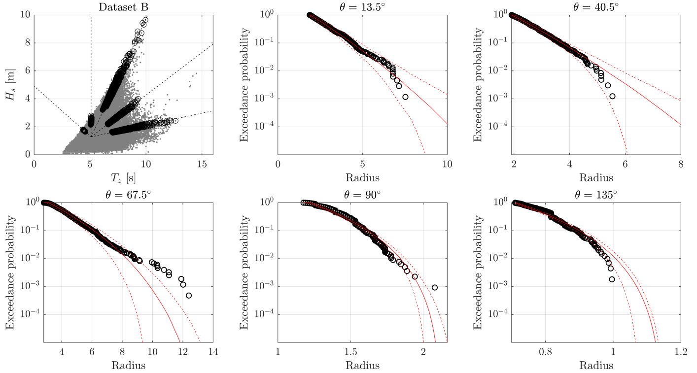
FIGURE 3. COMPARISON OF CONDITIONAL RADIAL EXCEEDANCE PROBABILITIES AT VARIOUS ANGLES, FROM OBSERVATIONS (CIRCLES) AND SPAR MODELS (RED LINES) FOR DATASET B. DASHED LINES INDICATE 95% BOUNDS FOR MODEL QUANTILES. TOP LEFT PLOT SHOWS ALL OBSERVATIONS (DOTS) AND THRESHOLD EXCEEDANCES USED AT EACH ANGLE (CIRCLES).
