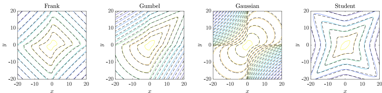
FIGURE 1. CONTOUR PLOTS OF JOINT DENSITIES OF VARIOUS COPULAS ON LAPLACE marginal distributions. ALL COPULAS HAVE PEARSON CORRELATION COEFFICIENT \rho = 0.6 . STUDENT-T COPULA HAS \nu = 2 DEGREES OF FREEDOM. SOLID LINES: TRUE ISODENSITY CONTOURS AT LOGARITHMIC INCREMENTS. DASHED LINES: ISODENSITY CONTOURS OF SPAR APPROXIMATIONS AT THE SAME DENSITY VALUES.
