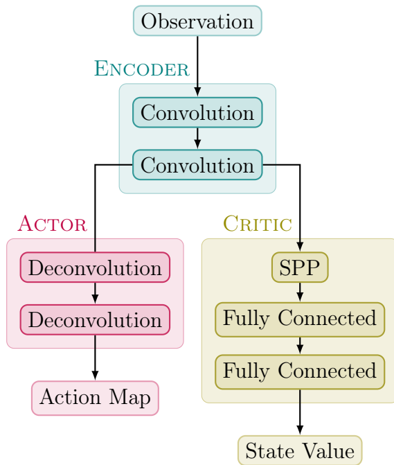
Figure 4: Network Architecture.
