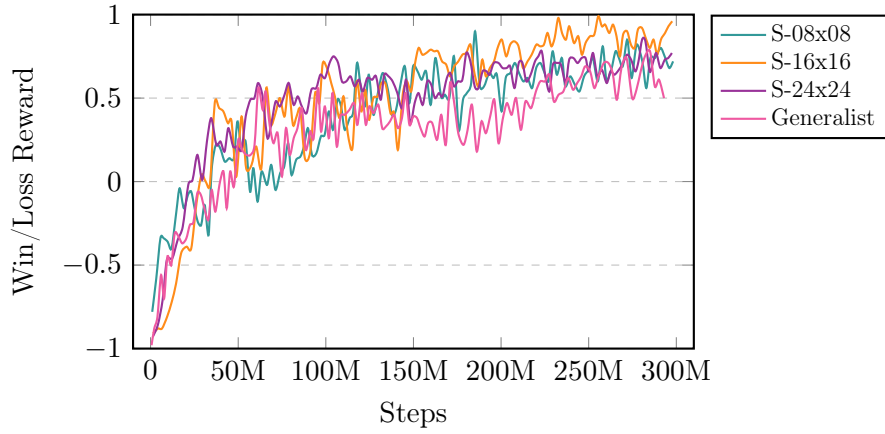
Figure 12: Comparison of win/loss rewards between specialized and generalist models across three map dimensions during training. All models exhibit similar performance trends.
