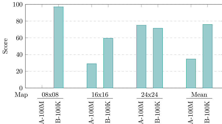
Figure 17: Comparison of models’ scores when the environment is swapped every 100K or 100M steps across three map dimensions. Swapping every 100K steps generally results in better performance, except on the 24 \times 24 map, where swapping every 100M steps yields superior results by a small margin.
