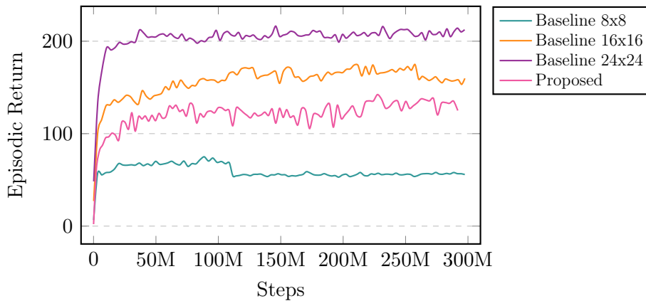
Figure 10: Comparison of episodic returns between proposed and baseline models across three map dimensions in the specialized setting. The proposed model’s performance cannot be directly compared to the baselines’ due to its training on multiple map dimensions, each offering distinct maximum achievable cumulative rewards.
