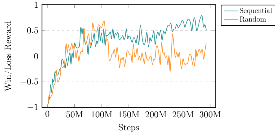
Figure 15: Comparison of win/loss rewards between models using random and sequential environment swap. The sequential method demonstrates a consistent improvement trend over time, whereas the random method experiences significant performance drops.
