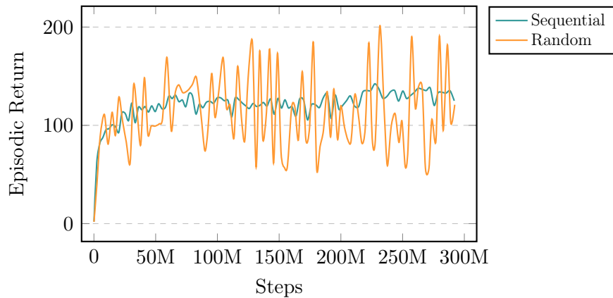
Figure 16: Comparison of episodic returns between models using random and sequential environment swap. The random method exhibits unstable returns compared to the sequential method.
