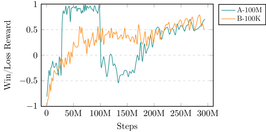
Figure 18: Comparison of win/loss rewards when the environment is swapped every 100K or 100M steps. The model A-100M stays for longer periods on the same map and exhibits significant performance drops when the environment is swapped. Meanwhile the model B-100K exhibits more consistent improvements.
