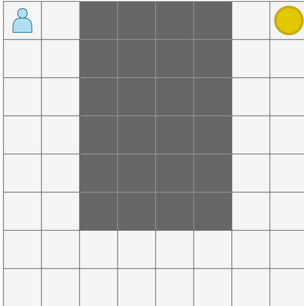
Figure 23: Illustration of the 8 \times 8 Grid Utilized in Our Frozen Lake Experimentation: Starting from the upper-left corner, the objective of the agent is to navigate to the goal located at the upper-right corner. The grid features cells depicted in white, representing frozen terrain that is safe for the agent to traverse, contrasted with the dark cells, which represent holes to be avoided.
