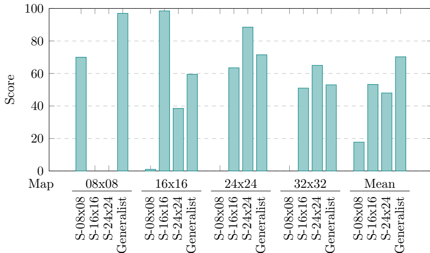
Figure 11: Comparison of specialist and generalist models’ scores across four map dimensions. The generalist model exhibits the best or second-best performance on all maps and achieves the best performance overall.
