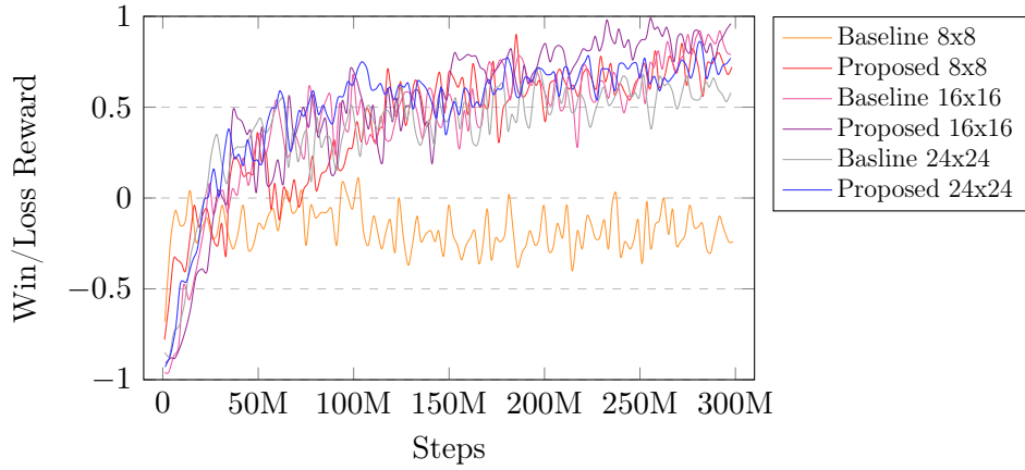
Figure 6: Comparison of win/loss rewards between proposed and baseline models across three map dimensions in the specialized setting. Both models exhibit similar performance trends, except on the 8 \times 8 map, where the baseline model struggled with learning optimal winning strategies over time.
