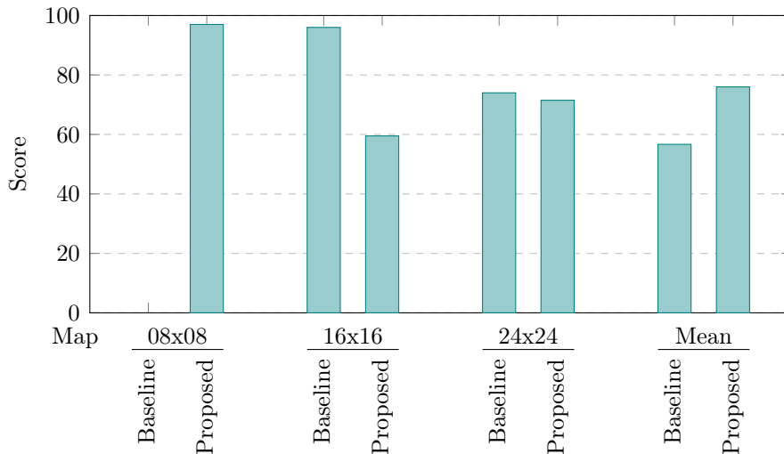
Figure 8: Comparison of proposed and baseline models’ scores across three map dimensions in the generalist setting. The baseline agent outperforms the proposed model in two of the three maps, but the proposed model achieves a greater mean score.
