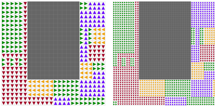
Figure 25: Agent policy transferability: on the left, the policy derived from training on the 24 \times 24 map; on the right, the corresponding policy transferred for a 48 \times 48 map. Despite the difference in map dimensions, the transferred policy closely matches the original policy, with only a few deviations.
