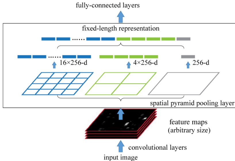
Figure 1: An example of Spatial Pyramid Pooling, assuming that the latest convolution layer yields 256 feature maps. The first SPP level has 16 bins of dimension 256, the second level has 4 bins and the third level has 1 bin. The final representation given by SPP has length (16 + 4 + 1) \times 256 regardless of the input. Source: He et al. (2015).
