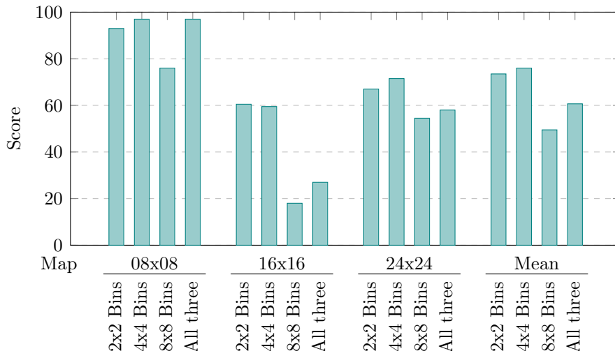
Figure 20: Comparison of models’ scores using different SPP layers across three map dimensions. The model with 4\times 4 bins exhibits the best performance overall and is closely followed by the model with 2\times 2 bins. The model with 8\times 8 shows the lowest performance among all configurations.
