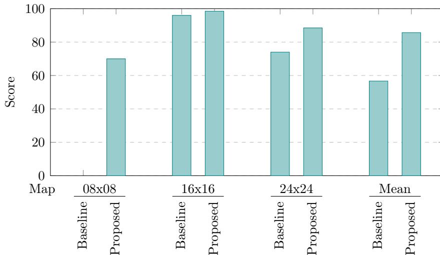
Figure 5: Comparison of proposed and baseline models’ scores across three map dimensions in the specialized setting. The proposed model outperforms the baseline on all tested dimensions.
