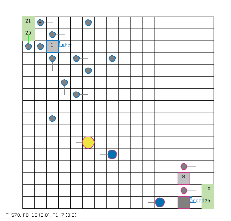
Figure 2: Screenshot of a \mu RTS match in a 16 \times 16 map that showcases distinct units and structures. Circles represent units, their type delineated by size and color, while squares denote various structures, each color-coded for easy identification.
