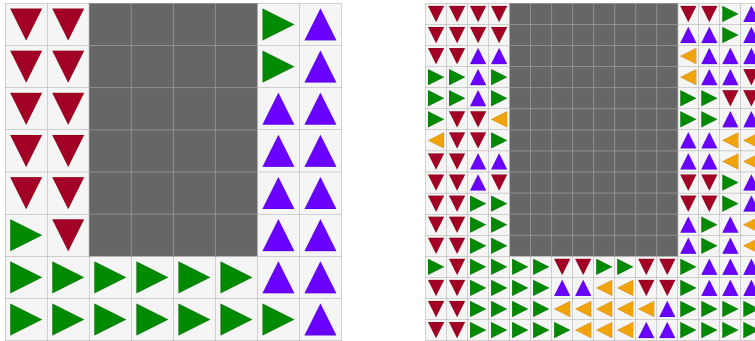
Figure 24: Agent policy transferability: on the left, the policy derived from training on the 8 \times 8 map; on the right, the corresponding policy transferred to a 16 \times 16 map. Significant discrepancies between the policies on each map are evident, indicating a suboptimal transfer.
