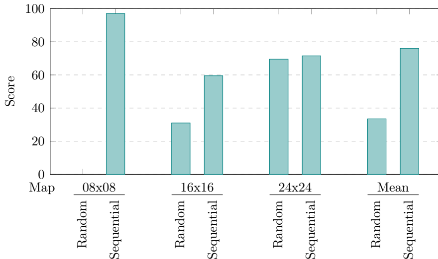
Figure 14: Comparison of models’ scores using random and sequential environment swap across three map dimensions. The sequential method consistently outperforms the random method in all maps.
