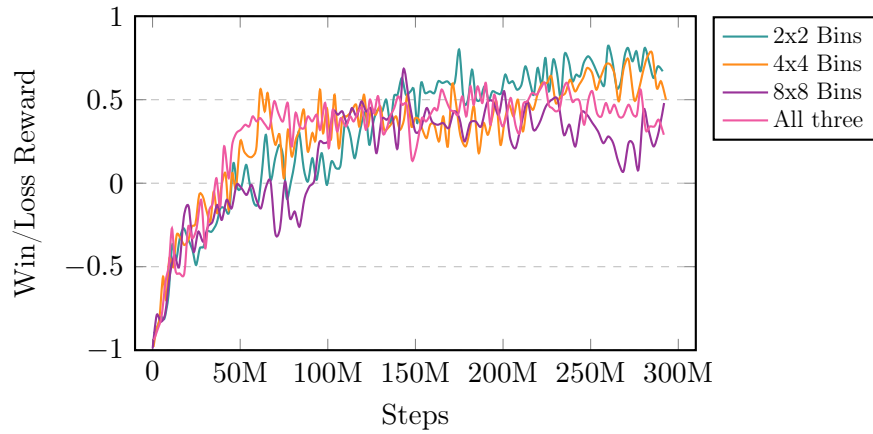
Figure 21: Comparison of win/loss rewards between models using different SPP layers. All models exhibit similar performance trends.
