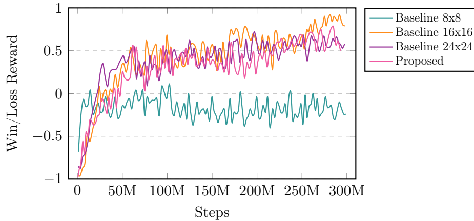
Figure 9: Comparison of win/loss rewards between proposed and baseline models across three map dimensions in the generalist setting. Both models exhibit similar performance trends, except on the 8 \times 8 map, where the baseline model struggled with learning optimal winning strategies over time.
