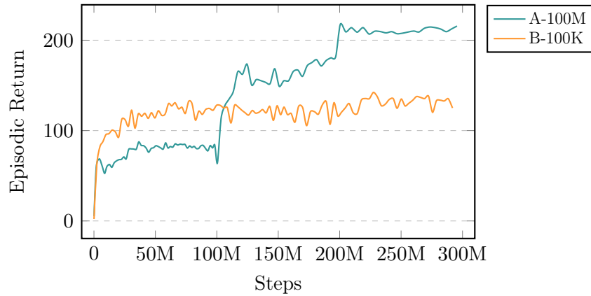
Figure 19: Comparison of episodic returns when the environment is swapped every 100K or 100M steps. Model B-100K, which experiences more frequent swaps, displays a smoother curve. In contrast, Model A-100M shows distinct steps in episodic returns corresponding to each environment swap.
