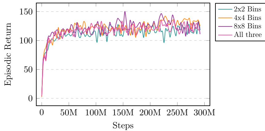
Figure 22: Comparison of episodic returns between models using different SPP layers. All models exhibit similar performance trends.
