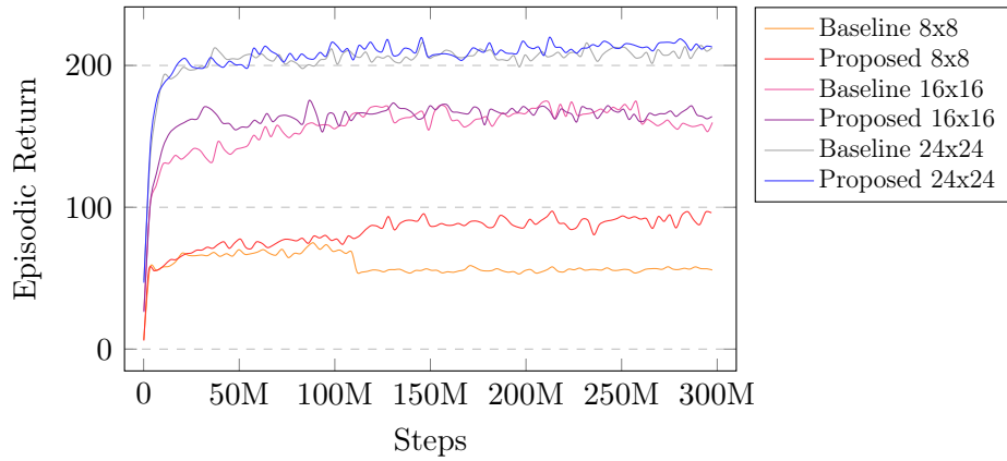
Figure 7: Comparison of episodic returns between proposed and baseline models across three map dimensions in the specialized setting. Both models exhibit similar performance trends, except on the 8 \times 8 map, where the baseline model struggled with learning optimal winning strategies over time. Larger maps result in longer games, leading to greater cumulative rewards per game for the agents.
