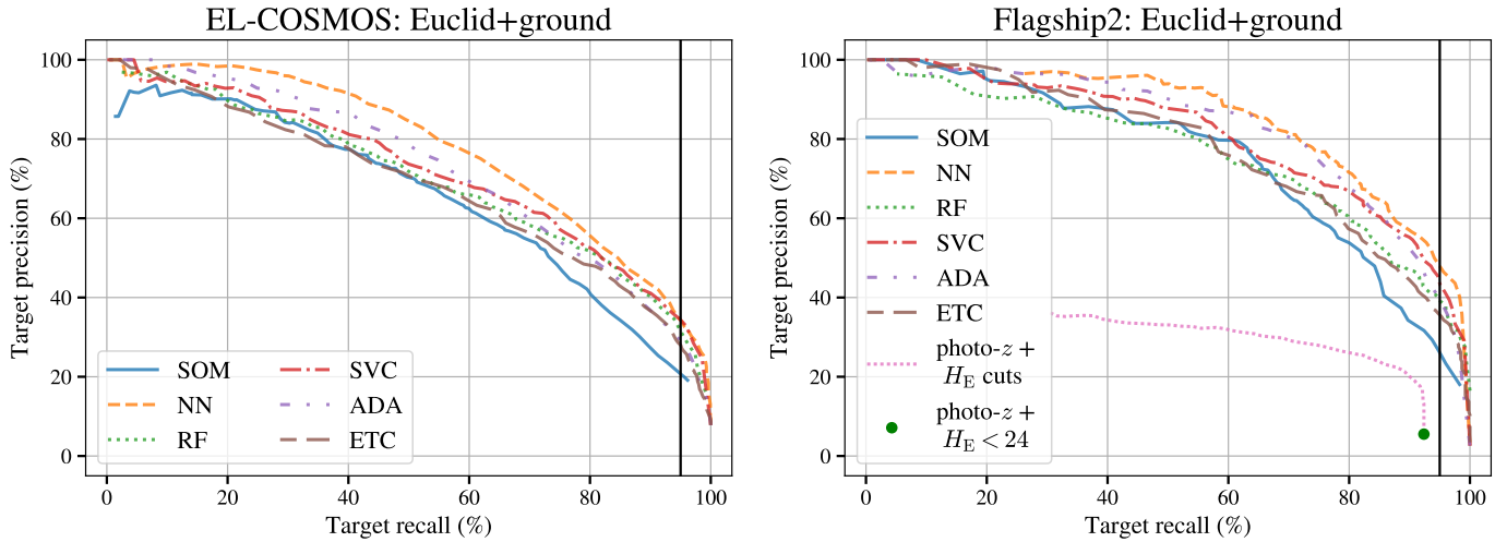
Fig. 7. Precision versus recall curves for the analyses with Euclid photometry and ground-based photometry. Left : results for EL-COSMOS. Right : results for Flagship2. The dotted magenta line represents the photo- z selection for a range of H_E magnitude limits. The green marker indicates the photo- z selection with H_E < 24 .
