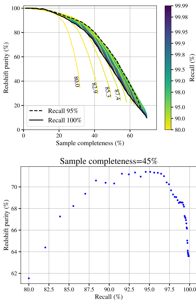
Fig. 12. Spectroscopic redshift purity and completeness with the addition of the photometric classification. Top : the curves are colour-coded as a function of the recall of the photometric classification. The spectroscopic reliability threshold varies along each curve, while varying the threshold on the photometric classification probability shifts the curve. The purity improves as recall increases, reaching a maximum for recall \sim 95\% and declining after. For better visualisation, the first lines are labelled with the corresponding recall value. At recall values above 95\% the curves are tightly packed. The solid black line corresponds to 100\% recall, while the dashed line to 95\% recall, the value we chose to benchmark our results. Bottom : redshift purity as a function of the recall of the photometric classification, fixing the value of sample completeness to 45\% .
