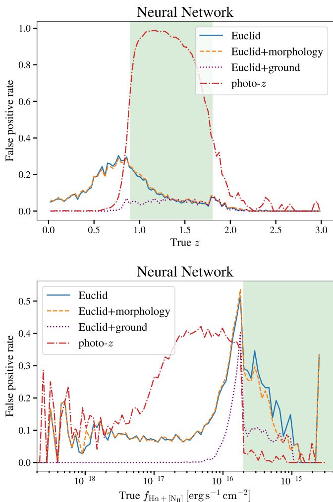
Fig. 10. False positive rate as function of redshift and f_{H\alpha+[NII]} for Flagship2. The plot allows us to identify the origin of non-targets that enter the selected samples. The solid blue, dashed orange, and dotted purple curves, respectively, correspond to the neural networks trained with Euclid photometry, Euclid plus morphological data, and Euclid plus ground-based photometry. The dash-dotted red line is the false positive rate of the photo- z selection. Top : False positive rate as a function of z . The green shaded area marks the target redshift range. Bottom : False positive rate as a function of f_{H\alpha+[NII]} . The green shaded area corresponds to the H\alpha limiting flux. There is a peak in the false positive rate just below the flux limit used to define the target sample, although we note that these galaxies can still give correct redshift measurements.
