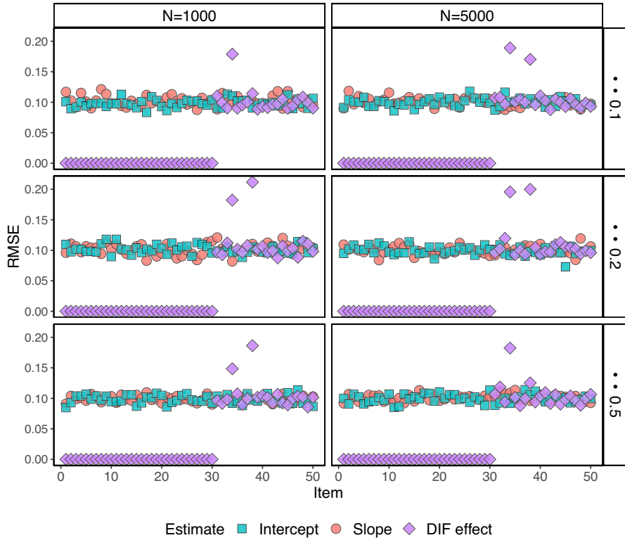
FIGURE 3. RMSE for J = 50 under the 2-group setting.
