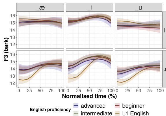
FIG. 10. The F_3 (Bark) trajectories illustrating differences between the different proficiency groups among L1 Japanese speakers predicted by GAMMs over the liquid-vowel intervals for each liquid (rows) in each vowel context (columns). Each panel shows predictions based on the model excluding parametric and smooth terms associated with gender for simplicity, with a mean smooth and 95% confidence interval for advanced (blue), intermediate (red), beginner (green) L1 Japanese speakers and L1 English speakers (orange). (Colour online)
