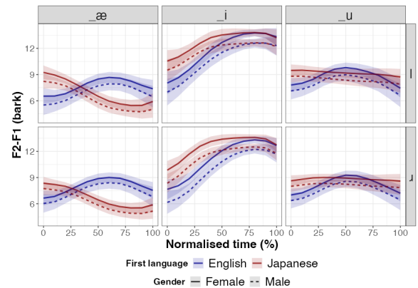
FIG. 7. The F_2-F_1 (Bark) trajectories predicted by GAMMs over the liquid-vowel intervals for each liquid (rows) in each vowel context (columns). Each panel shows predictions based on the full model with a mean smooth and 95% confidence interval for L1 English (blue) and L1 Japanese (red) speakers and for female (solid) and male (dashed) speakers. (Colour online)
