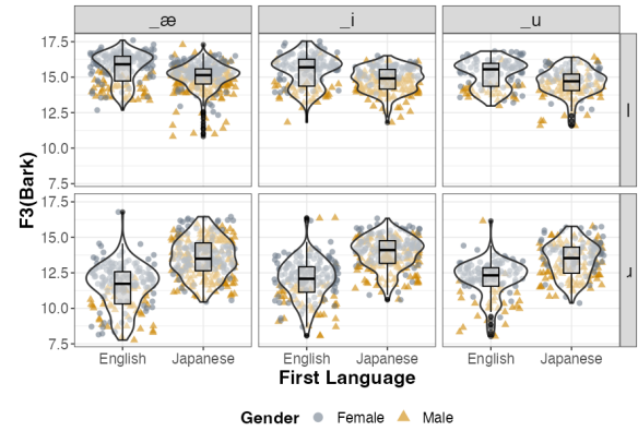
FIG. 4. F_3 (Bark) at liquid midpoint. Each column shows vowel contexts for /l/ (top row) and /ɹ/ (bottom row). Each panel shows distributions of F_3 (Bark) for L1 English (left) and L1 Japanese (right) speakers. Overlaid is the scatter plot indicating speaker’s gender: female (grey circles) and male (yellow triangles) speakers.
