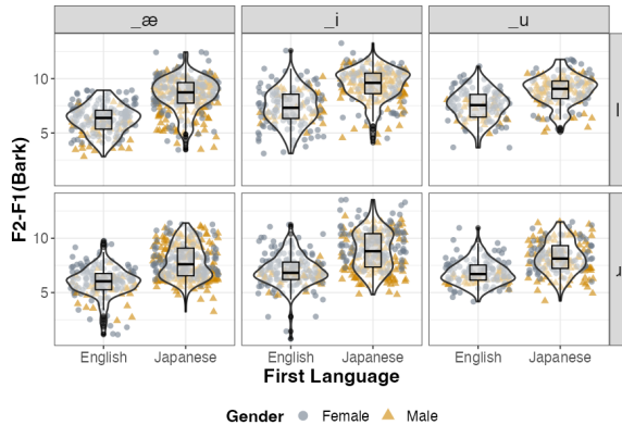
FIG. 3. F_2-F_1 (Bark) at liquid midpoint. Each column shows vowel contexts for /l/ (top row) and /ɹ/ (bottom row). Each panel shows distributions of F_2-F_1 (Bark) for L1 English (left) and L1 Japanese (right) speakers. Overlaid is the scatter plot indicating speaker’s gender: female (grey circles) and male (yellow triangles) speakers. (Colour online)
