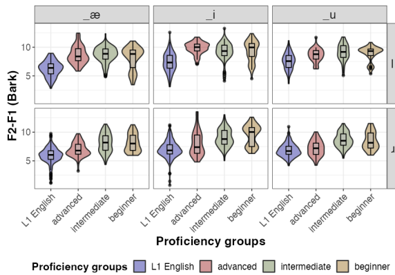
FIG. 5. F_2-F_1 (Bark) at liquid midpoint by proficiency groups. Each column shows vowel contexts for /l/ (top row) and /ɹ/ (bottom row). Each panel shows distributions of F_2-F_1 (Bark) for L1 English speakers and three groups of L1 Japanese speakers: advanced, intermediate and beginner, from left to right. (Colour online)
