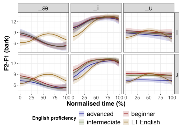
FIG. 9. The F_2-F_1 (Bark) trajectories illustrating differences between the different proficiency groups among L1 Japanese speakers predicted by GAMMs over the liquid-vowel intervals for each liquid (rows) in each vowel context (columns). Each panel shows predictions based on the model excluding parametric and smooth terms associated with gender for simplicity, with a mean smooth and 95% confidence interval for advanced (blue), intermediate (red), beginner (green) L1 Japanese speakers and L1 English speakers (orange). (Colour online)
