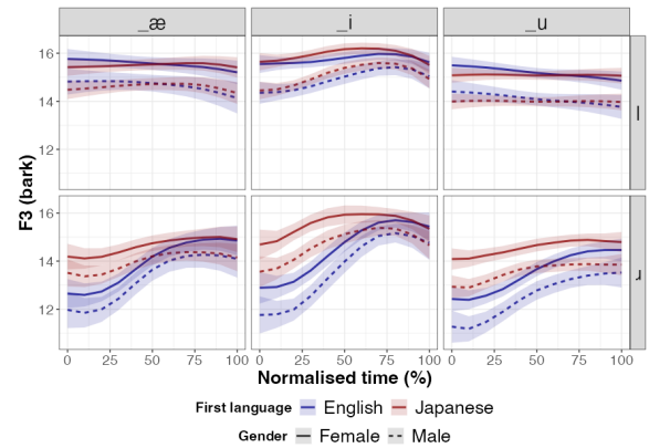
FIG. 8. The F_3 (Bark) trajectories predicted by GAMMs over the liquid-vowel intervals for each liquid (rows) in each vowel context (columns). Each panel shows predictions based on the full model with a mean smooth and 95% confidence interval for L1 English (blue) and L1 Japanese (red) speakers and for female (solid) and male (dashed) speakers. (Colour online)
