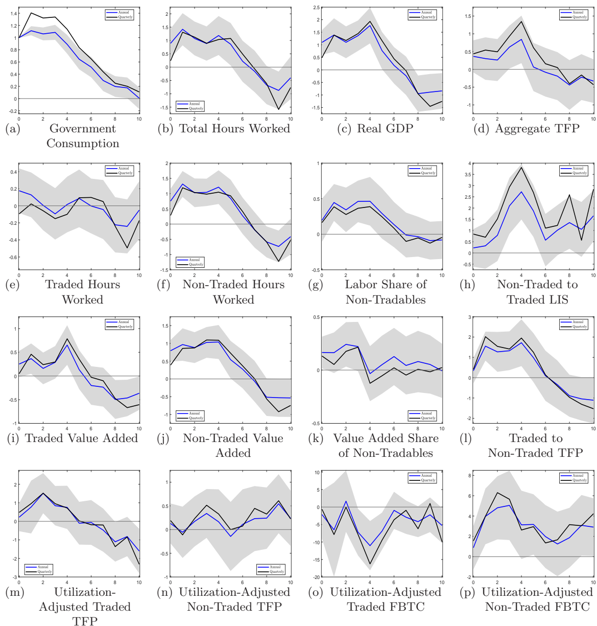
Figure 17: Addressing Endogeneity Issue: Identification on Quarterly vs. Annual Data. Notes: The solid blue line and solid black line show the response of aggregate and sectoral variables to an exogenous increase in government final consumption expenditure by 1% of GDP when we identify the government spending shock by using Blanchard and Perotti [2002] identification method. In the blue line, we identify government spending shocks on annual data and in the solid black line, we identify the government spending shock on quarterly data. Shaded areas indicate the 90 percent confidence bounds. We estimate the dynamic effects by using Jordà's [2005] single-equation method. Horizontal axes indicate years. Vertical axes measure percentage deviation from trend in GDP units (sectoral value added, sectoral value added share, labor income share), percentage deviation from trend in total hours worked units (sectoral hours worked, labor share), percentage deviation from trend (sectoral TFPs, sectoral FBTC). Sample for annal data : 17 OECD countries, 1970-2015. Sample for quarterly data : 17 OECD countries, 1970q1-2015q4
