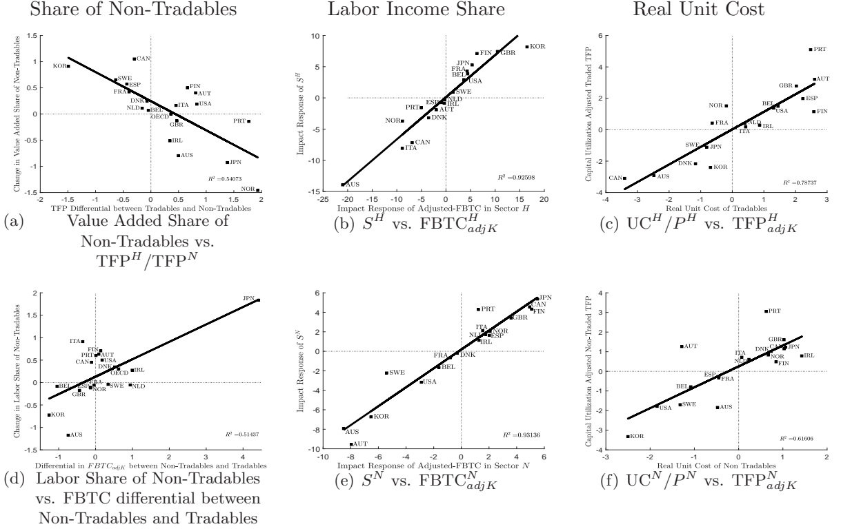
Figure 11: Effects of Government Spending Shocks and Cross-Country Differences in Technology Adjustment. Notes: Fig. 11 plots responses to an exogenous increase in government consumption by 1% of GDP against measures of technological change. Fig. 11(a) plots the present value of the cumulative change in the value added share of non-tradables, \nu_t^{Y,N} (vertical axis) against the present value of the cumulative change in the ratio of traded TFP to non-traded TFP (horizontal axis), both computed over a six-year horizon and divided by the present value of the cumulative change in government consumption. In accordance with eq. (48), the TFP differential is scaled by multiplying by (1 - \nu^{Y,H}) \nu^{Y,H} . Fig. 11(d) plots the present value of the cumulative change in the share of non-traded hours worked in total hours worked (vertical axis) against the present value of the cumulative change in the differential in capital-utilization-adjusted FBTC between non-tradables and tradables (horizontal axis), both computed over a six-year horizon and divided by the present value of the cumulative change in government consumption. To construct time series for FBTC_{t,adjK}^j for each country, we use eq. (5) and take estimates of the elasticity of substitution between capital and labor \sigma^j from columns 18 and 19 of Table 7. The response of FBTC_{t,adjK}^j in sector j is adjusted with 1 - s_L^j and the differential is scaled by \alpha_L^H \alpha_L^N , see eq. (67) in Online Appendix C. The second column of Fig. 11 plots impact responses of sectoral LISs (vertical axis) against the adjustment of capital-utilization adjusted FBTC (the horizontal axis). The third column of Fig. 11 plots impact responses of the ratio of the unit cost for producing to the value added deflator (vertical axis) against the adjustment of capital-utilization adjusted TFP (horizontal axis). The construction of the unit cost for producing is detailed in Online Appendix H. Sample: 18 OECD countries, 1970-2015, annual data.
