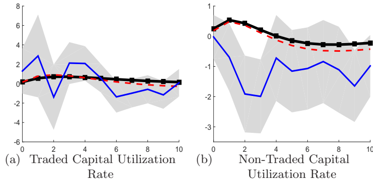
Figure 41: Theoretical vs. Empirical Responses Following Unanticipated Government Spending Shock: Capital Utilization Rate. Notes: Solid blue line displays point estimate of VAR with shaded areas indicating 90% confidence bounds. The solid black line with squares displays model predictions in the baseline scenario with capital and technology utilization together with FBTC. Whilst in the baseline scenario we assume that taxes are lump-sum, the dashed red line shows results for the same model when we allow for distortionary (i.e., labor and consumption) taxation.
