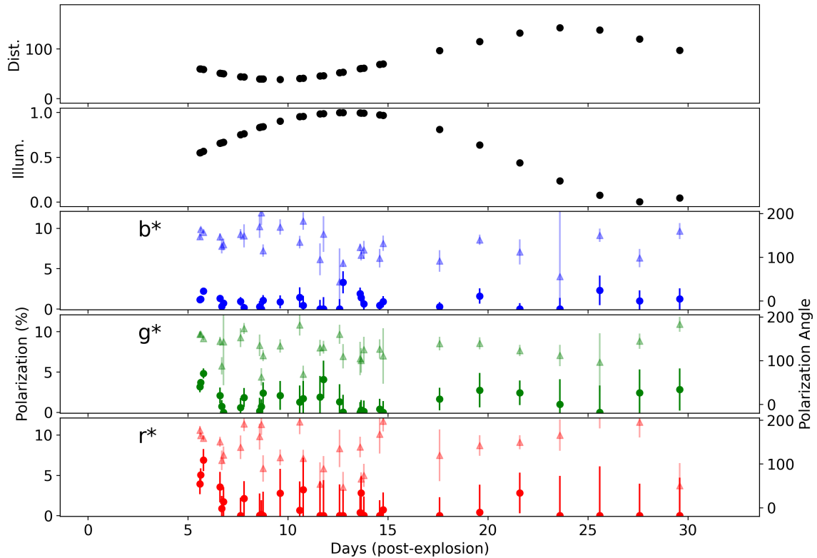
Figure 4. The evolution of the degree of polarization ( \bullet ) and polarization angle ( \blacktriangle ) of AT2018cow, in the three RINGO3 bands b^*/g^*/r^* (lower panels) with respect to changing moon distance (top panel) and illumination (second panel) over the period of observations.
