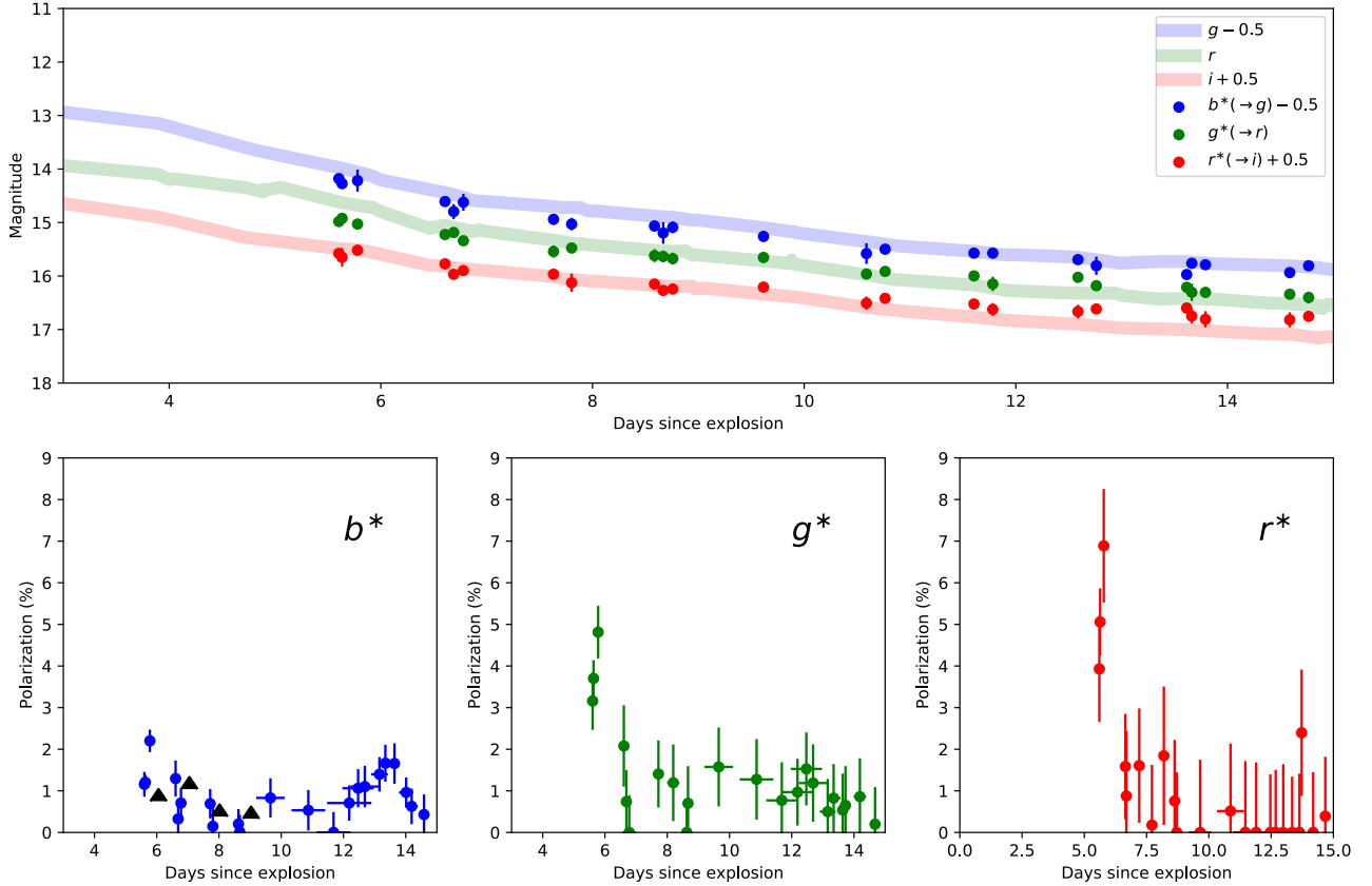
Figure 2. The observed evolution of the polarization of AT2018cow measured in the RINGO3 b^* (blue), g^* (green) and r^* (red) bands. Top panel ) The lightcurve of AT2018cow (Perley et al. 2019) (solid lines) and overlaid are photometry derived from the RINGO3 observations transformed to the approximately equivalent filters of the Sloan Digital Sky Survey. Bottom panels ) The polarization of AT 2018cow measured by RINGO3 in the b^* , g^* and r^* bands, for which the temporal binning of the data has been chosen to fix the precision of each binned data point (see text). The black triangles are observations of AT2018cow acquired with the 2.3m Bok telescope (Smith et al. 2018), approximately consistent with the RINGO3 b^* band (the reported uncertainties are smaller than the size of the points)
