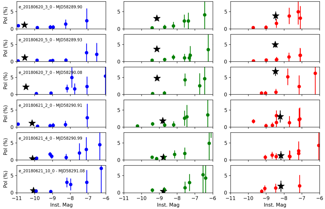
Figure 3. The polarization of sources in the field surrounding AT 2018cow in the b^* (left), g^* (middle) and r^* (right) bands for the first six epochs (corresponding to the first two nights of observations). The polarization values have been corrected for bias, using the expression of Wang et al. (1997). In each panel AT2018cow is indicated by the \star symbol. For the first 3 epochs, the polarization of AT 2018cow exhibits an excess (particularly in the g^* and r^* bands) compared to other sources in the field of similar brightness.
