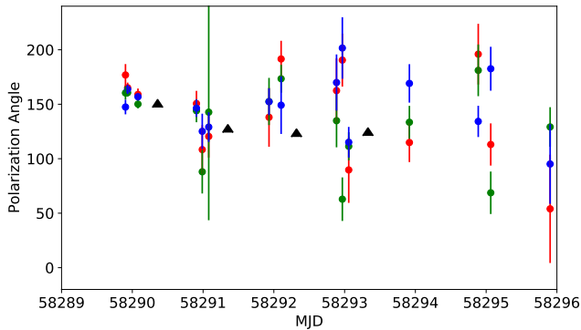
Figure 5. Evolution of the polarization angle of AT2018cow. The black triangles are measurements made with the 2.3m Bok Telescope and are most directly comparable with the measurements made in the RINGO3 b^* channel. It is important to note that the increased scatter in the polarization angle, measured by RINGO3 at later times, is correlated with the decrease in both the brightness and polarization of AT 2018cow.
