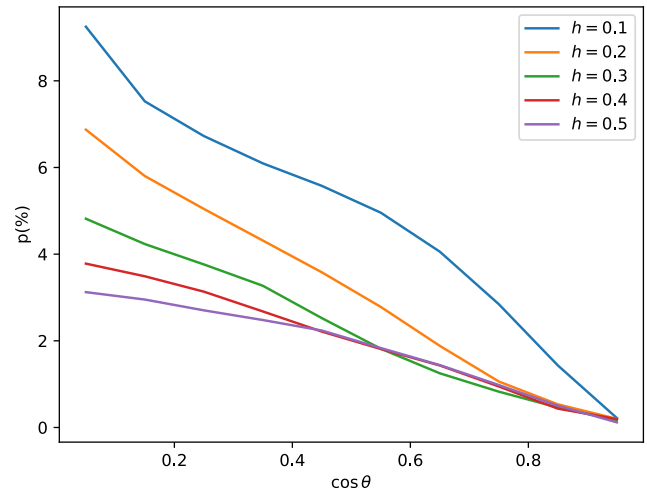
Figure 7. The predicted polarization as a function of the inclination angle \theta for models of flat disks with optical depth of \tau = 5.0 and thickness h (relative to the projected maximum extent of the disk on the sky).
