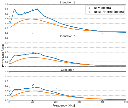
Figure 12. Fast Fourier transforms (FFTs) of noise waveform data collected by the ICARUS TPCs, before and after filtering of coherent noise. Results are shown separately for the Induction 1 plane (top), Induction 2 plane (middle), and Collection plane (bottom).
