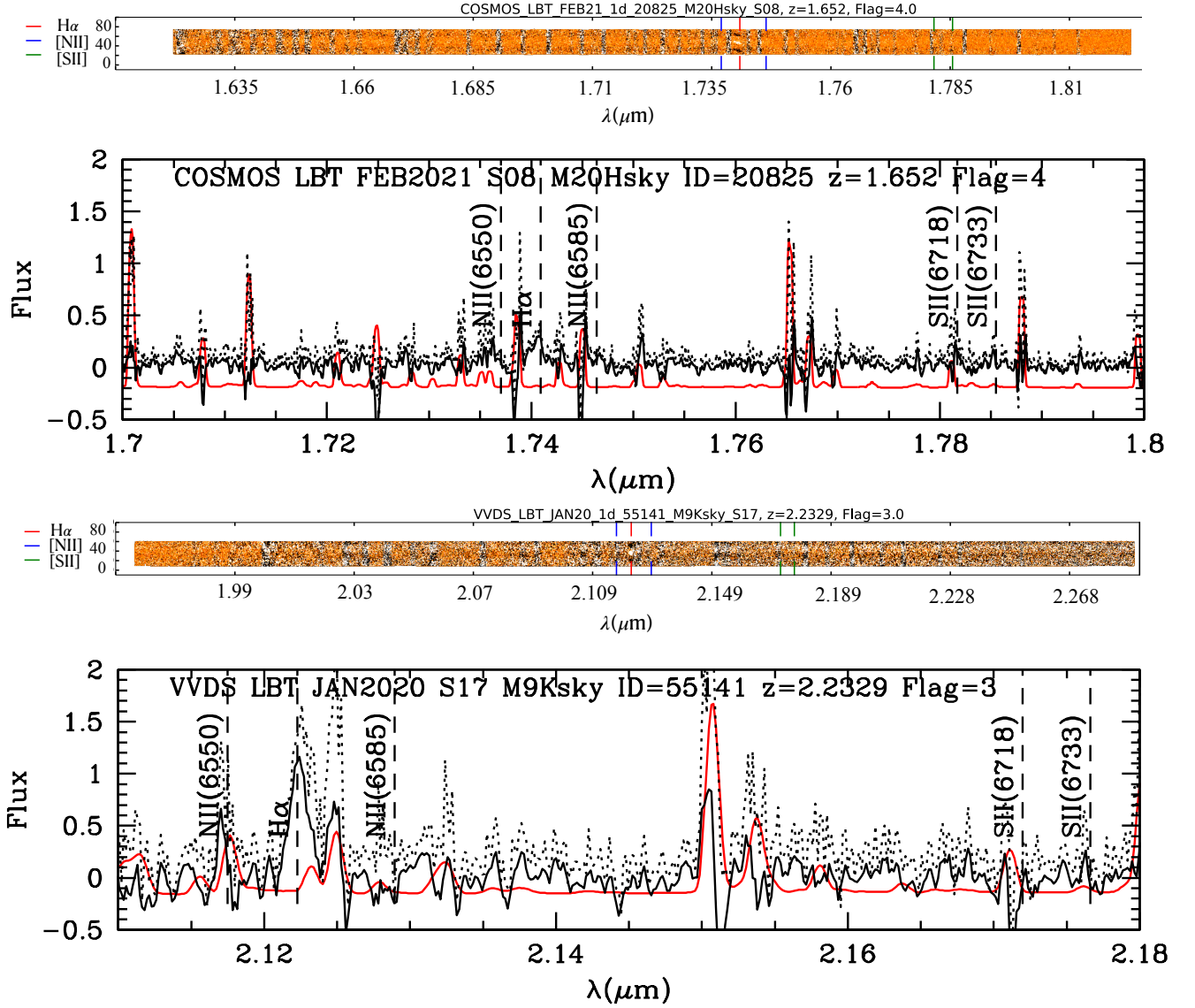
Fig. 3: One- and two-dimensional spectra with Flag = 4, 3.5, 3 of objects with z_{\text{meas}} < 2 . The two-dimensional spectra are 10 arcsec wide, with the vertical scale given in pixels, and show the whole wavelength range (in \mu\text{m} ) observed. The one-dimensional spectra show the wavelength range around the relevant emission lines; the black solid lines show the measured flux (in arbitrary units with a 3 pixel smoothing), the dotted lines the flux without smoothing plus its errors, the red lines the sky (scaled down by a factor of 1000 and shifted by -0.2 flux units). The vertical dashed lines mark the emission lines (with vacuum rest-frame wavelengths in \text{\AA} ) used (when visible) to measure the spectroscopic redshift (not yet corrected to the heliocentric system).
