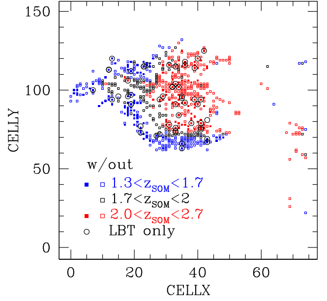
Fig. 11: Filled squares show cells probed by the current spectroscopic release, empty squares cells still lacking spectroscopy. Blue cells have 1.3 < z_{\text{phot,SOM}} < 1.7 , black cells have 1.7 < z_{\text{phot,SOM}} < 2.0 , and red cells have 2.0 < z_{\text{phot,SOM}} < 2.7 . Open circles mark the 49 cells without spectroscopy before this release. The circles without a centered square have z_{\text{phot,SOM}} outside the probed range.
