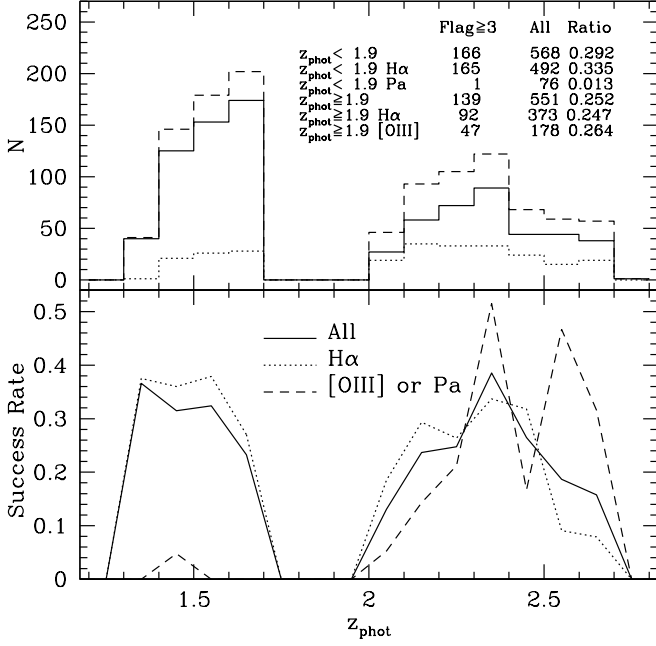
Fig. 9: Top : histogram of z_{\text{phot}} of targeted galaxies (dashed), targeting H \alpha (full lines) and the [O III] or Pa lines (dotted). Bottom : the success rate as a function of z_{\text{phot}} considering all lines (H \alpha , [O III], Pa, full line), based on H \alpha only (dotted line), or on [O III] or Pa (dashed line).
