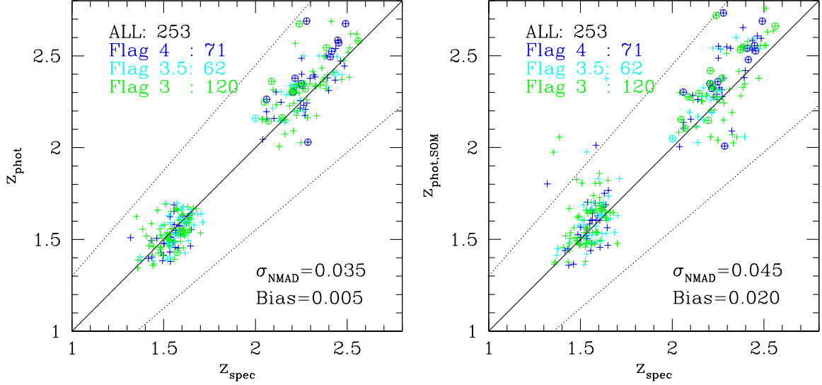
Fig. 6: Left : comparison between z_{\text{phot}} and z_{\text{spec}} for high-quality (Flag \geq 3 ) redshift galaxies observed during the LBT campaign. Crosses show spectroscopic redshifts determined from the H \alpha line, circles with crosses from the [O III] lines. The dotted lines define the region outside which the z_{\text{phot}} is considered a ‘catastrophic failure’, defined by a redshift error |z_{\text{phot}} - z_{\text{spec}}|/(1 + z_{\text{spec}}) \geq 0.15 . Right : same as the left panel but comparing z_{\text{phot,SOM}} and z_{\text{spec}} . The values of \sigma_{\text{NMAD}} = 1.48 \text{Median}(|z - z_{\text{spec}}|/(1 + z_{\text{spec}})) and Bias = Mean( (z - z_{\text{spec}})/(1 + z_{\text{spec}}) ) are also given, with z = z_{\text{phot}} in the left and z = z_{\text{phot,SOM}} in the right plot.
