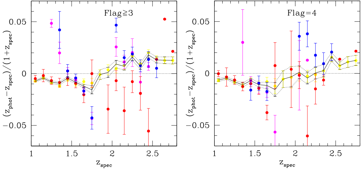
Fig. 7: Left : the mean differences in bins of (z_{\text{phot}} - z_{\text{spec}})/(1 + z_{\text{spec}}) of non-catastrophic failures as a function of z_{\text{spec}} for Flag \geq 3 redshifts released by the C3R2 project: yellow from Masters et al. (2015, 2017, 2019); magenta from G2020; red from Euclid Collaboration: Stanford et al. (2021); blue, this paper. The black line shows the average in bins of the whole sample, the dotted lines the error range. Right : the same for Flag = 4 redshifts.
