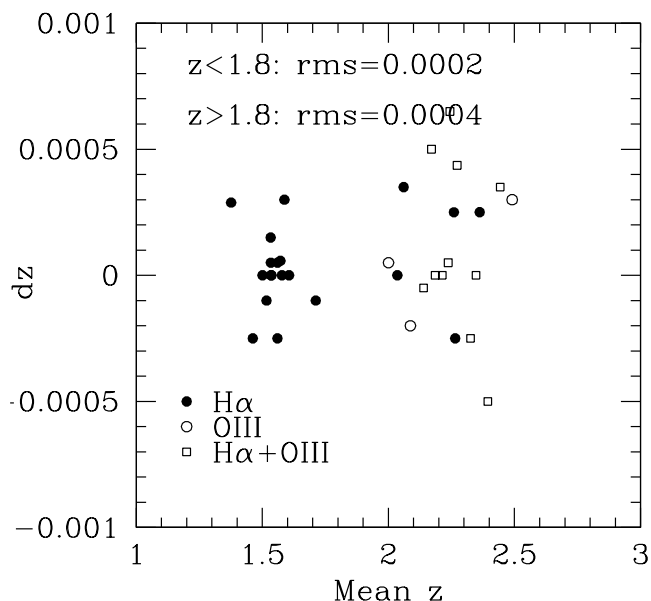
Fig. 5: Errors from repeated observations. The filled circles show the differences dz between the spectroscopic redshifts determined from two or more spectra of the same objects using the H\alpha line (if more than two spectra were collected, we show the difference to the average of the measurements). The open circles show differences between redshifts based on the [O\text{III}] lines; the open squares show differences between redshifts measured using the H\alpha and the [O\text{III}] lines.
