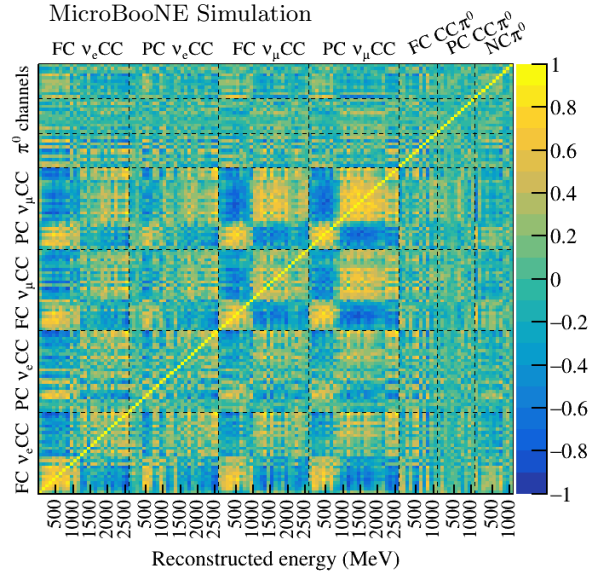
FIG. 17: Correlations of total detector systematics for the seven channels. The correlations between the FC and PC \nu_\mu CC channels are dominated by the components of light yield and recombination.
