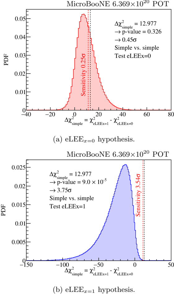
FIG. 27: Distributions of simple-vs-simple \Delta\chi^2_{\text{simple}} assuming (a) the eLEE x =0 hypothesis is true and (b) the eLEE x =1 hypothesis is true. Both distributions are obtained from 4 million pseudo experiments. Data \Delta\chi^2_{\text{simple}} values are indicated by dashed vertical lines.
