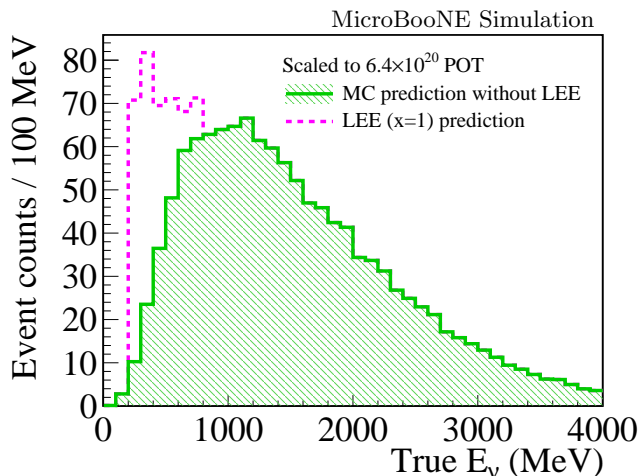
FIG. 1: Expected \nu_e CC events in the MicroBooNE detector for eLEE_{x=1} hypothesis and eLEE_{x=0} hypothesis as a function of true neutrino energy at 6.4 \times 10^{20} proton-on-target (POT) exposure, assuming 100% detection efficiency.
