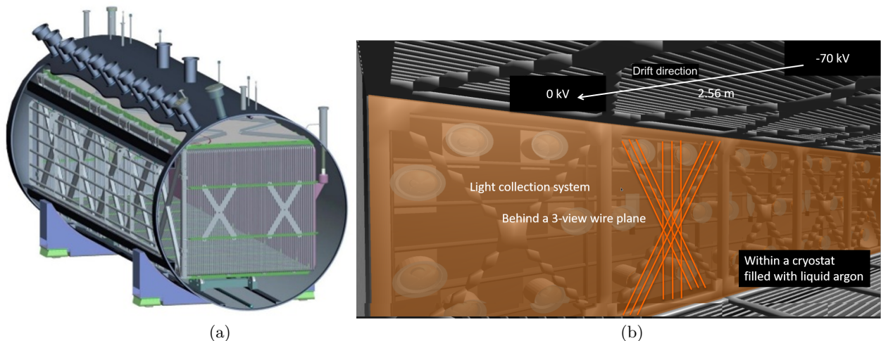
FIG. 3: Taken from Ref. [57]. (a) The MicroBooNE detector cryostat with the field cage shown inside. (b) Inside the cryostat of the MicroBooNE detector, visualized with the VENU software [61]. The maximum drift distance is 2.56 m with a drift electric field of 273 V/cm. The light-collection system, which consists of 32 PMTs, is located behind the three anode wire planes, which detect ionization charge.
