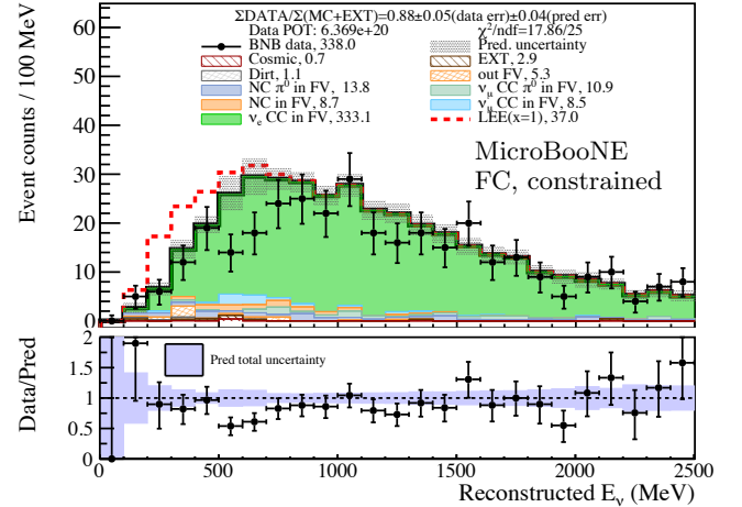
FIG. 25: Event distribution of FC \nu_e CC candidates as a function reconstructed E_\nu . Same set-up as that of Fig. 24 except that the constraint from PC \nu_e CC, FC \nu_\mu CC, PC \nu_\mu CC, FC CC \pi^0 , PC CC \pi^0 , and NC \pi^0 is used.
