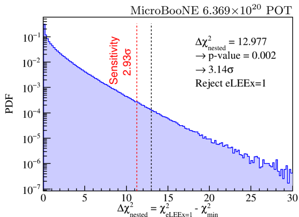
FIG. 29: Distribution of \Delta\chi^2_{\text{nested}} assuming \text{eLEE}_{x=1} is true. The sensitivity of rejecting the \text{eLEE}_{x=1} hypothesis is at 2.93\sigma following the Feldman-Cousins procedure. Using the same procedure, the data measurement rejects \text{eLEE}_{x=1} hypothesis at the p-value of 0.002, which corresponds to 3.14\sigma . The results are obtained from 10 million pseudo experiments.
