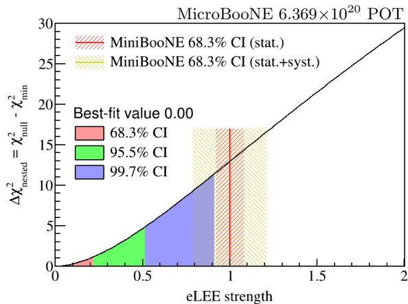
FIG. 28: The \Delta\chi^2_{\text{nested}} with the nested likelihood ratio test. The best-fit eLEE strength is at x_{\text{min}} = 0 . The Feldman-Cousins 68.3%, 95.5% and 99.7% confidence intervals (CI) are displayed with the red, green and blue bands, respectively. The 68.3% confidence interval of the eLEE strength extracted from the MiniBooNE 2020 result are also shown for comparison purpose.
