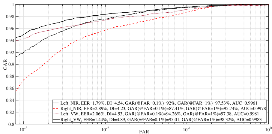
Fig. 4 ROC curves for DF
