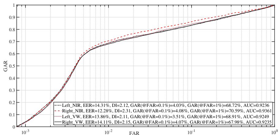
Fig. 3 ROC curves for HCF
