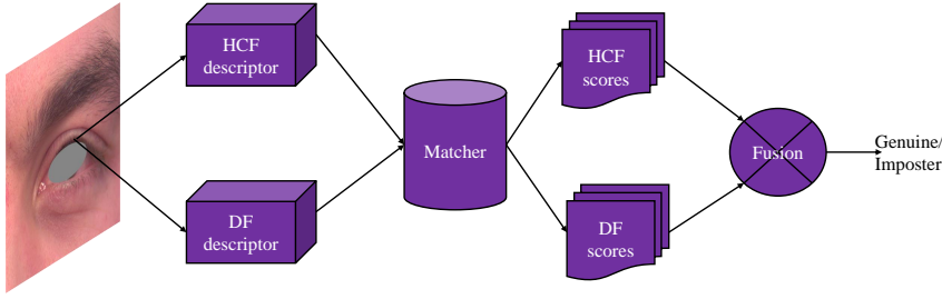
Fig. 1 Overall block diagram of the proposed approach
