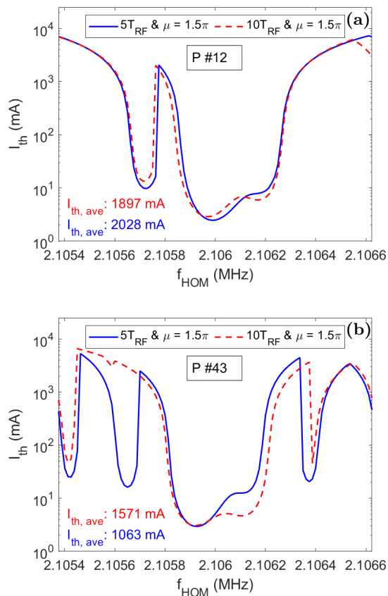
FIG. 9: Threshold currents as function of HOM frequency pattern number 12 and 43 at two bunch spacings. In (a) they are similar and in (b) different threshold currents.
