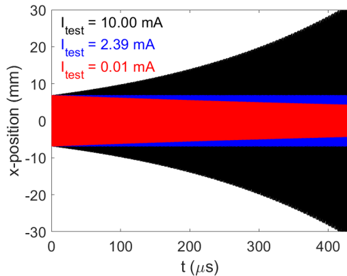
FIG. 5: Particle x-position (in the cavity) when test currents I_{test} is above (black), below (red), and at (blue) the threshold current.
