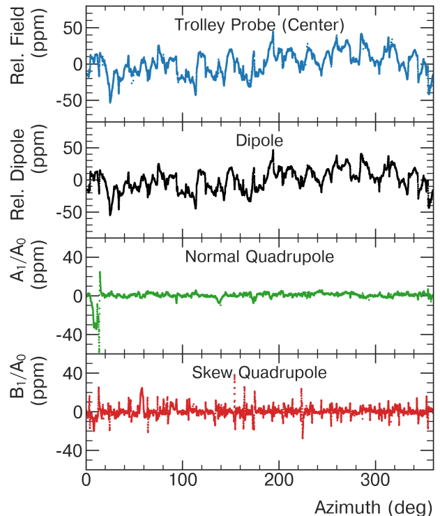
FIG. 12: A typical field map from a trolley run (25th of April 2018, approximately at 3 a.m.). On top, the raw, relative frequency (\omega_j(\phi, 0) - \langle \omega_j \rangle) / \langle \omega_j \rangle for the central trolley probe, j = 1 . The lower three plots show the corresponding lowest-order multipoles, dipole (black), normal quadrupole (green), and skew quadrupole (red), as a function of azimuth. The dipole distribution has an RMS of 16 ppm with a peak-to-peak variation of 101 ppm.
