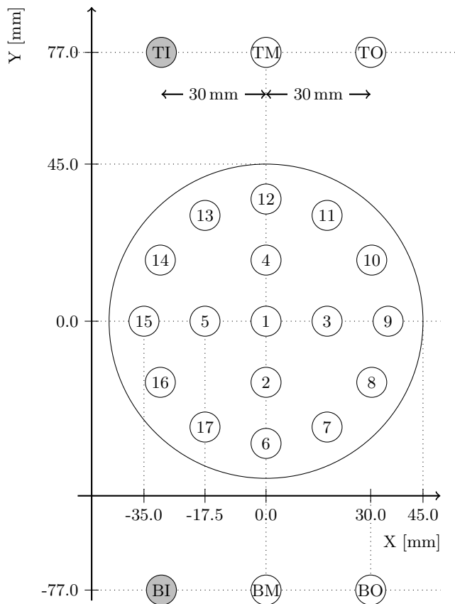
FIG. 6: The layout of the 17 probes in the trolley. Positive x is towards higher radius. The fixed probe locations on the top (T) and bottom (B) of the storage region are shown as well. For the fixed probes, the six-probe stations have probes in the inner (I), middle (M), and outer (O) positions. In the four-probe stations, only the middle and outer probes are present.
