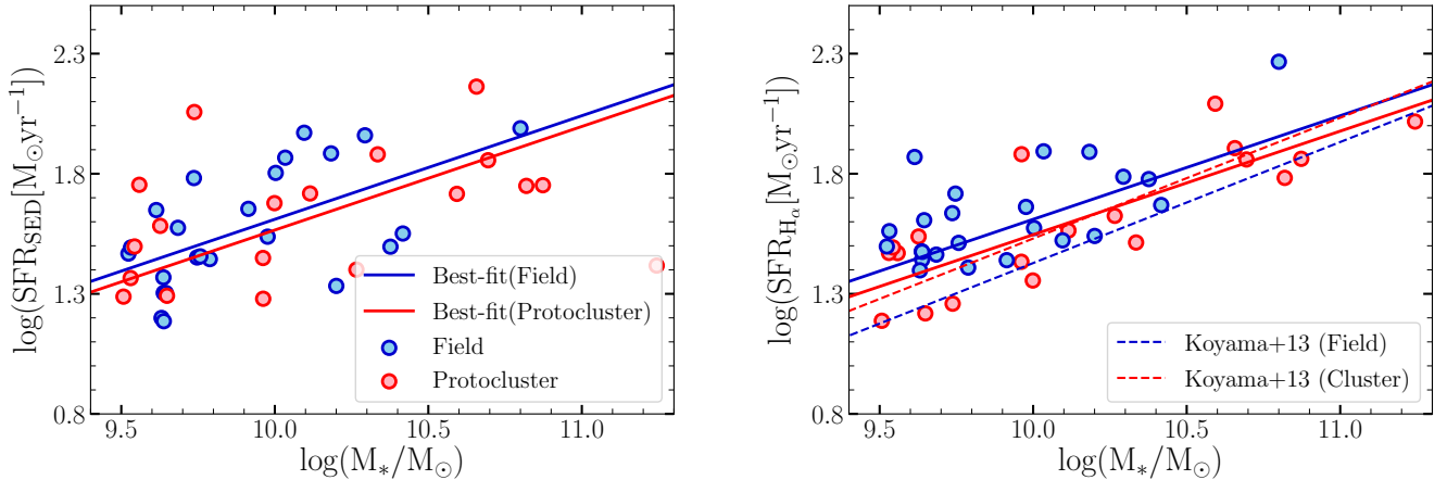
Figure 2. SFR of the field (blue circles) and protocluster (red circles) galaxies as a function of their stellar masses. Left: The SFRs are calculated from SED fitting. Right: The SFRs are determined using the H\alpha luminosity of galaxies corrected for the dust extinction based on their stellar masses. The solid lines in each panel show the best-fit to the data points. The slope of the protocluster best-fit line (solid red lines) is fixed at the slope of the best-fit line for field galaxies (solid blue lines). The dashed blue (red) line shows the best-fit for the field (cluster) galaxies from Koyama et al. (2013).
