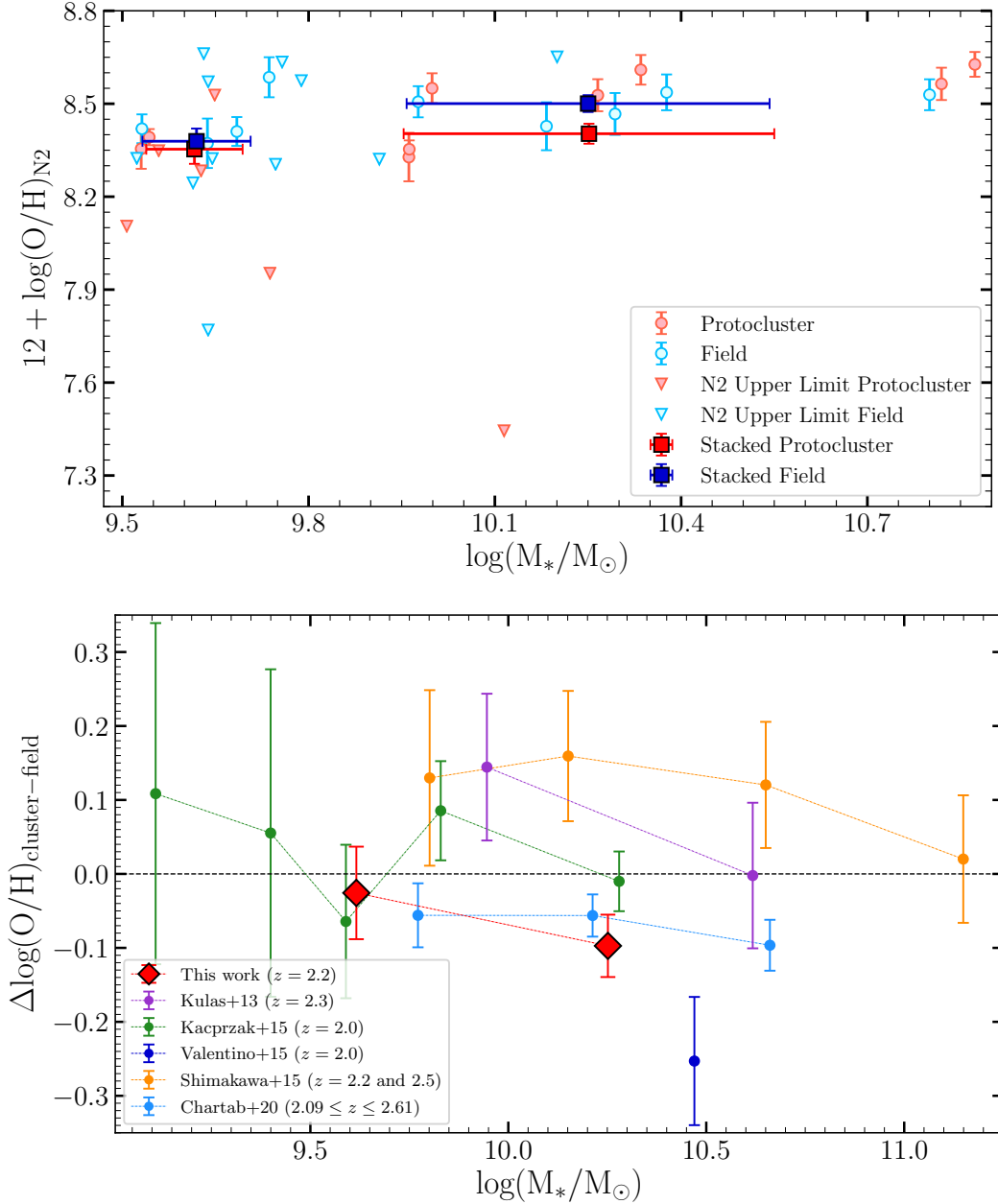
Figure 5. Top: The MZR for the mass-matched samples at z \sim 2.2 for protocluster galaxies (red) and field galaxies (blue). Inverted triangles show [\text{NII}]\lambda 6584 non-detections. The gas-phase metallicities for stacked spectra of protocluster and field samples in two stellar mass bins of 10^{9.5}M_\odot \leq M_* < 10^{9.9}M_\odot , and 10^{9.9}M_\odot \leq M_* \leq 10^{10.9}M_\odot are also shown in red and blue squares, respectively. The horizontal error bars in the stacked data show 1\sigma scatter in stellar mass of each bin. Bottom: The compilation of the difference (offset) between gas-phase metallicity of protocluster and field galaxies as a function of stellar mass from literature. The red data points show the offset for the mass-matched samples used in this work in two stellar mass bins. The uncertainties in the offsets include errors from gas-phase metallicities of both protocluster and field samples.
