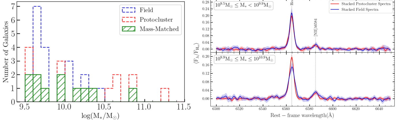
Figure 4. Left: The stellar mass distributions for the field (blue) and protocluster (red) galaxies. The green hatched region shows the matched stellar mass distributions of protocluster and field galaxies. Right: Composite spectra for the mass-matched samples in two bins of stellar mass ( 10^{9.5}M_{\odot} \leq M_{*} < 10^{9.9}M_{\odot} , and 10^{9.9}M_{\odot} \leq M_{*} \leq 10^{10.9}M_{\odot} ). The stacked spectra of protocluster galaxies are shown in red and the stacked spectra of field galaxies are shown in blue.
