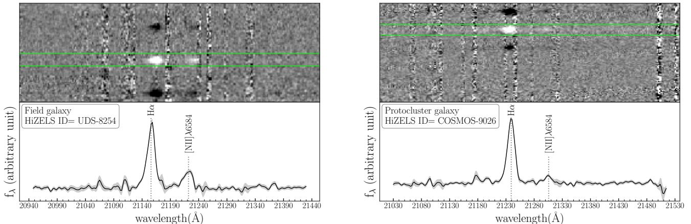
Figure 1. The 2D and corresponding optimally extracted 1D spectra for two galaxies selected from our sample. Left: Example of a field galaxy. This galaxy is at z = 2.223 and has a stellar mass 10^{10.05} M_{\odot} . Right: A galaxy member of the protocluster at z = 2.235 . The stellar mass of this galaxy is 10^{9.96} M_{\odot} . In both spectra, H\alpha and [\text{NII}]\lambda 6584 emission lines are evident.
