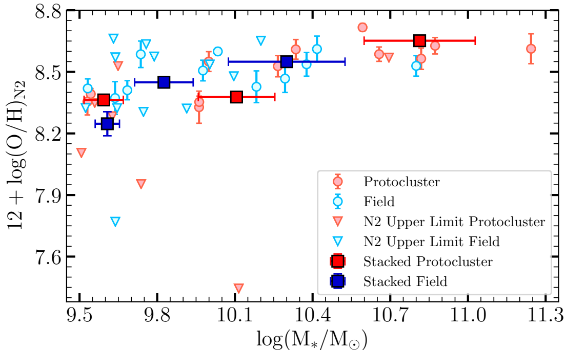
Figure 3. MZR for the field (blue circles) and protocluster (red circles) galaxies at z \sim 2.2 , without controlling for the stellar mass distribution (mass-matching). The 1\sigma upper-limits for galaxies with undetected [\text{NII}]\lambda 6584 line are shown with inverted triangles. The solid blue (red) squares indicate the metallicity measurements for stacked spectra of field (protocluster) galaxies in three bins of stellar mass. The error bars are smaller than the square symbols if not shown. Also, the horizontal error bars in the stacked data show the 1\sigma scatter in the stellar mass of each bin.
