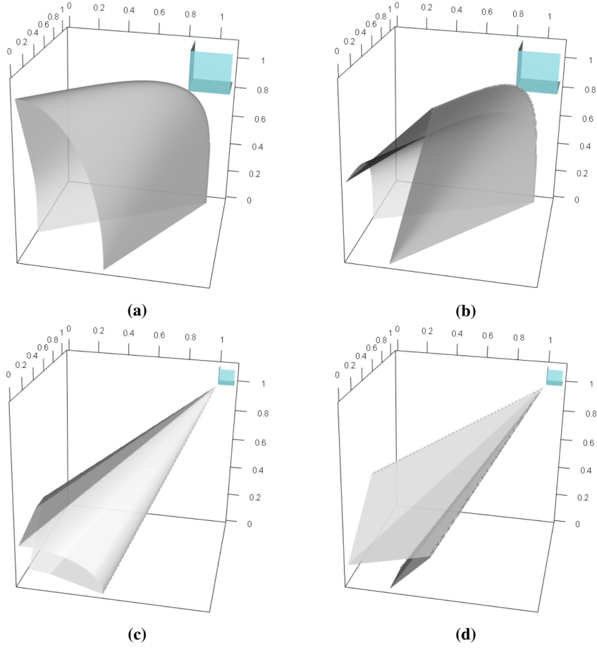
Fig. 11: The sets G = \{x \in \mathbb{R}^3 : g(x) = 1\} for the remaining four trivariate vine copula cases (grey) with the boundary of the set [\eta_{(1,2,3)}, 1, 1]^3 (blue): \alpha = 0.5, \beta = 0.25, \gamma = 0.5 .
