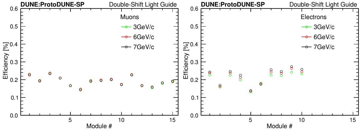
Figure 42: Efficiency measurements of 15 double-shift light-guide modules (PDS beam side), as determined from beam muons (left) and beam electrons (right) data at different momenta (only modules j = 1, \dots, 10 in APA3, and 2 at the shorter distance from the shower and higher photon counting are displayed).
