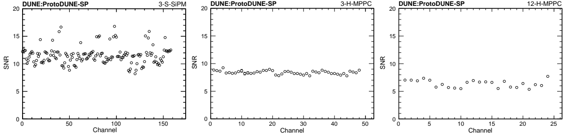
Figure 35: Signal-to-Noise Ratio (SNR) for the 3-S-SiPM channels (left), for the 3-H-MPPC channels (center), and for the 12-H-MPPC channels (right).
