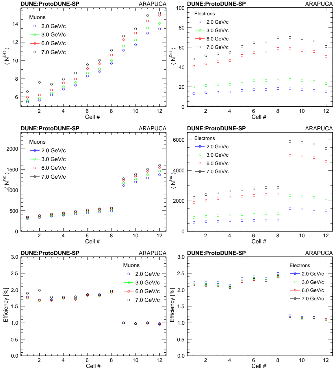
Figure 41: ARAPUCA cell efficiency as determined from beam muons (left) and beam electrons (right). Cells are of two types with the last four cells (channels j = 9, \dots, 12 ) have double size but equal number of photosensors than the first eight. Top: average number of detected photons with beams at different momenta. Center: average number of photons incident on the cell surface from MC simulation of electron and muon beams at corresponding momenta. Bottom: efficiency of the cell from the detected-to-incident ratio. Statistical error bars are small, not visible inside the symbols.
