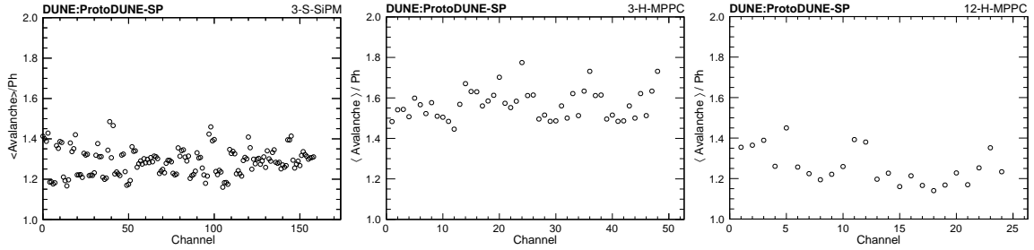
Figure 37: Afterpulse and crosstalk contribution to the photosensor signal expressed by the average number of avalanches generated per detected photon for the 3-S-SiPM channels (left), for the 3-H-MPPC channels (center), and for the 12-H-MPPC channels (right).
