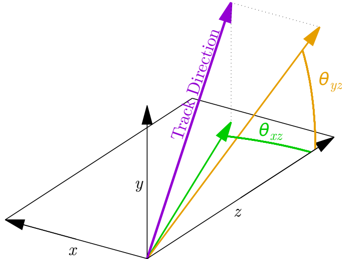
Figure 27: The definitions of the track direction angles \theta_{xz} and \theta_{yz} .
