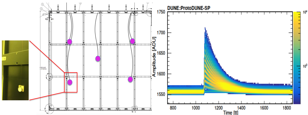
Figure 31: The ProtoDUNE-SP photon-detector calibration and monitoring system installation on the CPA panels (left). The inset shows the actual lower left diffuser at time of installation. Waveforms in a LED calibration run displayed in persistence trace mode (right) showing recorded single and multi-photon signals. Each time tick (tt) represents 6.67 ns.
