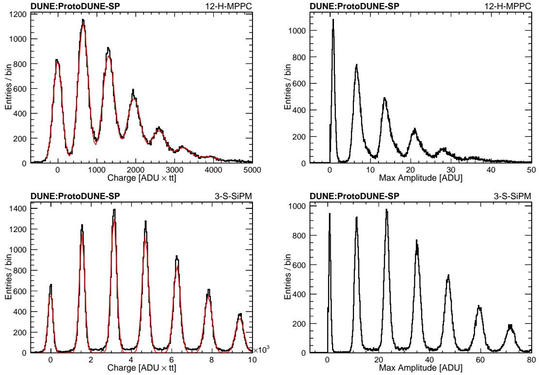
Figure 33: Charge (left) and current (right) distribution for typical 12-H-MPPC channel ( V_{\text{B}} = 48 \text{ V} ) (top) and 3-S-SiPM channel ( V_{\text{B}} = 26 \text{ V} ) (bottom) under low amplitude pulsed LED illumination. A fit of the charge distributions with a multi-Gaussian function giving peak positions and widths is shown in red.
