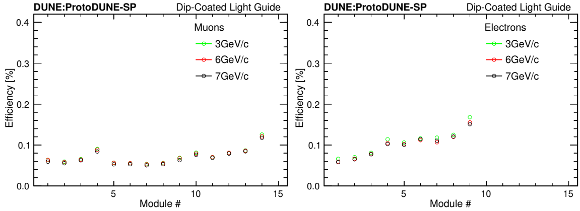
Figure 43: Efficiency measurements of 14 dip-coated light-guide modules (PDS beam side), as determined from beam muons (left) and beam electrons (right) data at different momenta (only modules j = 1, \dots, 9 in APA3, and 2 at the shorter distance from the shower and higher photon counting are displayed).
