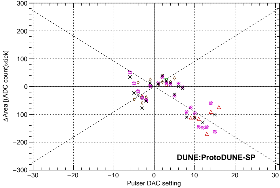
Figure 17: Measurement residuals (data - fit) for the same data as the preceding figure (black) plus the same for data taken in the following months (colors). The dashed lines indicate deviations of \pm 1\% .
