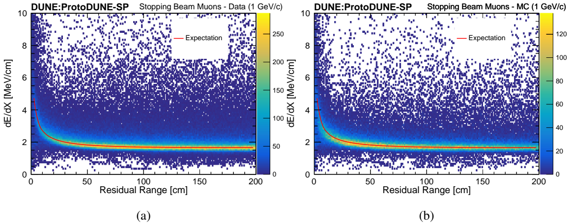
Figure 63: dE/dx vs residual range for selected stopping muons in the 1 GeV/ c beam after applying the calibration derived using cosmic-ray muons, in data (a) and MC (b). The expected most probable value of dE/dx is plotted as a function of residual range for both.
