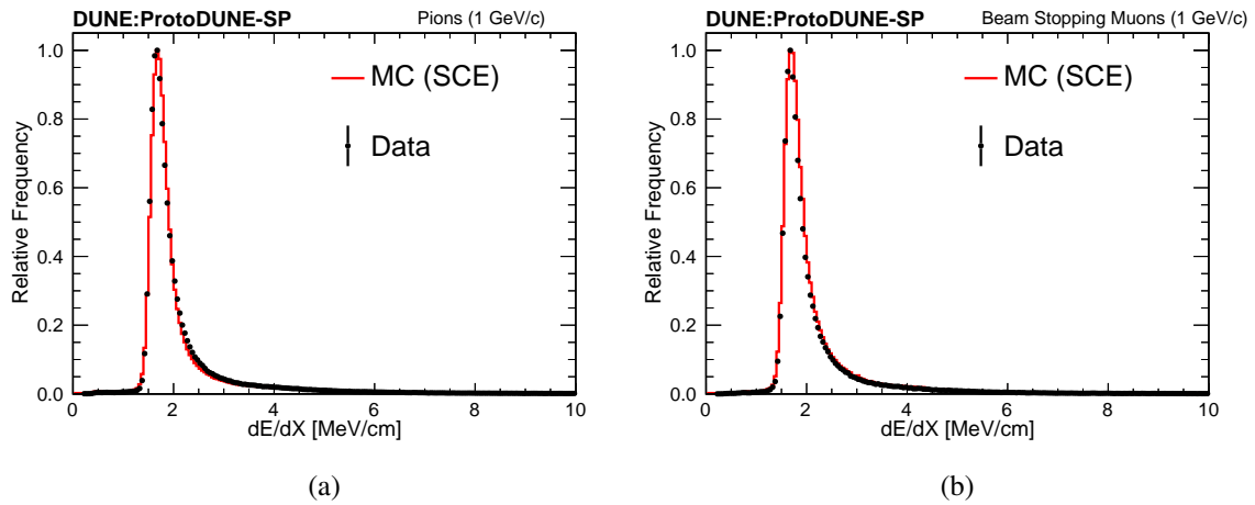
Figure 62: Pion (a) and stopping muon (b) dE/dx distributions for the ProtoDUNE-SP beam data after applying the calibration derived using cosmic-ray muons. The distribution for replica selections on a beam Monte Carlo sample with space charge effect simulated is also shown. The histograms are normalized such that the maximum frequency is one.
