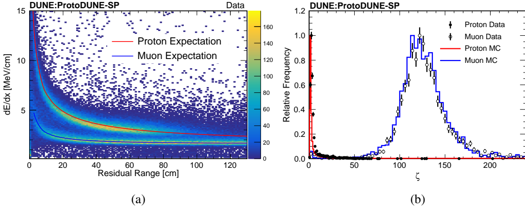
Figure 67: (a) dE/dx versus residual range after the SCE corrections for the stopping protons (upper band) and the muons (lower band). The solid lines represent the expected most probable values for the protons (red) and the muons (blue). (b) The \zeta distributions of the stopping protons and muons. The histograms are normalized such that the maximum frequency is one.
