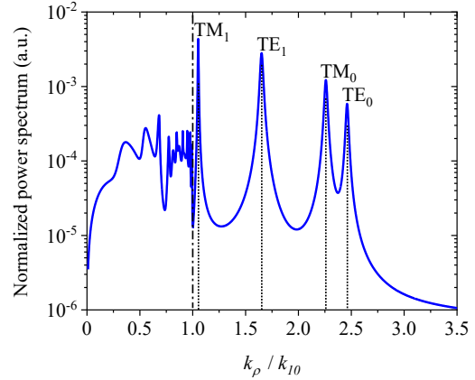
Fig. 3. Power spectrum of a HED emitting near the silicon waveguide.
