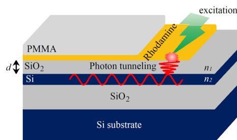
Fig. 1. Sample structure of energy transfer from submonolayer rhodamine to an ultrathin silicon waveguide.
