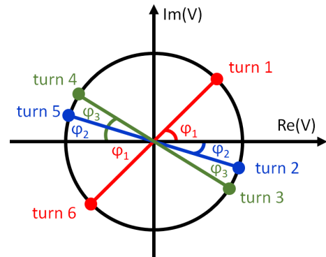
FIG. 16: Definition of off-set angles in off-crest beamloading.
