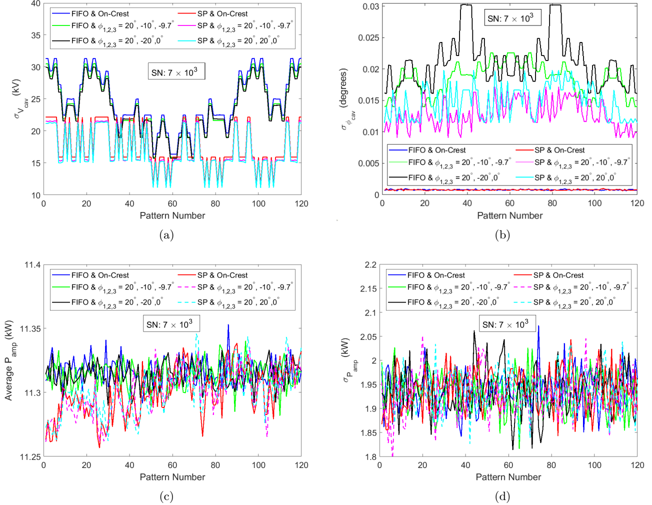
FIG. 23: Comparison of SP and FIFO at dynamic set-points when beam loading is at on-crest: (a) cavity voltage jitters; (b) cavity phase jitters; (c) average amplifier power; and (d) amplifier power jitters.
