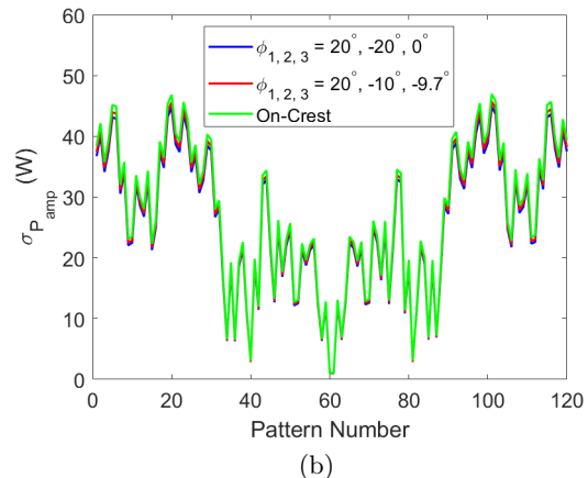
FIG. 18: Cavity voltage fluctuation (a) and amplifier power amplitude fluctuation (b) of off-crest beam loading for 120 patterns for 6-turn ERL. The S/N is 10^{12} .
