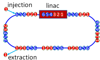
FIG. 3: Filling of ERL by multiple bunch packets.
