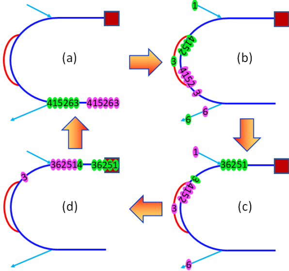
FIG. 21: Topology with an extra arc 6 length to preserve \{4\ 1\ 5\ 2\ 6\ 3\} bunch-turn number sequence. (a) Depiction of two bunch packets before entering the arcs. (b) Green bunch at 3 rd turn gets delayed. Bunches at their 6 th turn are extracted. (c) Green bunch at 3 rd turn is delayed and joined pink packet. When the packet passes injection point, all the bunch numbers are incremented by 1. (d) A new bunch is injected into pink packet. New circulation starts with (a) again.
