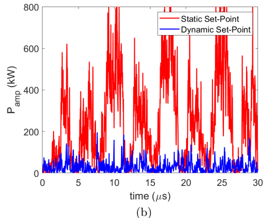
FIG. 10: Comparison of static and dynamic set-points for filling pattern [1 2 3 4 5 6] when S/N = 7.1 \times 10^2 . (a) cavity voltage and (b) amplifier power as function of time.
