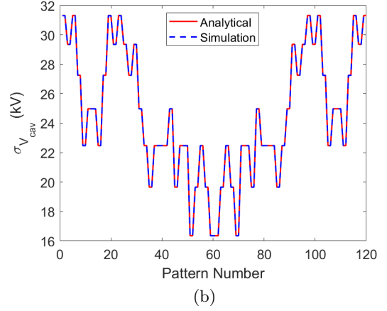
FIG. 13: Simulated \sigma_{V_{cav}} of 120 patterns with (a) static and (b) dynamic set-points compared to prediction. The S/N was set to 1 \times 10^{12} to turn off the noise.
