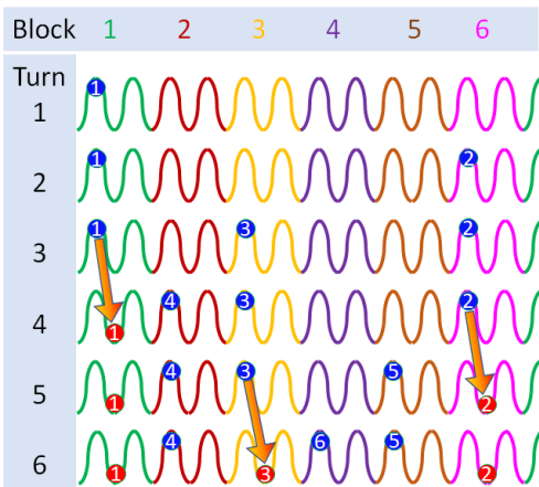
FIG. 4: Filling of recirculating linac with filling pattern [1 4 3 6 5 2].
