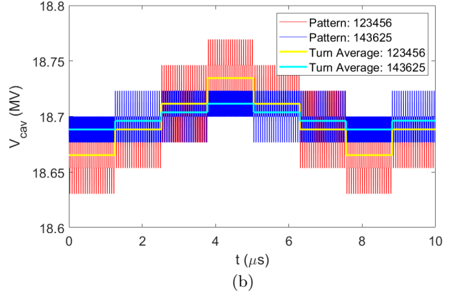
FIG. 15: Comparison of V_{cav} and turn average of V_{cav} of different patterns. (a) ASPO and non-optimal pattern. (b) DSPO and non-optimal pattern.
