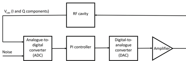
FIG. 8: A block diagram of the modelled LLRF system and the feedback loop.
