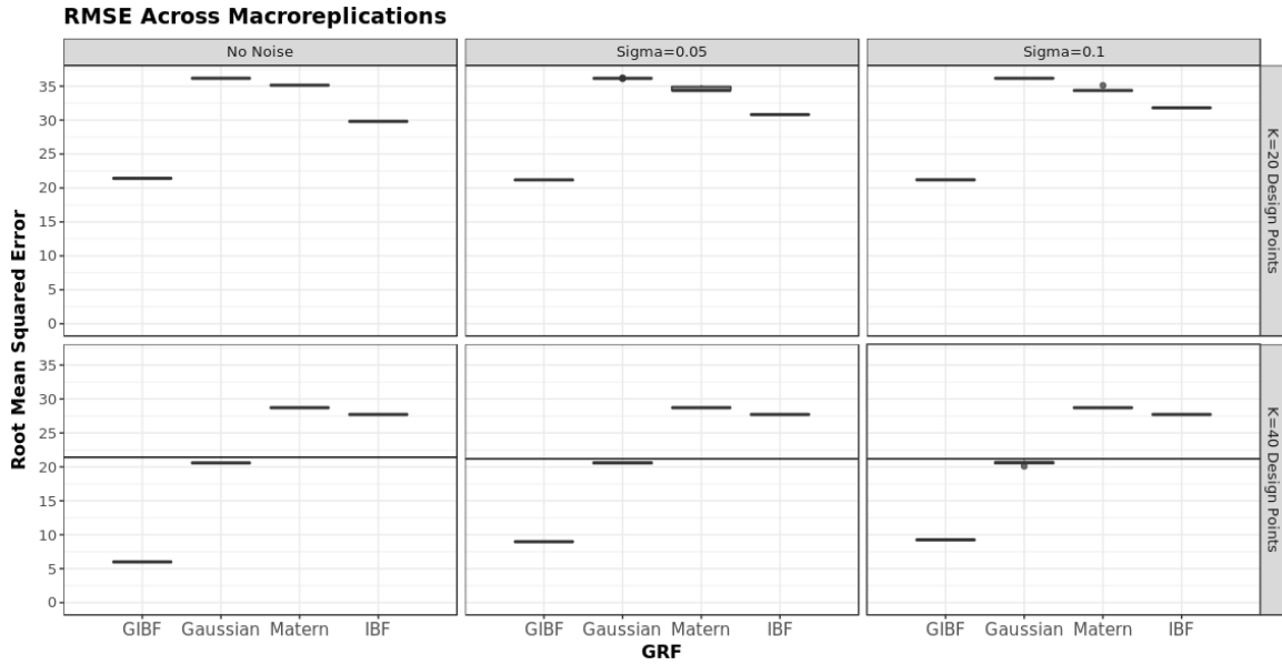
Figure 5 Box-plots of RMSE for the expected profit simulation.
