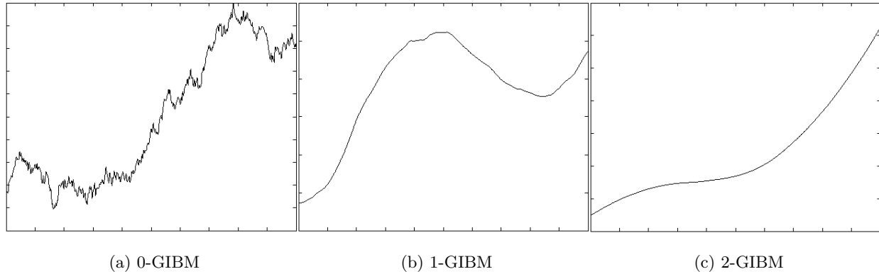
Figure 1 Sample paths of GIBMs on the unit interval.
