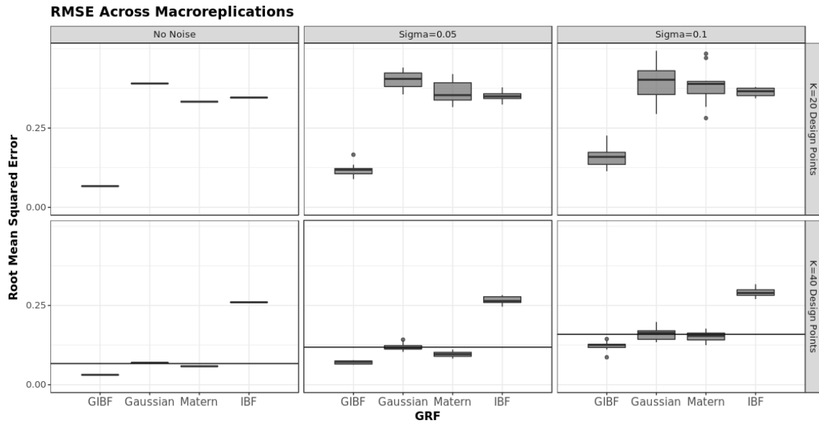
Figure 6 Box-plots of RMSE for the Alpine-1 test function.
