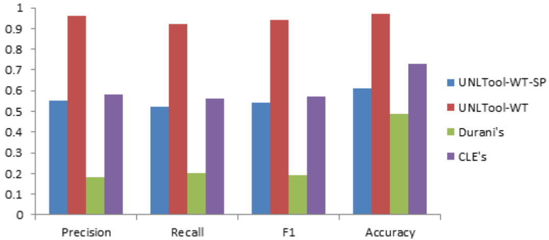
Fig. 3.1 Performance comparison of various Urdu word tokenizers on UNLTool-WT-Test dataset
