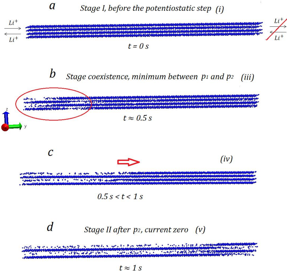
Figure 9: Snapshots taken from kMC simulations for a potentiostatic steps from 50 mV to 95 mV. Li-ions are represented in blue; graphite was omitted with visualization purposes. The graphite / electrolyte interphase (Li-ion exchange) is highlighted on the left of Figure a with arrows, illustrating lithium intercalation / deintercalation. On the right of the figure, lithium ions are confined by a wall and cannot be exchanged with the reservoir of particles. This effect is represented with crossed arrows.
