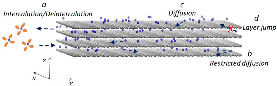
Figure 1: Events and restrictions imposed to the system. Li-ions are represented in blue, graphite in grey, solvated Li-ion are represented with blue spheres surrounded by orange balloons.
