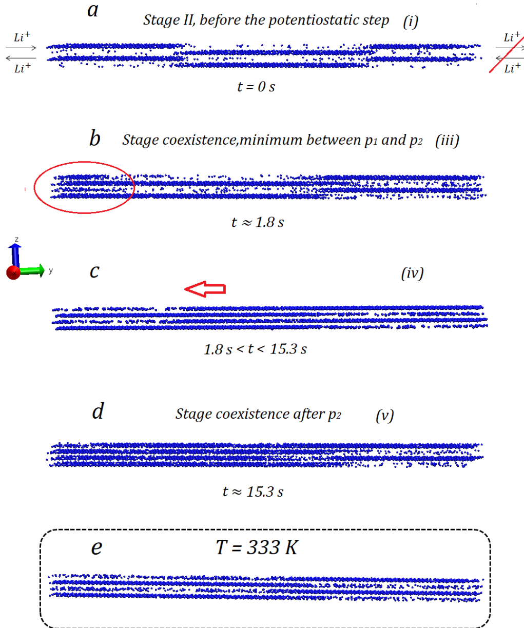
Figure 11: Snapshots for kMC simulations for the potentiostatic step from 95 mV to 78 mV. Li-ion are represented in blue; graphite was omitted with visualization purposes. The graphite / electrolyte interphase (Li-ion exchange) is highlighted in Figure a at the left of the figure with arrows for lithium intercalation / deintercalation. At the right of the figure lithium ions cannot be exchanged with the reservoir of particles, this is represented with crossed arrows. Figures a to d corresponds to T=313 \text{ K} . Figure e , enclosed in a dashed line rectangle, is the frame corresponding to the final state of the simulation at T=333\text{K} .
