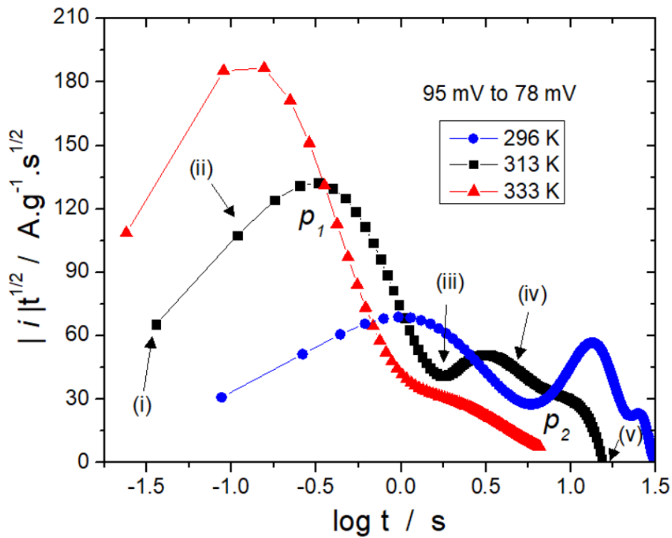
Figure 10: kMC results for the Cottrell representation for a potentiostatic step 95\text{ mV} \rightarrow 78\text{ mV} . The main features are pointed with arrows from (i) to (v) for T = 313\text{ K} . The peaks p_1 and p_2 are indicated for T = 313\text{ K} . The different features may be correlated with simulation snapshots presented in Figure 11.
