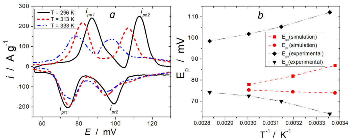
Figure 3: Effect of temperature on simulated voltammetric profiles. a ) Voltammograms at \nu = 5.00 \text{ mV}\cdot\text{s}^{-1} and for different temperatures. b ) E_{p1} vs T^{-1} for voltammetric data from the simulations shown in Figure 3 a (red dashed lines, the symbols are different for oxidation and reduction). E_{p1} vs T^{-1} from experimental data, taken from Fig 1 from ref. [2] (black solid lines, the symbols are different for oxidation and reduction). On Figure b the error bars for the simulated data are smaller than symbol size.
