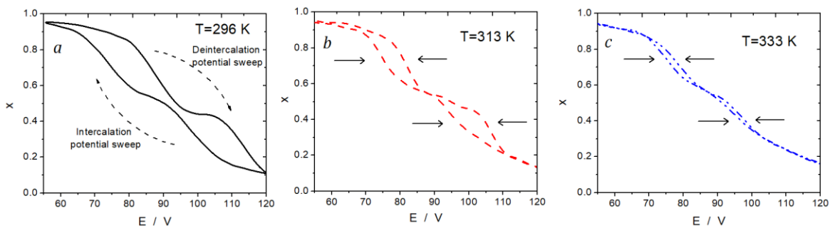
Figure 4: Isotherms at different temperatures, 296 K ( a ), 313 K ( b ) and 333 K ( c ), indicated in each figure, at \nu = 5.00 \text{ mV}\cdot\text{s}^{-1} . These plots were constructed from the voltammograms in Figure 3. For simplicity, the colors and line types are the same as those used in Fig 3. Black arrows indicate the direction of hysteresis reduction as temperature increases.
