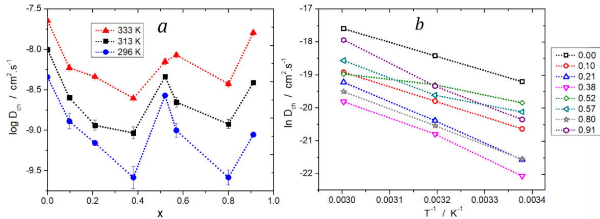
Figure 14: a ) Chemical diffusion coefficients for different temperatures, calculated with equation (4). b ) Arrhenius plots for the diffusion coefficients obtained at different lithium composition, dotted lines are drawn to guide the eye.
