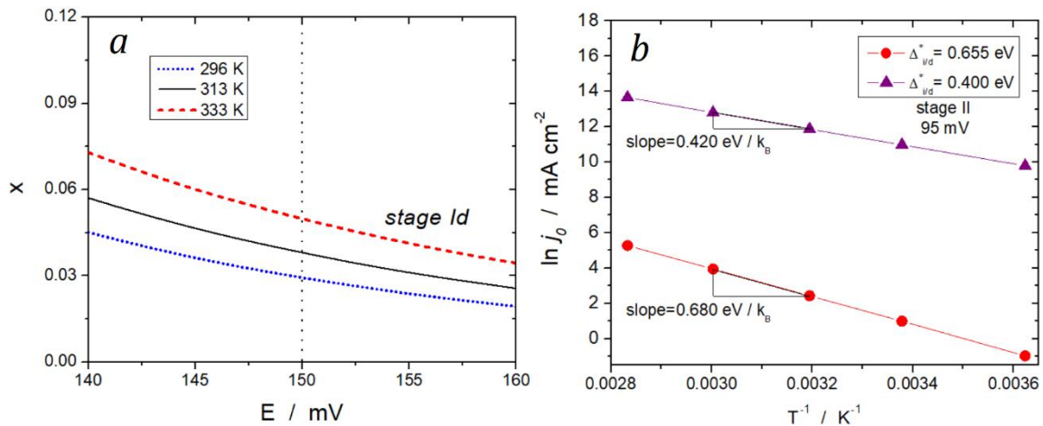
Figure 13: a ) Occupation by lithium ions as a function of potential in a small potential window from Figure 6. The change of the occupation of stage Id with temperature can be appreciated. The potential used for the analysis of the activation energy of Stage Id is indicated with a vertical dotted line. b ) Arrhenius plot for different activation barriers for the insertion/deinsertion process, \Delta^*_{i/d} . The lattice occupation corresponds to stage II and
