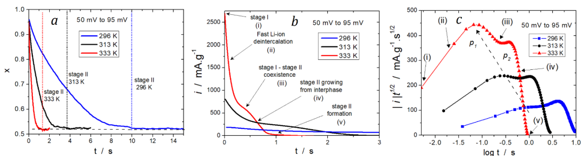
Figure 8: kMC simulations of a potentiostatic step from 50 mV to 95 mV for three different temperatures. a ) lithium composition vs t . b ) chronoamperometric response. c ) |i|t^{1/2} vs \log t plots. Features for the different processes are marked with arrows from (i) to (v) in Figs b and Figure c . The denominations of the peaks are only marked for T=333 K, but the same notation is valid for all temperatures. The different (i) to (v) features may be correlated with simulation snapshots presented in Figure 9.
