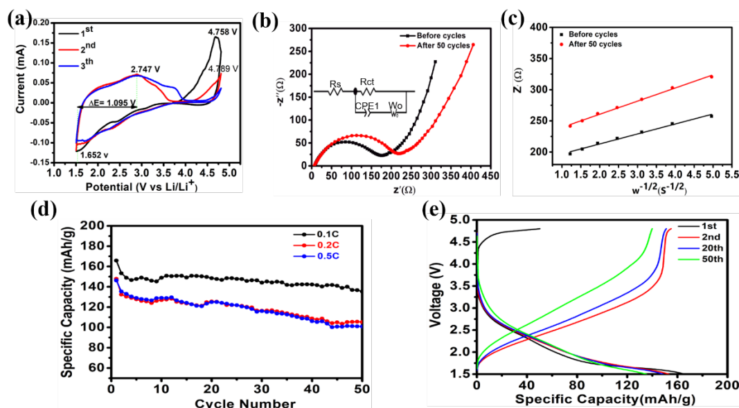
Fig. 3. (a) CV curves of the first three cycles, (b) Nyquist curves (the inset shows the equivalent circuit), (c) linear fitting curves of Z' vs \omega^{-1/2} and (d) cycling performance of \alpha -LiFeO 2 nanorods at 0.1, 0.2 and 0.5 C; (e) specific charge-discharge curves at 0.1 C of \alpha -LiFeO 2 nanorods
