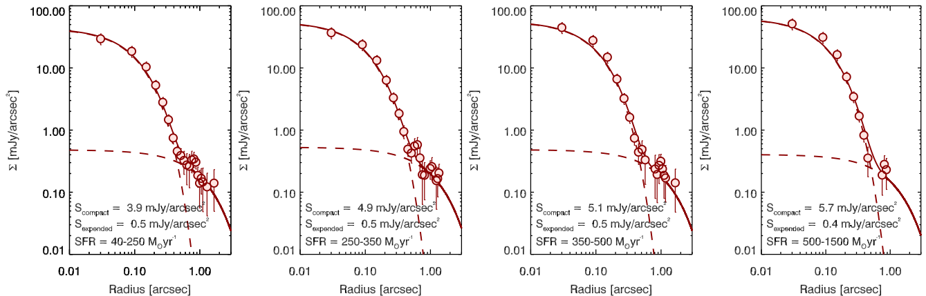
Figure 9. Surface brightness as a function of radius for the image stacks split into bins of star-formation rates of 40–250, 250–350, 350–500 and 500–1500 M_{\odot}\ \text{yr}^{-1} . Both stacks in the image plane and visibility plane return similar profiles, which are composed of a compact and an extended component (we therefore only show the image stack). We fit double exponential profiles and find that the peak flux of the extended component is close to constant at a mean of 0.47 \pm 0.03\ \text{mJy} for the four stacks, while the compact component becomes brighter with increasing star-formation rate.
