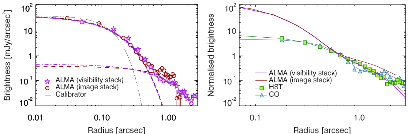
Figure 7. Left: The 870\ \mu\text{m} continuum light profile obtained by stacking the 870\ \mu\text{m} dust maps in the visibility and image plane. The profile shows that most of the emission is compact, but that 13 \pm 1\% of the emission is extended on larger scales ( \geq 0''.5 or \geq 10\ \text{kpc} ), and only detected in our maps by stacking. The RMS level of the image stack is illustrated by the dotted line. Right: The 870\ \mu\text{m} continuum light profile obtained by stacking the 870\ \mu\text{m} dust maps in the visibility and image planes, normalised and compared to the stacked stellar and molecular gas profile seen in HST and ALMA imaging (Calistro Rivera et al. 2018). While the 870\ \mu\text{m} dust continuum emission has an excess in the nuclear region compared to the stellar and molecular gas profiles, the extended component follows that of the stellar and molecular gas, suggesting that they trace the same structural component in these systems.
